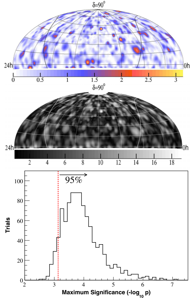
FIG. 10 (color online). Sky map of significances ( -\log_{10}p ) obtained in the full-sky search excluding trial factors (top panel), sky map of \nu_\mu + \nu_\tau 90% confidence level flux upper limits for an E^{-2} energy spectrum ( 10^{-11} TeV cm ^{-2} s ^{-1} ) over the energy range 1.9 TeV to 2.5 PeV (middle panel), and the distribution of maximum significances for 1000 randomized sky maps, with the obtained significance p = 7.4 \times 10^{-4} dotted (bottom panel).
