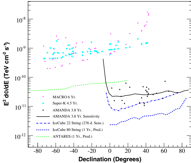
FIG. 11 (color online). Limits on an E^{-2} muon neutrino flux for sources in Table III from this work (triangles), limits from MACRO [14], and Super-K [15], E^{-2} \nu_{\mu} sensitivity for this work and the IceCube 22-string analysis, and predicted sensitivity for ANTARES [40] and IceCube. Our \nu_{\mu} + \nu_{\tau} limits are divided by 2 for comparison with limits on only \nu_{\mu} .
