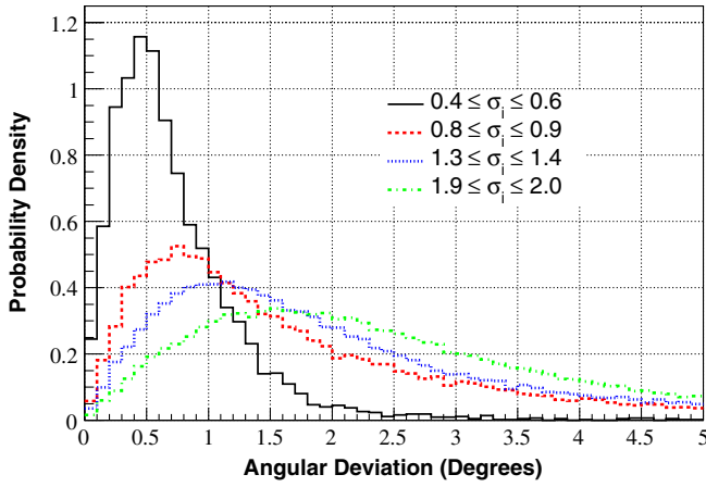
FIG. 7 (color online). Distributions of angular deviation between true and reconstructed tracks for simulated neutrino events over several ranges of estimated angular uncertainty.
