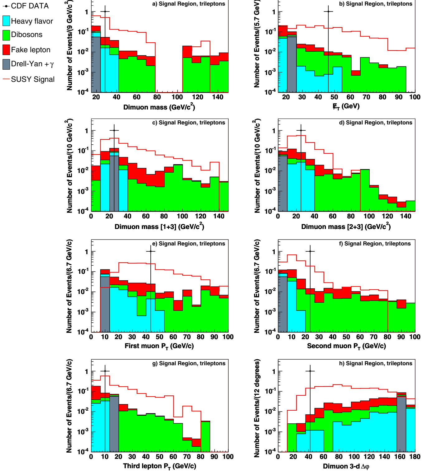
FIG. 8 (color online). Kinematic variables for the SM background and the SIG2 SUSY signal, in the trilepton signal region. The background histograms are stacked; the signal histogram is not. The CDF data are indicated by points with error bars.
