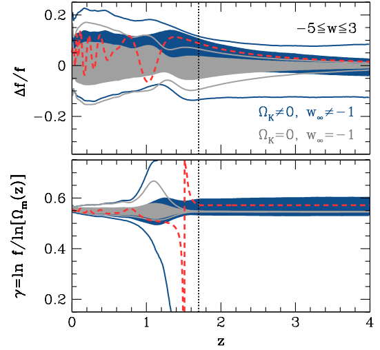
FIG. 20 (color online). Effects of curvature and early dark energy on the smooth dark energy growth rate. Same as Fig. 19 but for smooth dark energy models ( -5 \leq w \leq 3 ).
