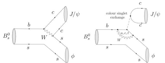
FIG. 1. Decay topologies contributing to B_s^0 \rightarrow J/\psi\phi in the SM.
