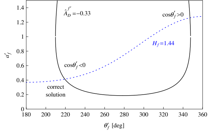
FIG. 6 (color online). Illustration of the contours in the \theta'_f - a'_f plane for an example, as discussed in the text.
