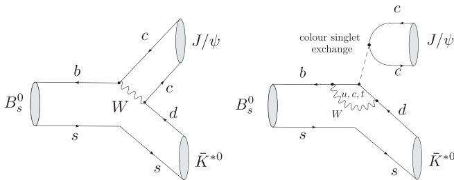
FIG. 5. Decay topologies contributing to B_s^0 \rightarrow J/\psi \bar{K}^{*0} in the SM.
