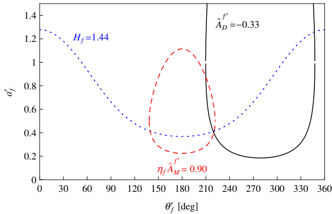
FIG. 7 (color online). Illustration of the resolution of the twofold ambiguity in Fig. 6 through the mixing-induced CP violation in B_d^0 \rightarrow J/\psi \rho^0 .
