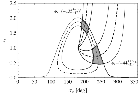
FIG. 2. The situation in the \sigma_s - \kappa_s plane of the NP parameters for B_s^0 - \bar{B}_s^0 mixing arising from current data and theory input, as discussed in the text.
