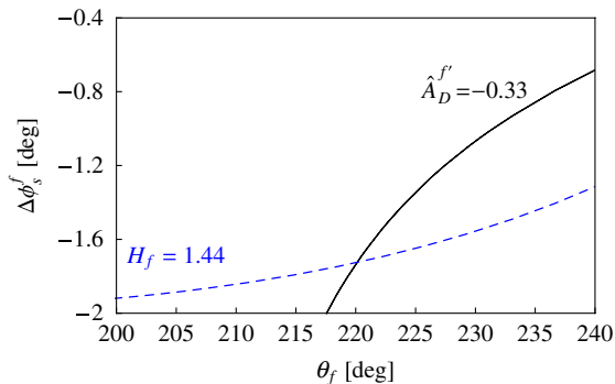
FIG. 8 (color online). Situation in the \theta_f - \Delta\phi_s^f plane for the example in Figs. 6 and 7.
