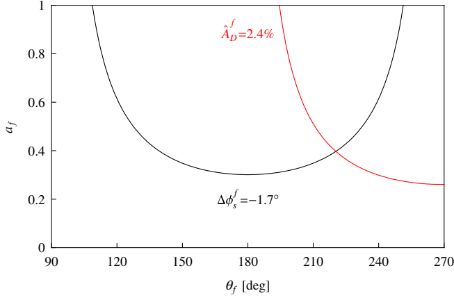
FIG. 10 (color online). The extraction of a_f and \theta_f from \Delta\phi_s^f and the direct CP asymmetry \hat{A}_D^f for internal consistency checks of the SU(3) flavor symmetry, as described in the text. The example corresponds to a_f = 0.4 and \theta_f = 220^\circ with \gamma = 65^\circ , as in the previous numerical illustrations.
