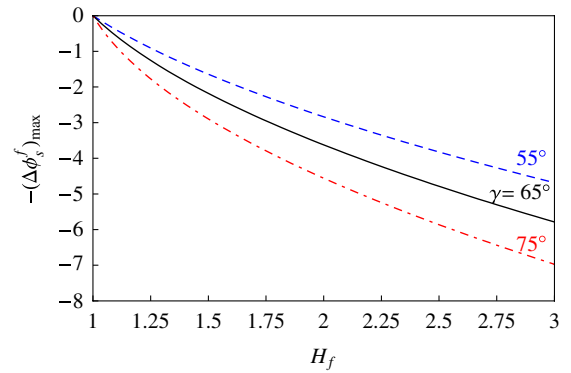
FIG. 9 (color online). The maximal shift of \phi_s as a function of H_f for various values of \gamma .
