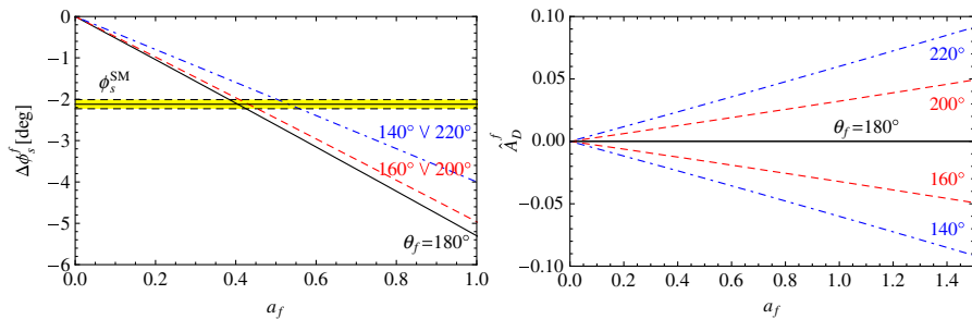
FIG. 4 (color online). Left panel: The dependence of \Delta\phi_s^f on a_f for various values of \theta_f ; right panel: the dependence of \hat{A}_D^f on a_f for various values of \theta_f .
