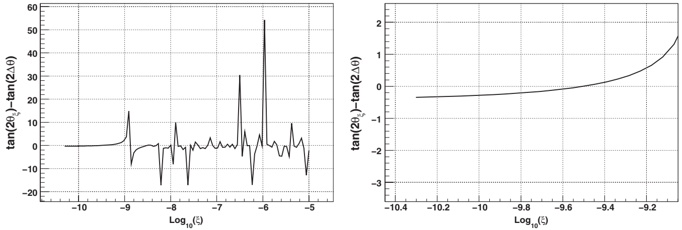
FIG. 2. Constraint for the polarization rotation case. Left panel: dependence of \tan(2\theta_f) - \tan(2\Delta\theta) on \xi . The spikes correspond to rotations by \pi/4 . Right panel: a zoom-in on the interesting range of values. The constraint is cast according to Eq. (6).
