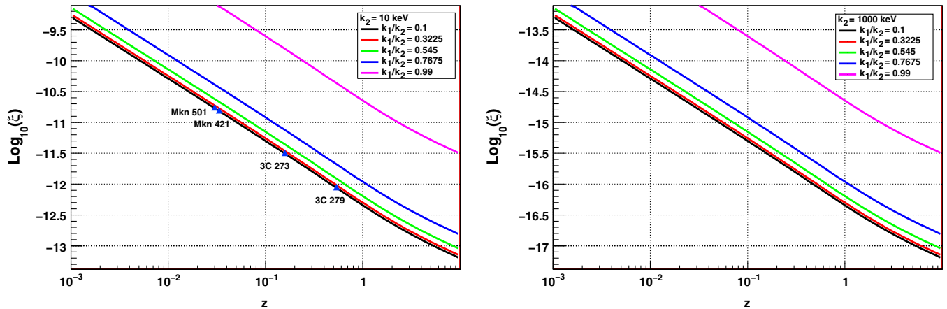
FIG. 3 (color online). Expected constraints from medium X- and soft \gamma -ray polarimetry of extragalactic sources. High-energy scale k_2 = 10 keV (left panel) and 1 MeV (right panel), with \kappa \equiv k_1/k_2 from 0.1 to 0.99. Points in the left panel refer to the characteristics of a new generation X-ray polarimeter [37] assuming that polarization is detected from the mentioned objects. The constraints are derived as in case of Eq. (4) for a concordance cosmology ( \Omega_m = 0.28 , \Omega_\Lambda = 0.72 and H_0 = 73 \text{ km s}^{-1} \text{ Mpc}^{-1} ).
