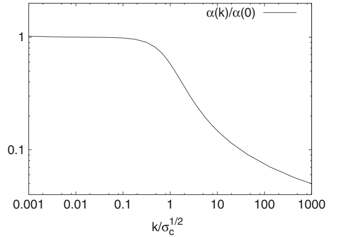
FIG. 2. Running coupling as calculated in [27].
