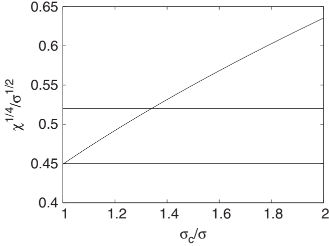
FIG. 3. Value of \chi^{1/4}/\sqrt{\sigma} depending on the ratio \sigma_c/\sigma . The two horizontal lines limit the range of the lattice results.
