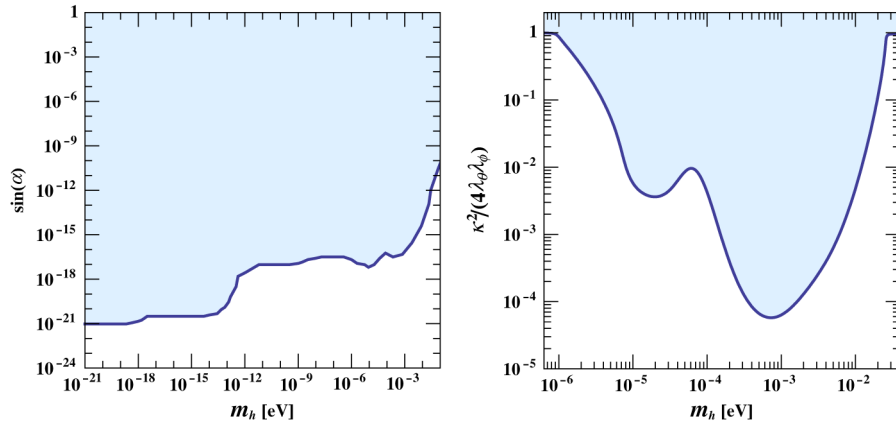
FIG. 5 (color online). Bounds on the Higgs–hidden-Higgs mixing \sin\alpha from fifth-force experiments as a function of the hidden-Higgs mass m_h (left panel). Using a Higgs mass of m_H = 120 GeV we can translate these constraints into bounds on the scaled Higgs Portal term \kappa^2/(4\lambda_\phi\lambda_\theta) as a function of the hidden-Higgs mass (right panel). For the latter we get interesting constraints in the \mu\text{eV} to 0.1 eV range. Note that the hidden-Higgs mass is related to the hidden-photon mass by Eq. (4.4) and symmetry breaking of the hidden U(1)_X requires \kappa^2/(4\lambda_\phi\lambda_\theta) < 1 .
