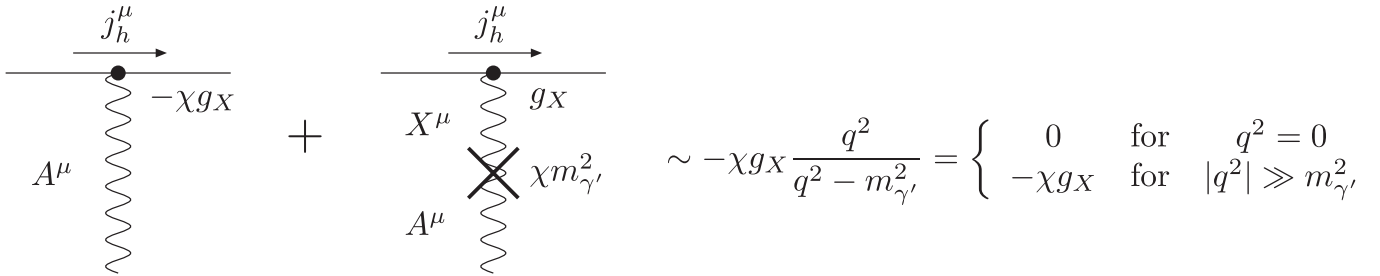
FIG. 2. Contributions to the coupling of the photon to the current generated by a hidden sector particle h in a situation where the hidden-photon is massive. The first is the direct contribution via the charge Q_{\text{EM,mixing}}e that arises from the shift (2.2) of the hidden-photon field. The second is due to the A^\mu - X^\mu oscillations caused by the nondiagonal mass term (2.7). Note that the second diagram is only present if the hidden-photon has nonvanishing mass m_{\gamma'}^2 \neq 0 .
