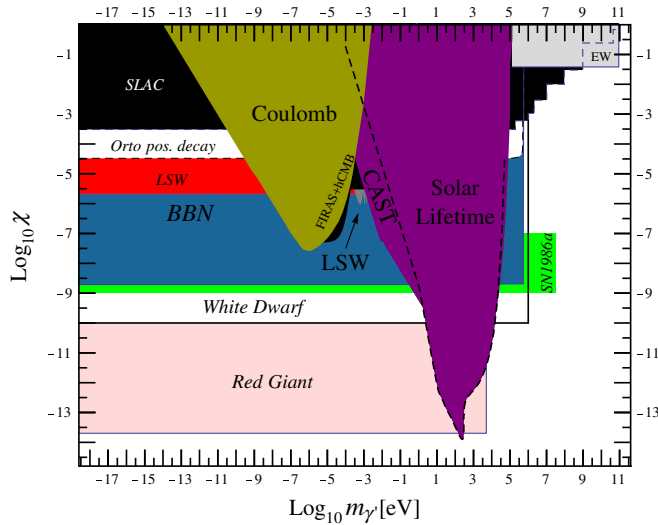
FIG. 7 (color online). Bounds on the kinetic mixing parameter for massive hidden sector photons (cf. the caption of Fig. 1). Regions labeled in italic are the bounds that apply if the mass arises from a Higgs mechanism, and the Higgs boson appears as a minicharged particle. We have bounds from a SLAC beam-dump experiment, invisible orthopositronium decays, LSW, big bang nucleosynthesis, and energy loss considerations in supernovae (SN1986a), white dwarfs and red giants (see [11,13–15]). Notice that we have assumed g_X q_X = e (so |\chi| = |q_\theta| ) and m_{\gamma'} \approx m_h . For g_X q_X \ll e , typically m_h \gg m_{\gamma'} and the new bounds move upwards and to the left.
