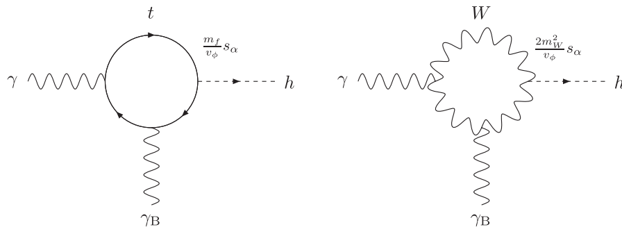
FIG. 4. Diagrams contributing to photon–hidden-Higgs oscillations in an external magnetic field.
