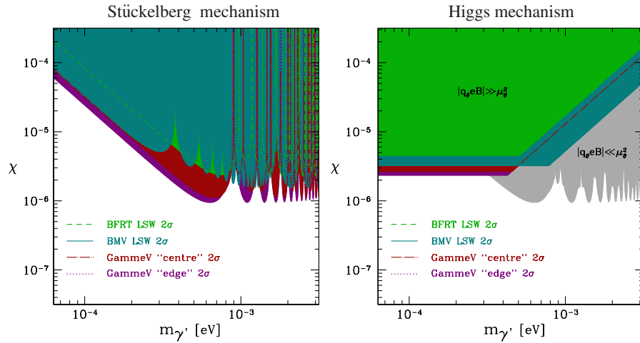
FIG. 3 (color online). Upper limits on the kinetic mixing parameter as a function of the hidden-photon mass from the nonobservation of light-shining-through-the-wall in the experiments BFRT, BMV, and GammeV. Left panel: hidden-photon mass arising via the Stückelberg mechanism. See Ref. [11] for details. Right panel: hidden-photon mass arising via the Higgs mechanism. For strong magnetic fields |q_\theta eB| \gg \mu_\theta^2 the hidden U(1) is unbroken and LSW bounds from scalar MCP loops (cf. [10]) apply. In this region, m_{\gamma'}^2 = (q_X g_X \mu_\theta)^2 / \lambda_\theta corresponds to the mass the hidden-photon would have in vacuum . Inside the magnetic field the hidden-photon mass is zero. For |q_\theta eB| \ll \mu_\theta^2 we have LSW bounds from photon-hidden-photon oscillations arising from the mass term (gray area). We use the benchmark point q_X = 1/2 , g_X = e , \kappa = 0 , and \lambda_\theta = 1 .
