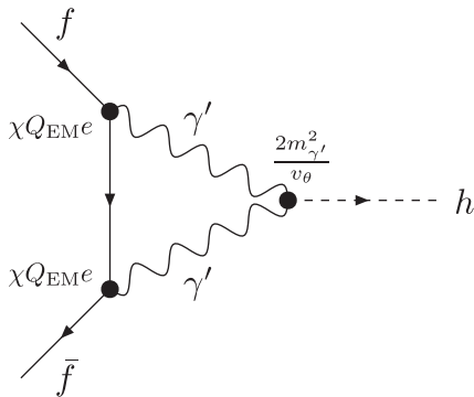
FIG. 6. Kinetic mixing contribution to the coupling of a standard model fermion f , e.g. quarks or electrons to the hidden-Higgs (the couplings for the mass eigenstates can be found in Table I). The quark coupling, in turn, contributes to the coupling to the nucleon.
