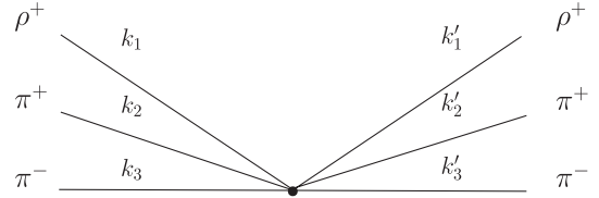
FIG. 6. Contact term whose origin is in the chiral Lagrangian.
