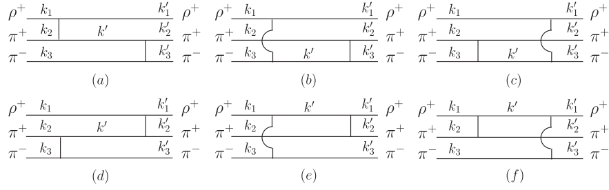
FIG. 5. Diagrams in which the off-shell part of the t matrices lead to a three-body force.
