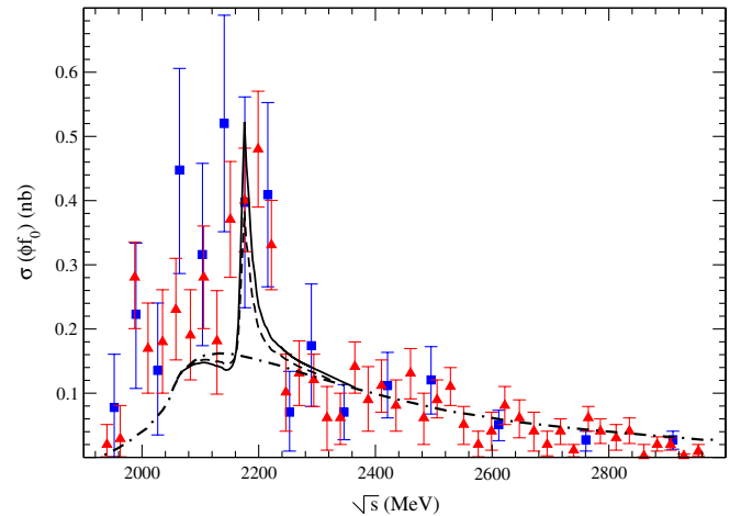
FIG. 2 (color online). The cross section for the e^+e^- \rightarrow \phi f_0 reaction. The dashed-dotted line shows the result of the calculation of the cross section in the plane wave approximation [8]. The dashed (solid) line shows the result of multiplying the amplitude from Ref. [8] by the final state interaction factor [Eq. (9)] calculated using a cutoff of 2 (2.5) GeV for the \tilde{G}_{\phi f_0}(s) . The data, which corresponds to the e^+e^- \rightarrow \phi(\pi\pi)_{I=0} reaction (triangles for charged pions and boxes for neutral pions), have been taken from [1,2].
