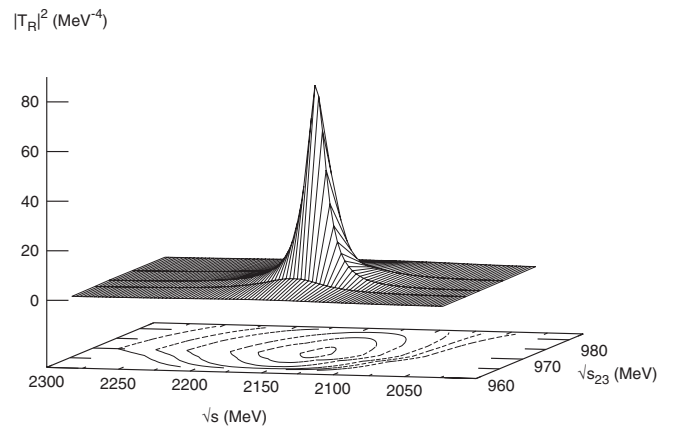
FIG. 1. The \phi K\bar{K} squared amplitude in the isospin 0 configuration.
