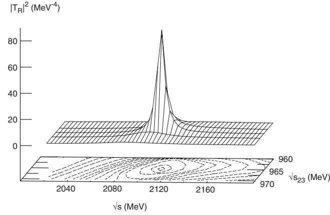
FIG. 3. The squared amplitude in the isospin 0 configuration including the \phi\pi\pi channel.
