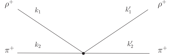
FIG. 4. Lowest order diagram contributing to the \rho^+\pi^+ interaction.
