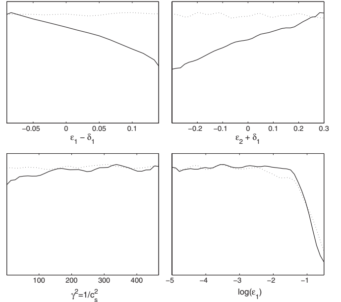
FIG. 5. Marginalized posterior probability distribution for the DBI primordial parameters by including the non-Gaussianity bounds on f_{\text{NL}} . The first Hubble flow parameter \epsilon_1 is now upper limited.
