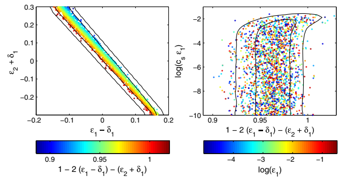
FIG. 3 (color online). Two-dimensional marginalized posteriors (point density) together with the one- and two-sigma contours. Although (\epsilon_1 - \delta_1) and (\epsilon_2 + \delta_1) are not bounded, they are strongly correlated to give acceptable values of the spectral index (left panel). The right panel exhibits the correlations between \log(\epsilon_1 c_s) and n_s = 1 - 2(\epsilon_1 - \delta_1) - (\epsilon_2 + \delta_1) .
