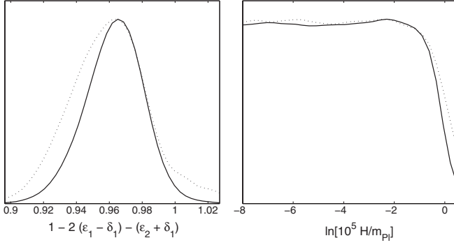
FIG. 4. Marginalized posterior probability distribution for the derived primordial parameters n_s and H_{\text{inf}} obtained by importance sampling.
