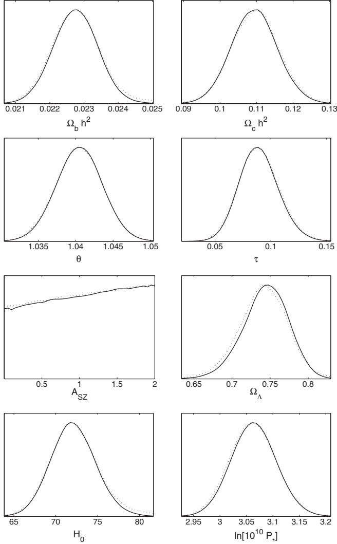
FIG. 1. One-dimensional marginalized posterior probability distribution (solid) and mean likelihoods (dotted) for the base and derived cosmological parameters, given the WMAP5 data and the k -inflation power spectra of Eq. (8).
