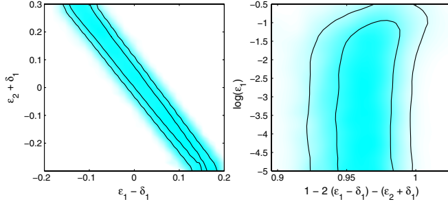
FIG. 6 (color online). One- and two-sigma contours of the two-dimensional marginalized posteriors for correlated pairs of primordial parameters. The shading traces the two-dimensional mean likelihood. The right panel shows that the non-Gaussianity bound on f_{\text{NL}} induces an upper bound on the first Hubble flow parameter \epsilon_1 .
