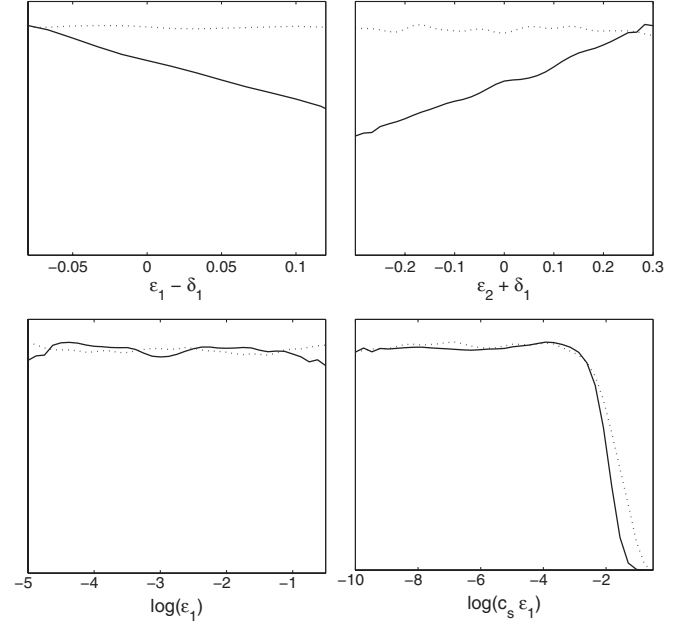
FIG. 2. One-dimensional marginalized posterior probability distribution (solid) and mean likelihood (dotted) for the sampled sound and Hubble flow parameters given the WMAP5 data. Only \log(\epsilon_1 c_s) is upper limited, this parameter fixing the tensor-to-scalar ratio. Notice, in particular, that \epsilon_1 is not constrained. The parameters (\epsilon_1 - \delta_1) and (\epsilon_2 + \delta_1) are, however, correlated (see Fig. 3).
