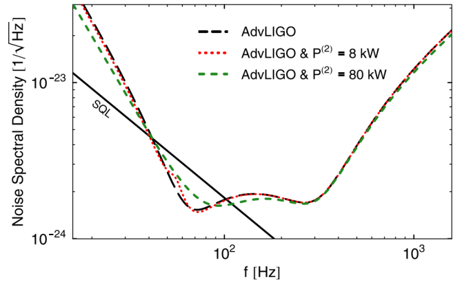
FIG. 5 (color online). Noise spectrum of weak-stabilization DOS configurations, with parameters corresponding to the configuration in Fig. 3. Namely, the first carrier is identical to the carrier in the Advanced LIGO narrowband mode (cf. Table I). Two possible choices for the stabilizing second carrier are (i) P^{(2)} = 8 kW, \epsilon^{(2)} = 2\pi 5 Hz, \lambda^{(2)} = -2\pi 55 Hz and (ii) P^{(2)} = 80 kW, \epsilon^{(2)} = 2\pi 60 Hz, \lambda^{(2)} = -2\pi 60 Hz. Phase quadrature detection ( \zeta^{(2)} = 0 ) in both cases.
