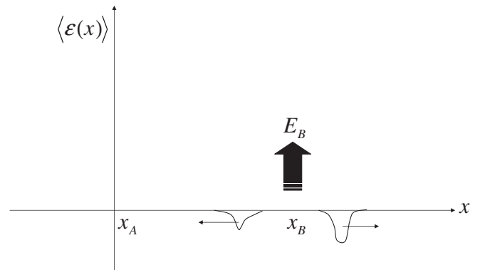
FIG. 3. The third schematic diagram of QFET. In the process of U_n(B) , Bob gets a positive amount of energy from the field, generating negative-energy wave packets in the field system.
