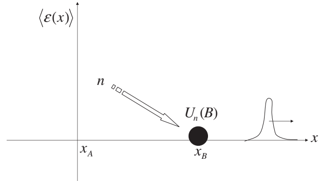
FIG. 2. The second schematic diagram of QFET. After the wave packet passes through Bob's location, Alice announces to Bob the measurement result n . Bob obtaining n performs local unitary operation U_n(B) depending on n .
