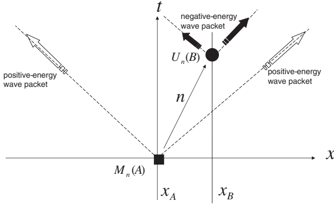
FIG. 4. A spacetime diagram of QFET. Entanglement is created between positive-energy wave packets generated by Alice and negative-energy wave packets generated by Bob, which form a loosely bound state.
