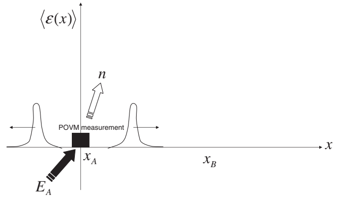
FIG. 1. The first schematic diagram of QFET. Alice stays at x = x_A and Bob at x = x_B . Alice performs a general measurement to the vacuum state with energy input E_A and obtains the measurement result n . Then, positive-energy wave packets are generated in the system and escape to spatial infinity at the speed of light. The expectational value of the energy density \langle \varepsilon(x) \rangle = \text{Tr}[\rho \hat{\varepsilon}(x)] is plotted as a function of x .
