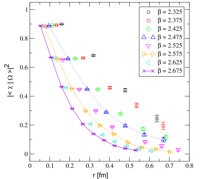
FIG. 2 (color online). Overlap between the axial state and the ground state, plotted against the physical separation of the charges. Some lines have been added to guide the eye. It is seen that, for all r , the overlap is smaller for finer lattice spacings (larger \beta ).
