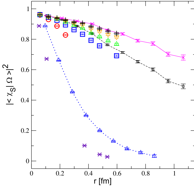
FIG. 4 (color online). Smeared state overlap with the ground state, plotted against physical separation. Axial state data ( S = 0 ) is displayed for comparison and some lines have been added to guide the eye. Legend as in Fig. 3.
