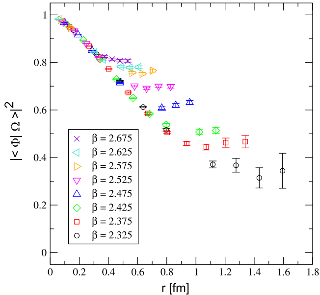
FIG. 9 (color online). Wilson action overlap of the Coulomb state and ground state, plotted against the physical separation of the charges. The overlap increases as we increase \beta .
