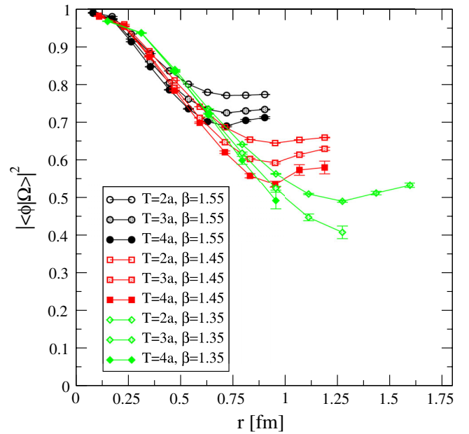
FIG. 7 (color online). A summary of the improved action results for the Coulomb overlap, plotted at a range of \beta and T values.
