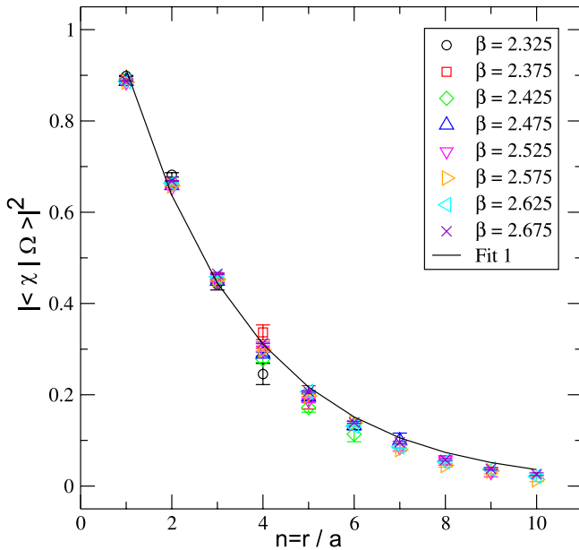
FIG. 1 (color online). Overlap between the axial state and the ground state, at various lattice spacings, plotted against the number of lattice points n = r/a between charges (for simulation details, see the text). The overlap is independent of \beta .
