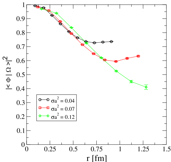
FIG. 6 (color online). Improved action simulation of the overlap between the Coulomb and ground states. At a fixed time, here T = 3a , we observe an increase in the overlap in the continuum limit ( \beta \rightarrow \infty or a \rightarrow 0 ).
