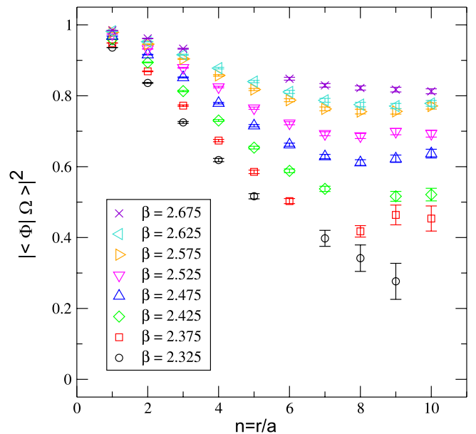
FIG. 8 (color online). Wilson action overlap of the Coulomb state and ground state, plotted against the number of lattice sites n = r/a between the charges. For lattice data, see the text. Measurements were taken from T \geq 3a . Notably, the overlap increases as we go to the continuum, \beta \rightarrow \infty .
