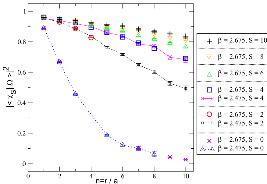
FIG. 3 (color online). Smeared state overlap with the ground state at various lattice spacings. For a fixed smearing level S the results lie on the same curve, they are \beta independent. We have added data for the axial state ( S = 0 ) for comparison, and some lines to guide the eye. Lattice: 500 configurations, T = 4a , relative error of Wilson line correlator < 0.5 , \chi^2/\nu < 3 and Q > 10^{-2} .
