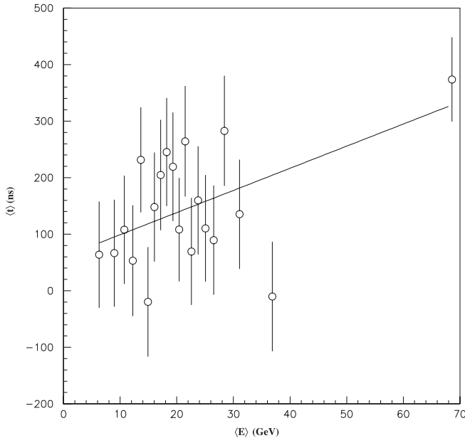
FIG. 13. The measured shifts in the average arrival times of neutrinos in 1000-event slices with increasing energies, assuming a time delay during neutrino propagation at the level of \tau = 5 ns/GeV.
