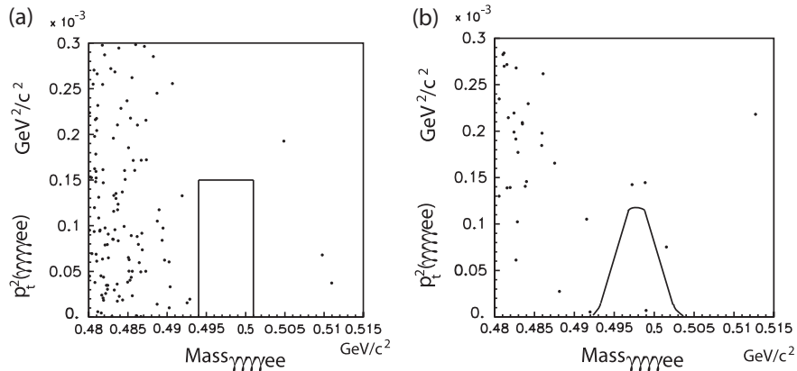
FIG. 3. (a) M_{ee\gamma\gamma\gamma} vs p_T^2(ee\gamma\gamma\gamma) for the 1997 KTeV data; (b) M_{ee\gamma\gamma\gamma} vs p_T^2(ee\gamma\gamma\gamma) for the 1999 KTeV data.
