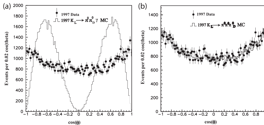
FIG. 1. (a) comparison of \cos(\theta) for a K_L \rightarrow \pi^0 \pi_D^0 \gamma signal MC vs \cos(\theta) as observed in the 1997 data; (b) comparison of \cos(\theta) for the K_L \rightarrow \pi^0 \pi^0 \pi_D^0 background MC vs \cos(\theta) for the 1997 data.
