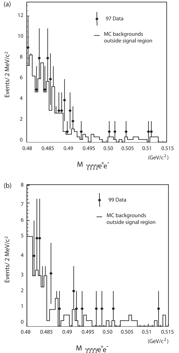
FIG. 2. Data and Monte Carlo background comparisons passing all cuts except the signal region contours of Fig. 3 for (a) the 1997 run; (b) the 1999 run.
