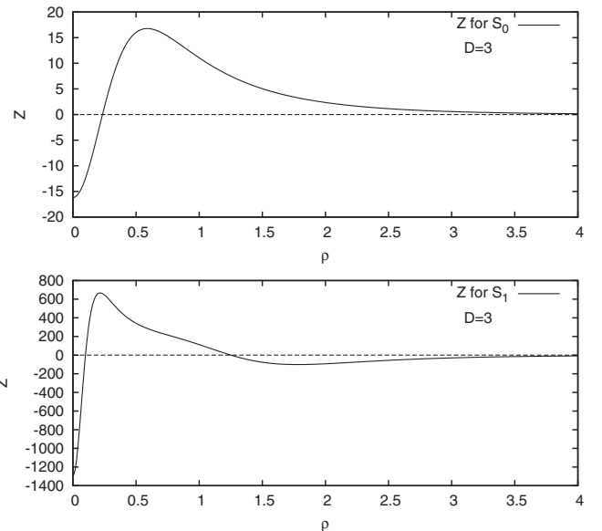
FIG. 4. Solutions of Eq. (45) in three dimensions. The central values of Z are -16.174 03 and -1290.021 .
