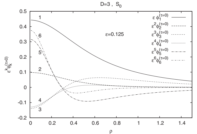
FIG. 5. Contributions of the various \varepsilon^k order terms corresponding to S_0 to the scalar field, \phi , at the moment of time symmetry \tau = 0 in D = 3 . The value of \varepsilon has been chosen to be 0.125, which brings the contribution of different terms to the same order. This value of \varepsilon is an obvious upper limit for the range of validity of our expansion.
