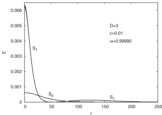
FIG. 17. Energy density \mathcal{E} of oscillon configurations evolved from S_0 and S_1 initial data, using \epsilon = 0.01 . The energy density is plotted on the same uniformly placed moments of time as in Fig. 16. The minimum of \mathcal{E} in the S_1 case remains below 10^{-7} near r = 51.3 .
