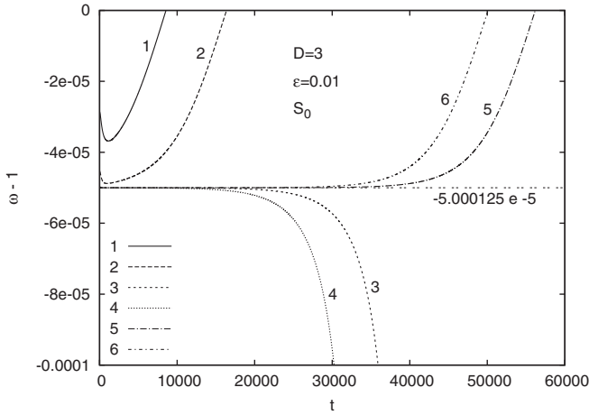
FIG. 13. Time evolution of the frequency of the oscillations of \phi evolving from initial data with \varepsilon = 0.01 in the D = 3 case. Since the frequency is very close to 1, the value \omega - 1 is plotted instead of \omega .
