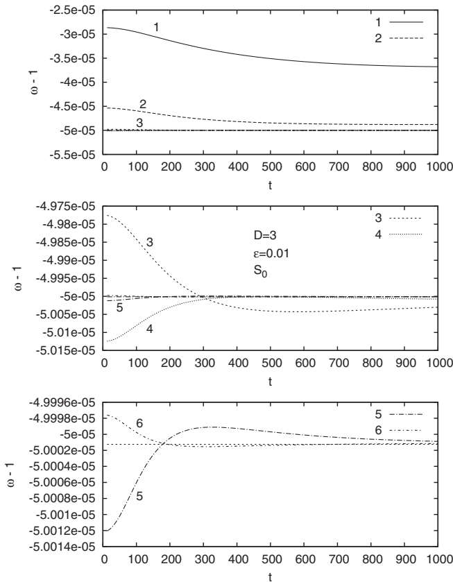
FIG. 14. Beginning of the time-evolution simulations shown on Fig. 13. For this shorter time interval the difference from the expected solution with \omega = 0.999\,949\,998\,75 decreases monotonically with the order of the \varepsilon approximation.
