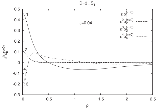
FIG. 6. \varepsilon^k \phi_k^{(\tau=0)} corresponding to the solution S_1 , with one node in the three dimensional case. Because of the sharp increase of the higher order functions, the value of \varepsilon was chosen to be much smaller as for S_0 .
