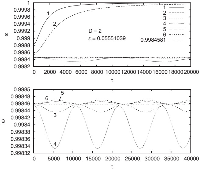
FIG. 19. The frequency as a function of time for the evolution of initial data with \varepsilon = 0.05551039 in case of D = 2 .
