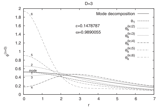
FIG. 9. Comparison of the value of the field at \tau = 0 obtained by the \varepsilon expansion to a very precise value obtained by a high order Fourier mode decomposition for \omega = 0.9890055 , i.e. for \varepsilon = 0.1478787 in D = 3 . For such a large value of \varepsilon the first order approximation gives a remarkably good estimate in the neighborhood of the central region. The contributions of the higher order approximations make this agreement increasingly worse in the neighborhood of the origin. Farther away from the center, however, the third order approximation gives the best, although not a very precise, result.
