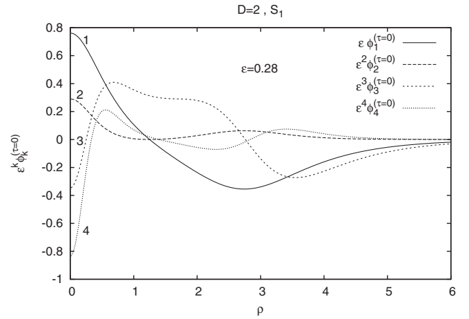
FIG. 8. \varepsilon^k \phi_k^{(\tau=0)} for D = 2 and with S_1 . The value of \varepsilon is the same as on Fig. 7. The contribution of the higher order terms is bigger than for S_0 , nevertheless it is smaller than for D = 3 .
