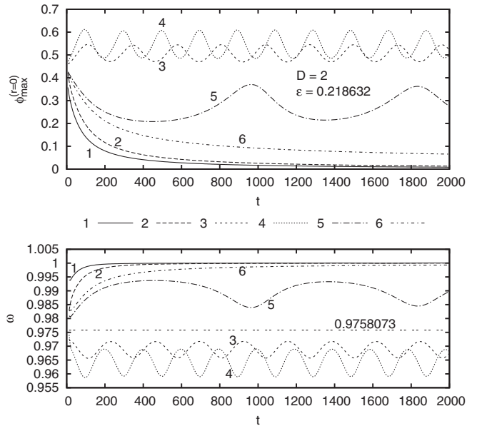
FIG. 18. Time evolution of the initial data produced by various order \epsilon expansions for \epsilon = 0.218632 in the two dimensional case. The top graph shows the upper envelope of \phi at r = 0 , while the bottom graph the time dependence of the frequency. The evolution of the third and fourth order initial data clearly corresponds to some oscillon state deformed by a low frequency ringing mode. The evolution of the fifth order initial data corresponds to a similar state with extreme high amplitude ringing. The first, second and sixth order initial data evolve into decaying modes, indicating a large error at these orders of the \epsilon expansion.
