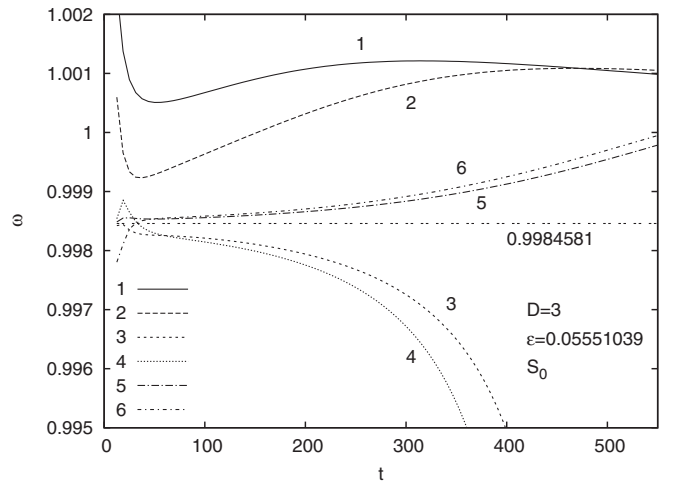
FIG. 12. Oscillation frequency as a function of time for the states shown on Fig. 11.
