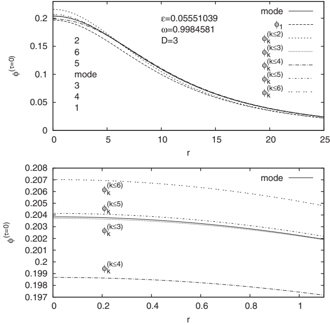
FIG. 10. Comparison of various order \varepsilon expansions of \phi at \tau = 0 to the value obtained by Fourier mode decomposition for \omega = 0.9984581 i.e. for \varepsilon = 0.05551039 in the D = 3 case.
