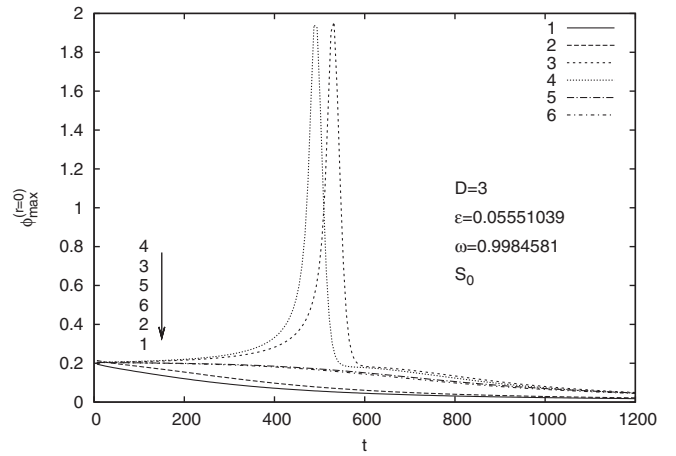
FIG. 11. Time evolution of the initial data obtained by the \varepsilon expansion method up to order six for \varepsilon = 0.05551039 in three spatial dimensions.
