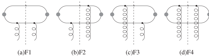
FIG. 8. The fermion diagrams for the impact factors.
