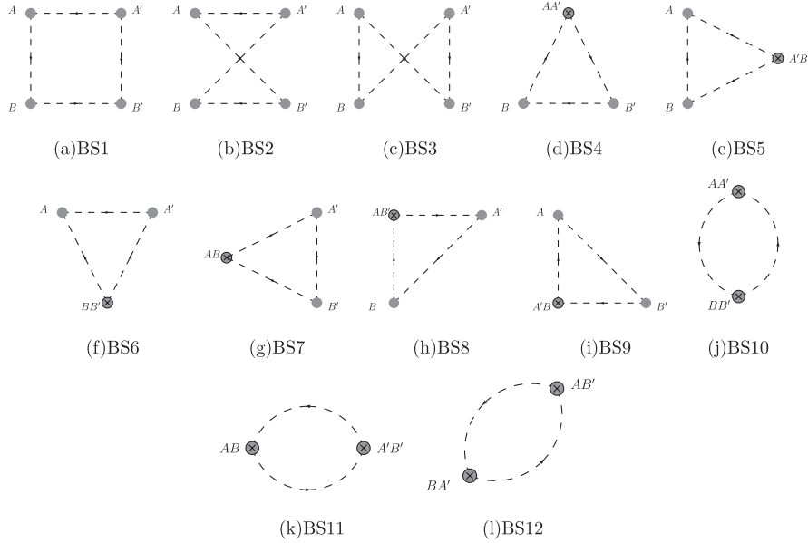
FIG. 6. One-loop diagrams with scalars.
