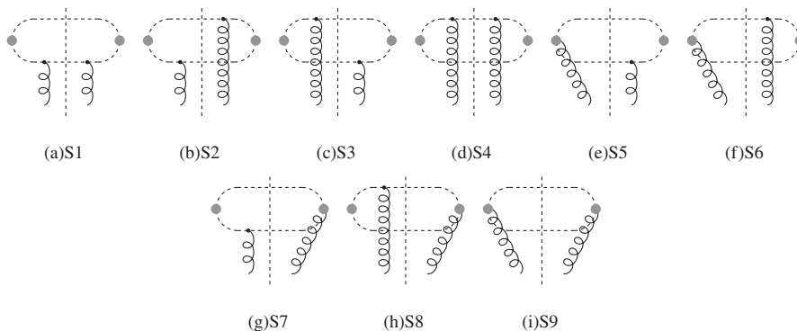
FIG. 9. The scalar diagrams for the impact factors.
