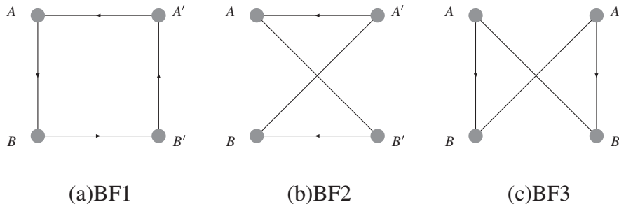
FIG. 5. One-loop diagrams with fermions.
