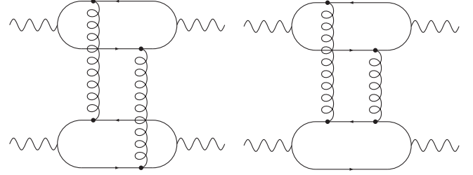
FIG. 2. An example of three-loop diagrams corresponding to two gluon exchange.
