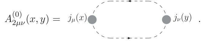
FIG. 4. Lowest order diagram contributing to the two point function of the electromagnetic current.
