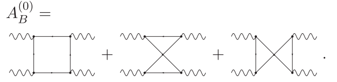
FIG. 1. Lowest order diagrams.
