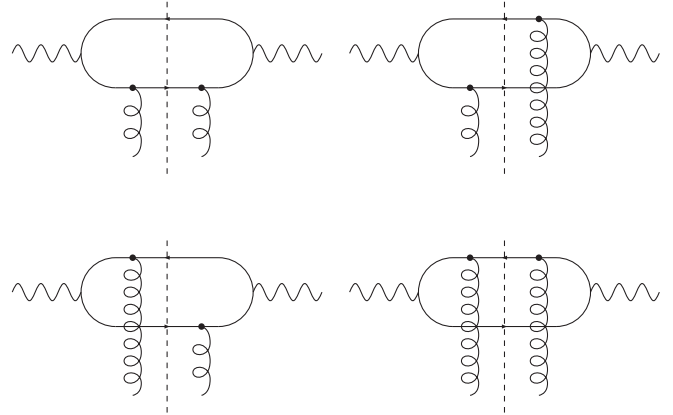
FIG. 3. The one-loop diagrams contributing to the impact factor \Phi .
