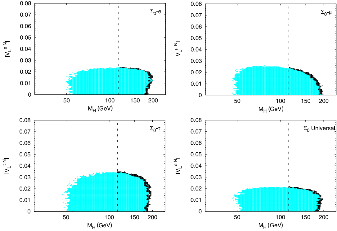
FIG. 5 (color online). The 90% confidence region in the |V_L^{eN}| - M_H parameter space for the \Sigma_0 triplet coupled to the first, second, and third families, respectively. The last plot corresponds to the universal case. In all cases the 90% confidence region with the cut M_H \geq 114.4 GeV (represented by the vertical dashed line) is shown in black.
