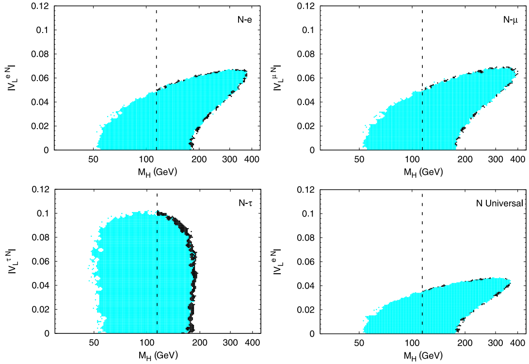
FIG. 1 (color online). The 90% confidence region in the |V_L^{eN}| - M_H parameter space for the N singlet coupled to the first, second, and third families, respectively. The last plot corresponds to the universal case. In all cases the extension of the 90% confidence region with the cut M_H \geq 114.4 GeV (represented by the vertical dashed line) is shown in black.
