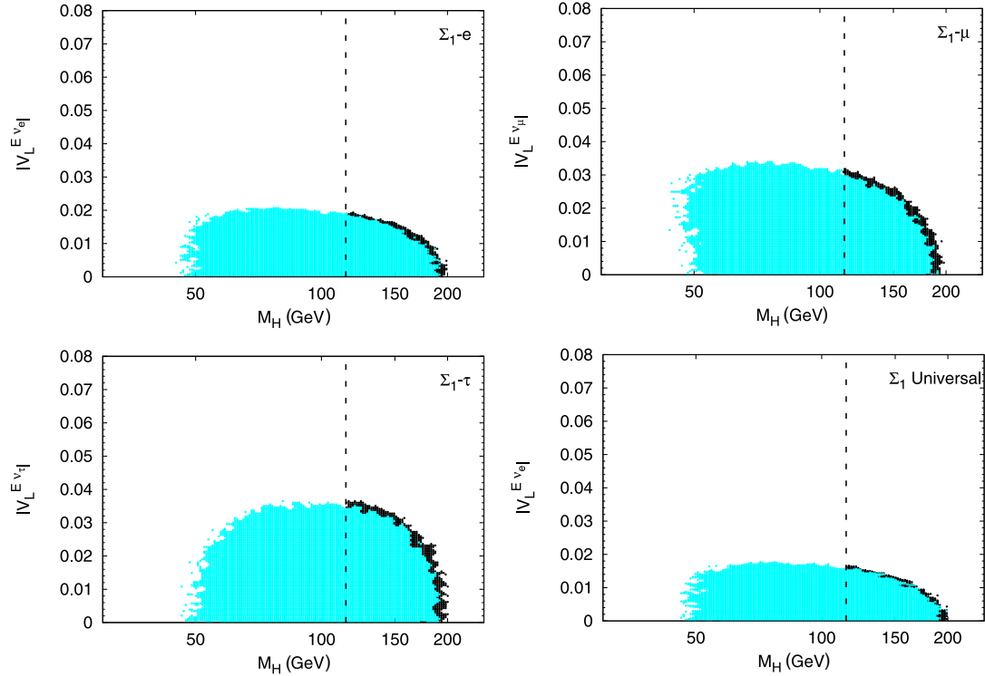
FIG. 6 (color online). The 90% confidence region in the |V_L^{E\nu}| - M_H parameter space for the \Sigma_1 triplet coupled to the first, second, and third families, respectively. The last plot corresponds to the universal case. In all cases the 90% confidence region with the cut M_H \geq 114.4 GeV (represented by the vertical dashed line) is shown in black.
