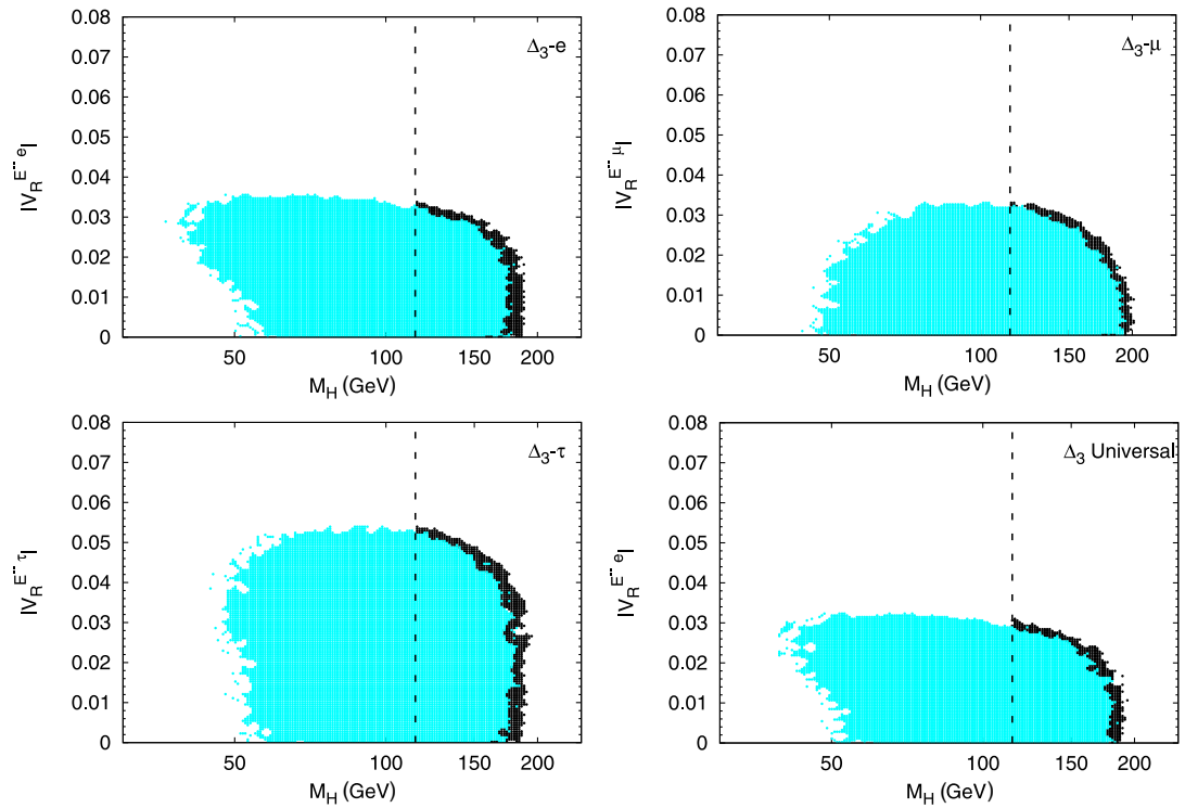
FIG. 4 (color online). The 90% confidence region in the |V_R^{E^+ e}| - M_H parameter space for the \Delta_3 doublet coupled to the first, second, and third families, respectively. The last plot corresponds to the universal case. In all cases, the extension of the 90% confidence region with the cut M_H \geq 114.4 GeV (represented by the vertical dashed line) is shown in black.
