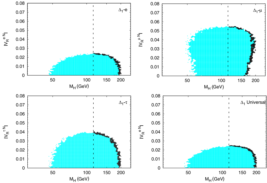
FIG. 3 (color online). The 90% confidence region in the |V_R^{eN}| - M_H parameter space for the \Delta_1 doublet coupled to the first, second, and third families, respectively. The last plot corresponds to the universal case. In all cases, the extension of the 90% confidence region with the cut M_H \geq 114.4 GeV (represented by the vertical dashed line) is shown in black.
