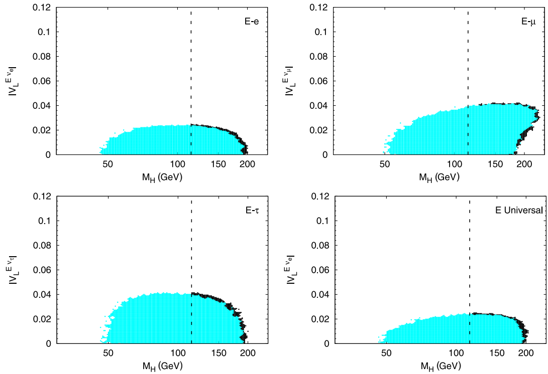
FIG. 2 (color online). The 90% confidence region in the |V_L^{E\nu}| - M_H parameter space for the E singlet coupled to the first, second, and third families, respectively. The last plot corresponds to the universal case. In all cases, the extension of the 90% confidence region with the cut M_H \geq 114.4 GeV (represented by the vertical dashed line) is shown in black.
