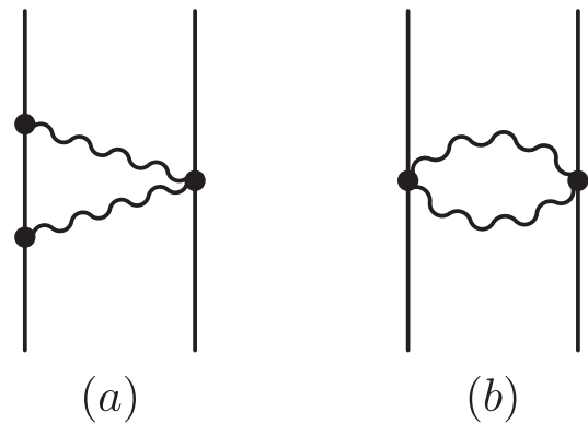
FIG. 3. Triangle and bubble diagrams used to evaluate the electromagnetic scattering of a charged and a neutral system.
