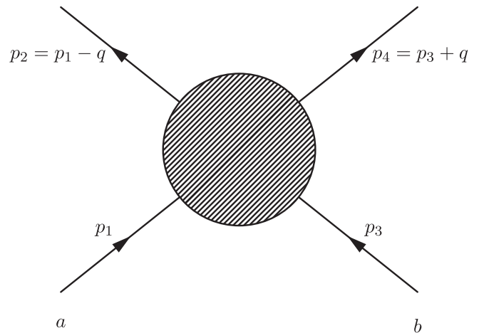
FIG. 1. Basic kinematics of electromagnetic scattering.
