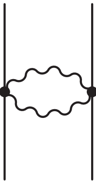
FIG. 2. Bubble diagram used to evaluate the electromagnetic scattering of two neutral systems.
