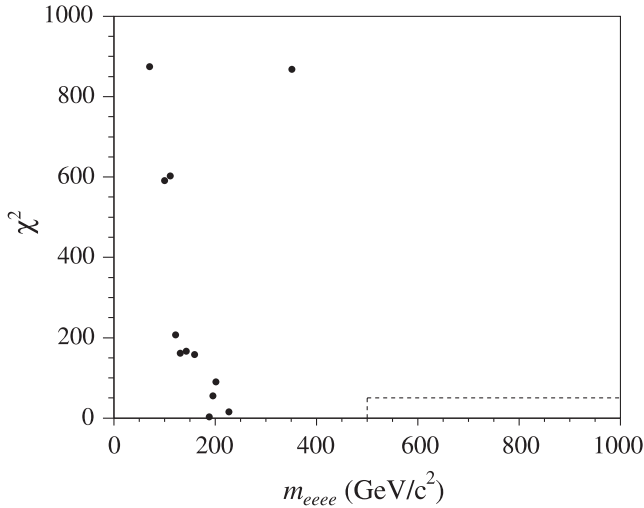
FIG. 7. Distribution of \chi^2 vs m_{eeee} for four-electron candidates in data. The signal region is \chi^2 < 50 and m_{eeee} > 500 \text{GeV}/c^2 , the boundaries of which are shown by the dashed line.
