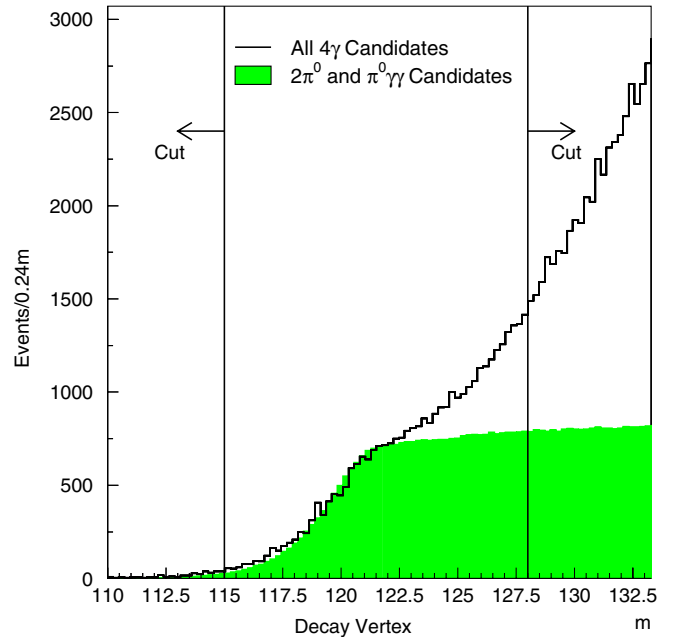
FIG. 4 (color online). The reconstructed decay vertex position from four photons for all events (histogram) prior to imposing the decay vertex cut. All cuts except for the decay vertex and photon shape \chi^2 have been applied. The shaded histogram indicates K_L \rightarrow \pi^0 \pi^0 and K_L \rightarrow \pi^0 \gamma \gamma candidates. The rise at large values is due to K_L \rightarrow \pi^0 \pi^0 \pi^0 decays in which one or more photons misses the CsI calorimeter. The position of the cut is indicated by the two vertical lines.
