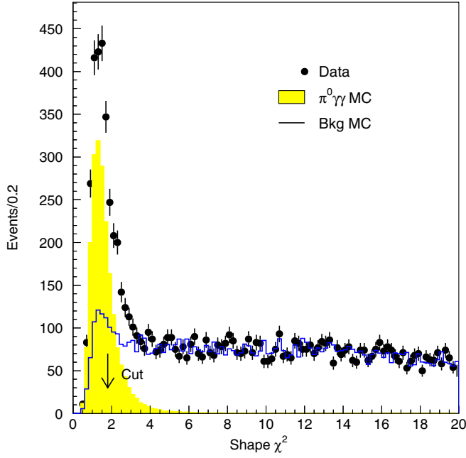
FIG. 5 (color online). The photon shape \chi^2 variable. The solid histogram shows the K_L \rightarrow \pi^0 \pi^0 \pi^0 Monte Carlo while the dotted histogram is the data. The K_L \rightarrow \pi^0 \gamma \gamma signal Monte Carlo simulation is the shaded histogram. The sum of the signal plus background Monte Carlo simulation agrees well with the data.
