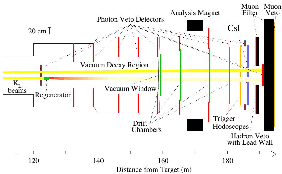
FIG. 1 (color online). Schematic of the KTeV detector.
