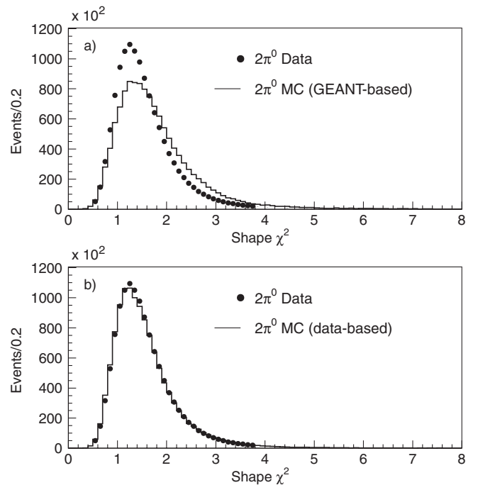
FIG. 3. The photon shape \chi^2 variable. (a) The photon shape \chi^2 variable for K_L \rightarrow \pi^0 \pi^0 with the dots representing the data and the solid histogram the Monte Carlo simulation. The Monte Carlo simulation was generated using our GEANT-based shower library. (b) The photon shape \chi^2 variable for K_L \rightarrow \pi^0 \pi^0 events. The dots are the data and the histogram represents the Monte Carlo simulation using our data-based shower library. The data-based Monte Carlo simulation shows marked improvement over the GEANT-based shower library.
