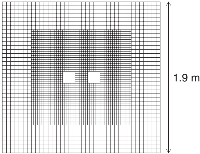
FIG. 2. Transverse view of the KTeV CsI calorimeter. The smaller blocks are located in the central region with the larger blocks located in the outer region.
