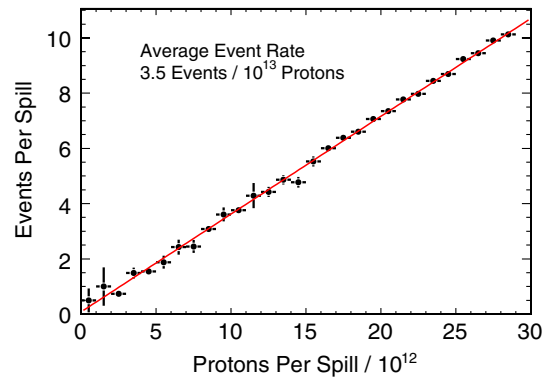
FIG. 13 (color online). Mean number of reconstructed events per Near Detector spill as a function of spill intensity.
