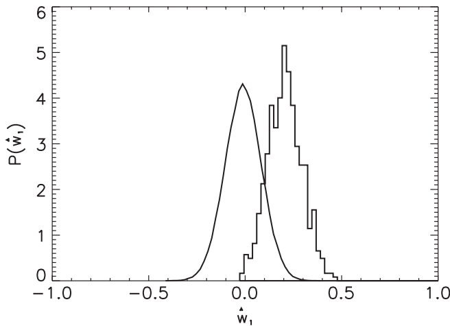
FIG. 6. Histogram of the joint estimator \hat{w}_1 coming from 545 3D realization of the dipole modulation model with w_1 = 0.2 and \tau = 0.09 . For comparison, the probability distribution for the isotropic w_1 = 0 model from Fig. 4 is also plotted (smooth curve).
