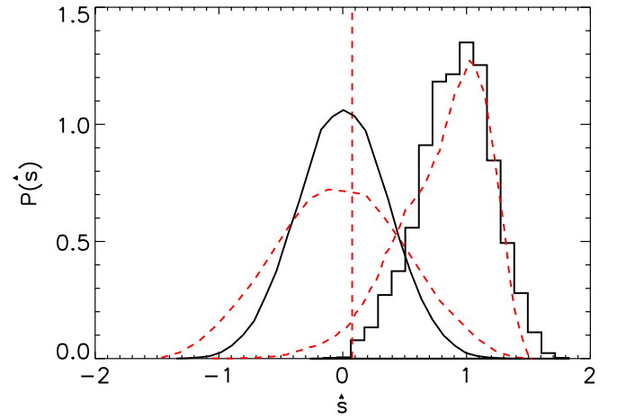
FIG. 14 (color online). Distribution of \ell \pm 2 correlation statistic \hat{s} . Distributions on the right with \langle \hat{s} \rangle = 1 represent the modulated model of Eq. (24) for the joint estimator (black solid lines) and the temperature estimator (red dashed lines). Curves on the left with \langle \hat{s} \rangle = 0 represent the isotropic Sachs-Wolfe model in the same manner. The histogram comes from 3482 3D realizations of the modulated model and other distributions from 10^5 2D realizations. The vertical red dashed line represents the observed value for temperature only for this modulated model, using the WMAP ILC map: \hat{s} = 0.076 .
