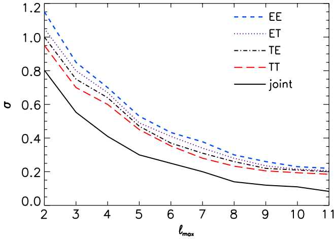
FIG. 5 (color online). Standard deviation of the individual estimators \hat{w}_1^{XY} and the joint estimator (black) as a function of maximum multipole pair employed in the estimators \ell_{\max} . The individual XY pairs are TT (red long-dashed curve), TE (black dotted-dashed curve), ET (violet dotted curve), and EE (blue dashed curve) from the analytic calculation of the appendix.
