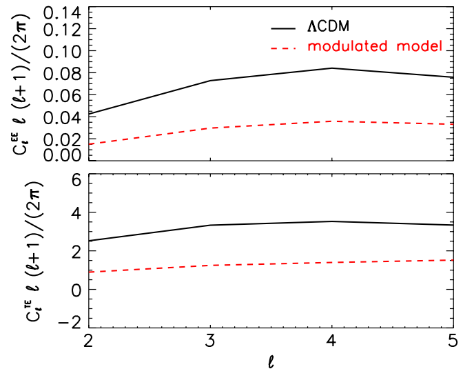
FIG. 13 (color online). EE and TE power spectra of the modulated model of Eq. (24) (red dashed lines) along with the \Lambda CDM power spectrum (black solid lines). The modulated model has a lower polarization at the same \tau (= 0.09) . The units are (\mu\text{K})^2 .
