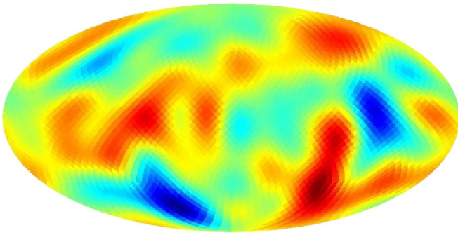
FIG. 3 (color online). Map composed of the first 10 multipoles of the E polarization field in a dipole modulation model with w_1 = 2.5 . The power is larger in the southern hemisphere.
