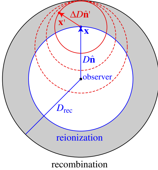
FIG. 2 (color online). Schematic diagram for polarization generation. After reionization, free electrons along the line of sight \hat{n} at a position \mathbf{x} see a quadrupole anisotropy on their recombination surfaces at a distance \Delta D in their angular coordinates \hat{n}' . Thomson scattering off these electrons produces the polarization field viewed by the observer at the origin in direction \hat{n} .
