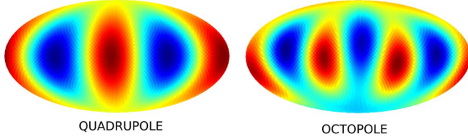
FIG. 10 (color online). Quadrupole and octopole of the temperature field from one realization of the quadrupole modulation model of Eq. (24). The normalized angular momentum here is \hat{L}_{23}^2 = 0.94 . The range goes from -50 \mu\text{K} to 50 \mu\text{K} for both cases.
