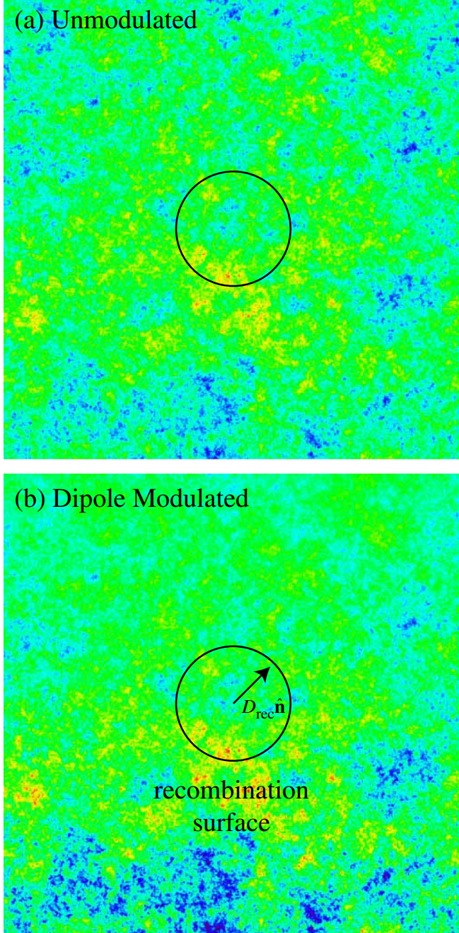
FIG. 1 (color online). Simulations of modulated temperature field. (a) Gaussian random unmodulated field g_1 . (b) Dipole-modulated potential field with h(\mathbf{x}) = w_1 \sqrt{3/4\pi} (z/D_{\text{rec}}) where the z axis is the modulation axis. Also shown (circle) is the surface at recombination upon which the observed temperature field originates. Note the power asymmetry in the modulated field.
