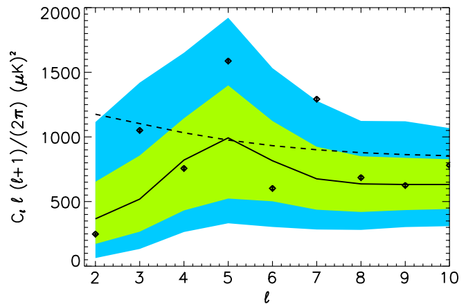
FIG. 9 (color online). Temperature angular power spectrum of the quadrupolar modulation model of Eq. (24) (solid line). The WMAP ILC data with noise errors are also shown. The solid bands correspond to the 68% and 95% cosmic variance confidence regions of the model. The dashed line represents the \Lambda CDM model against which this model is compared in Fig. 7.
