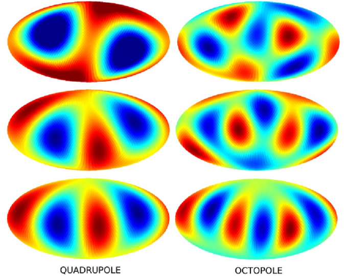
FIG. 12 (color online). Realizations of the quadrupole (left column) and octopole (right column) of the E component of the polarization field in order of increasing alignment: isotropic case with \hat{L}_{23}^{2(pol)} = 0.46 (first row), quadrupolar modulation model with parameters given by Eq. (24) with \hat{L}_{23}^{2(pol)} = 0.67 (second row) and an isotropic Sachs-Wolfe model constrained to match the WMAP ILC temperature multipoles with \hat{L}_{23}^{2(pol)} = 0.9 (third row). The color scale goes from -0.3 \mu\text{K} to 0.3 \mu\text{K} in all panels.
