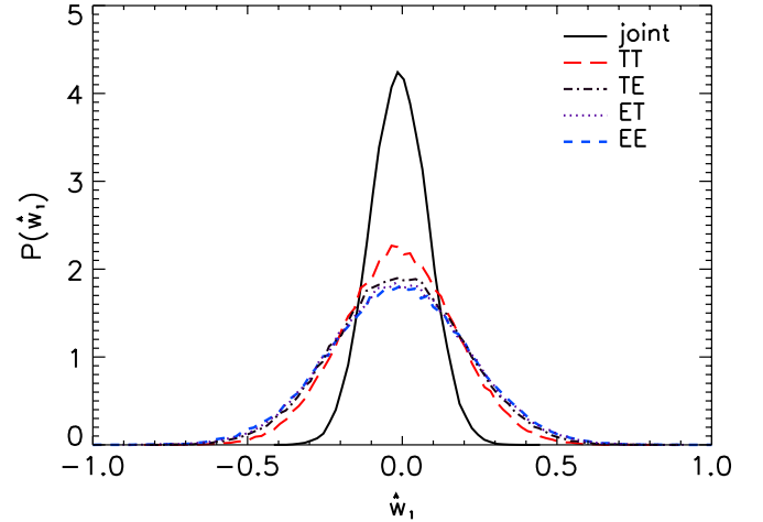
FIG. 4 (color online). Probability distribution of the dipole modulation estimators \hat{w}_1^{XY} for a model with w_1 = 0 where XY represents the two fields whose \ell and \ell + 1 multipoles are correlated: TT (red long-dashed curve), TE (black dotted-dashed curve), ET (violet dotted curve), and EE (blue thick dashed curve). The minimum variance joint estimator \hat{w}_1 is shown as the solid curve. We have assumed cosmic variance limited measurements and \ell_{\text{max}} = 11 for all estimators.
