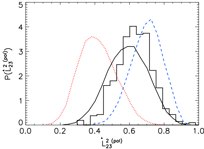
FIG. 11 (color online). Histogram of \hat{L}_{23}^{2(pol)} for 571 3D realizations of the quadrupole modulation model of Eq. (24) that also have \hat{L}_{23}^2 \geq 0.943 . For comparison we also show the distribution for isotropic random polarization fields (red dotted lines). Isotropic realizations constrained to the T_{\ell m} values of the ILC map have a distribution shifted to higher alignment values given the temperature-polarization correlation with just the Sachs-Wolfe effect (blue dashed lines) and with \Lambda\text{CDM} ISW contributions added (black solid curve).
