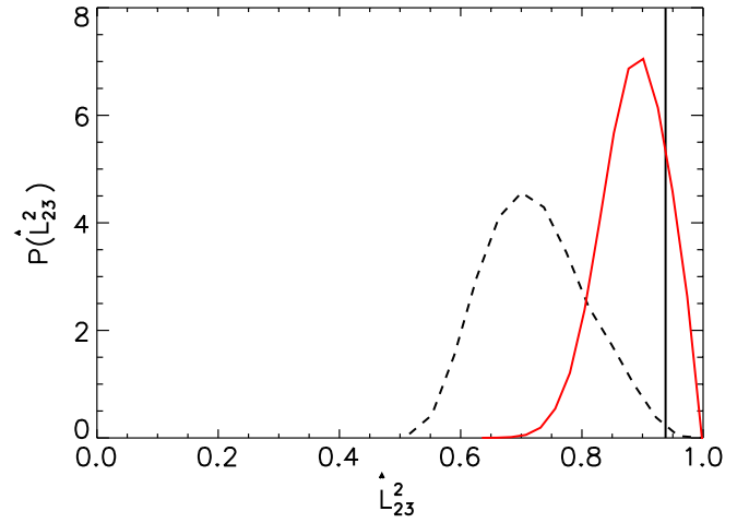
FIG. 8 (color online). Distribution of \hat{L}_{23}^2 (red solid line) for the quadrupolar modulation model of Eq. (24). 16.6% of the 10^4 realizations of this model have \hat{L}_{23}^2 > 0.943 . The distribution for the isotropic case is shown as a dashed line for comparison, where 0.85% have \hat{L}_{23}^2 larger than the WMAP ILC value: 0.943 (vertical line).
