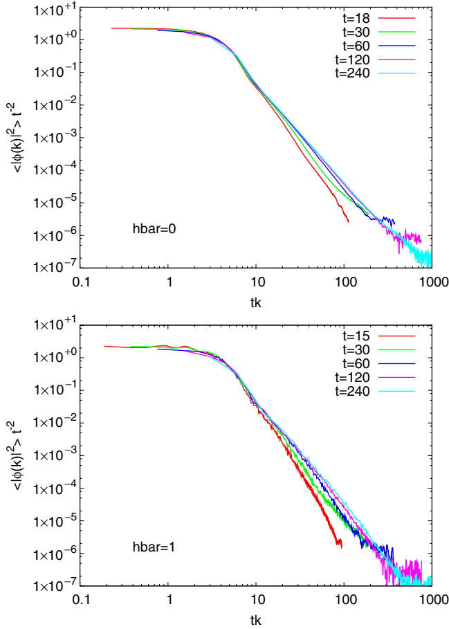
FIG. 4 (color online). The scaling of the power spectrum. The macroscopic part (domain walls) clearly follows the scaling law both in the classical (top) and in the quantum (bottom) case. The scaling breaks at the tail of the spectrum (small classical structures). ( L = 500 , average of 16000 and 192 runs for \hbar = 0 and 1, respectively.)
