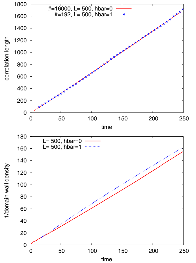
FIG. 5 (color online). The scaling of the correlation length (top) and the domain wall density (bottom).
