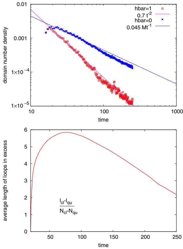
FIG. 6 (color online). Number of domains over lattice volume (top) in the classical and quantum framework. The classical scaling is counterintuitive. Dividing the difference of the total loop length by the number of loops (estimated by the number of domains) we get an average loop size (bottom).
