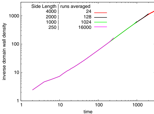
FIG. 1 (color online). Inverse domain wall density as a function of time. There is a perfect linear correspondence over more than 2 orders of magnitude ( t = 10 \dots 2000 ), from the time of ending the damped evolution at t = 10 to the end of the simulation, when the walls' mean curvature radius is over 10^3 times larger than their width.
