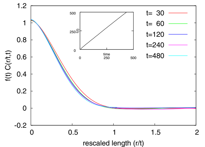
FIG. 3 (color online). Scaling of the equal time correlation function. Notice that the function has an approximate Gaussian shape, which is due to the nature of spinodal instability that created the domains. (There are deviations at small distance.) ( L = 1000, 1024 runs averaged.)
