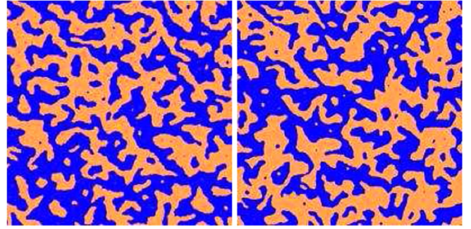
FIG. 2 (color online). Two snapshots of the lattice field configurations ( L = 2000 ). Blue and orange regions show the domains of the degenerate vacua. To the left, we show the configuration at t = 50 ; we cropped the region (0, L/2) \times (0, L/2) and scaled up by a factor of 2. To the right we show the uncropped lattice at t = 100 . There is no qualitative difference between the snapshots.
