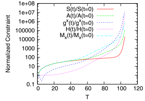
FIG. 11 (color online). The violation of all constraints normalized with their initial values, \|\delta\mathcal{C}\|_2(t)/\|\delta\mathcal{C}\|_2(0) , are plotted with a function of time. The evolutions of the gauge-wave test beds with the plain BSSN system are shown. The parameters of the test are the same as those shown in Sec. III A, and the lowest resolution run, \rho = 2 , is applied. By observing which constraint triggers the other constraint's violation from the constraint propagation equations, we may guess the mechanism by which the entire system is violating accuracy and stability. See the text for details.
