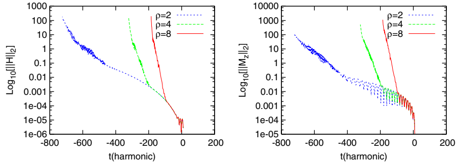
FIG. 7 (color online). Collapsing polarized Gowdy-wave test with the plain BSSN system. The L2 norm of \mathcal{H} and \mathcal{M}_z , rescaled by \rho^2/4 , are plotted with a function of the crossing time. (Simulation proceeds backwards from t = 0 .) We see almost perfect overlap for the initial 100 crossing time, and the higher resolution runs crash earlier. This result is quite similar to those achieved with the Cactus BSSN code, reported by [29].
