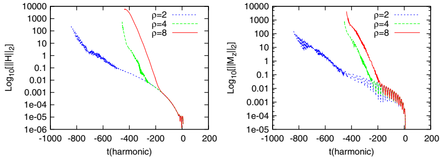
FIG. 9 (color online). Collapsing polarized Gowdy-wave test with the adjusted BSSN system in the \tilde{\gamma} -equation (2.21), with \kappa_{\tilde{\gamma}} = 0.000025 . The figure style is the same as Fig. 7. Note the almost perfect overlap for 200 crossing time in the both the Hamiltonian and momentum constraint and the \rho = 2 run can evolve stably for 1000 crossing time.
