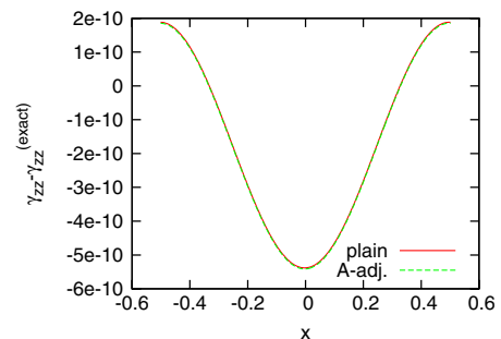
FIG. 6 (color online). Snapshot of errors with the exact solution for the linear wave test bed with the plain BSSN system and the adjusted BSSN system with the \tilde{A} -equation at T = 500 . The highest resolution \rho = 8 is used in both runs. The difference between the plain and the adjusted BSSN system with the \tilde{A} -equation is indistinguishable. Note that the maximum amplitude is set to be 10^{-8} in this problem.
