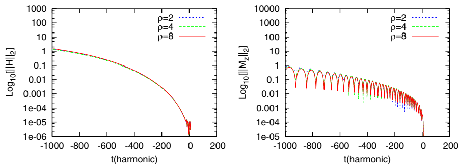
FIG. 8 (color online). Collapsing polarized Gowdy-wave test with the adjusted BSSN system in the \tilde{A} -equation (2.20), with \kappa_{\mathcal{A}} = -0.001 . The style is the same as in Fig. 7 and note that both constraints are normalized by \rho^2/4 . We see almost perfect overlap for the initial 1000 crossing time in both constraint equations, \mathcal{H} and \mathcal{M}_z , even for the highest resolution run.
