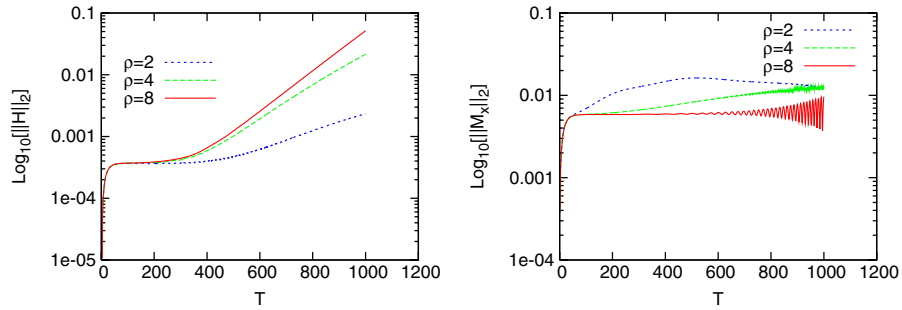
FIG. 2 (color online). The one-dimensional gauge-wave test with the adjusted BSSN system in the \tilde{A} -equation (2.20). The L2 norm of \mathcal{H} and \mathcal{M}_x , rescaled by \rho^2/4 , are plotted with a function of the crossing time. The wave parameter is the same as with Fig. 1, and the adjustment parameter \kappa_A is set to \kappa_A = 0.005 . We see the higher resolution runs show convergence longer, i.e., the 300 crossing time in \mathcal{H} and the 200 crossing time in \mathcal{M}_x with \rho = 4 and 8 runs. All runs can stably evolve up to the 1000 crossing time.
