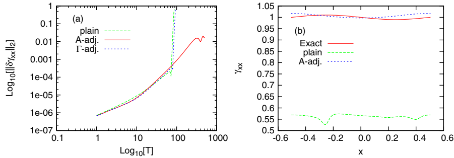
FIG. 4 (color online). Evaluation of the accuracy of the one-dimensional gauge-wave test bed. Lines show the plain BSSN, the adjusted BSSN with \mathcal{A} -equation, and with \tilde{\Gamma} -equation. (a) The L2 norm of the error in \gamma_{xx} , using (4.2). (b) A snapshot of the exact and numerical solution at T = 100 .
