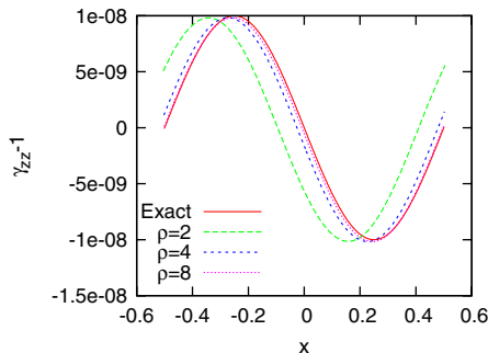
FIG. 5 (color online). Snapshots of the one-dimensional linear wave at different resolutions with the plain BSSN system at the simulation time 500 crossing time. We see there exists phase error, but they are convergent away at higher resolution runs.
