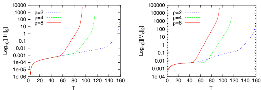
FIG. 3 (color online). The one-dimensional gauge-wave test with the adjusted BSSN system in the \tilde{\Gamma} -equation (2.22). The L2 norm of \mathcal{H} and \mathcal{M}_x , rescaled by \rho^2/4 , are plotted with a function of the crossing time. The wave parameter is the same as Fig. 1, and the adjustment parameter is \kappa_{\tilde{\Gamma}} = -0.1 . Note the near perfect overlap for the 55 crossing time in \mathcal{H} and the 40 crossing time in \mathcal{M}_x .
