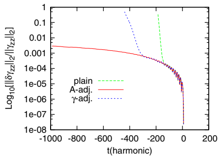
FIG. 10 (color online). Comparisons of systems in the collapsing polarized Gowdy-wave test. The L2 norm of the error in \gamma_{zz} , rescaled by the L2 norm of \gamma_{zz} , for the plain BSSN, adjusted BSSN with \tilde{A} -equation, and with \tilde{\gamma} -equation are shown. The highest resolution run, \rho = 8 , is depicted for the plots. We can conclude that the adjustments make longer accurate runs available. Note that the evolution is backwards in time.
