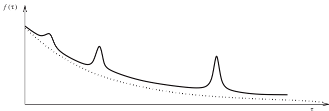
FIG. 3. Schematic drawing of the source term of the system of Eqs. (46).
