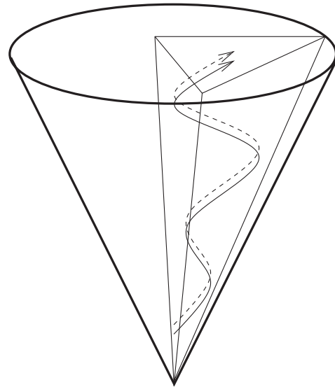
FIG. 4. Chaotic behavior .—This picture is a schematic drawing of the asymptotic dynamics of the ‘‘diagonal variables’’ at a given spatial point x , this dynamics is represented in the \beta -space. The dashed curve represents the zeroth order solution \beta_{[0]} . The exact solution is sketched as a continuous curve. The idea is that the approximate solution \beta_{[0]} becomes better and better as \tau \rightarrow +\infty ; this is formalized via a ‘‘generalized Fuchs theorem,’’ see the text. Note that here we consider a chaotic system and that the ‘‘fundamental chamber’’ determined by the walls is contained within the light cone.
