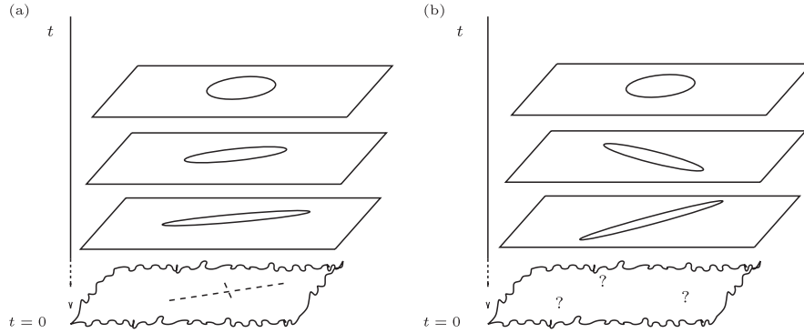
FIG. 1. (a) Nonchaotic behavior .—Sufficiently close to the singularity, the dynamics of the gravitational field can be approximated by a Kasner-like metric at each spatial point. Let us focus on one particular spatial point where asymptotically the metric is given by ds_{\text{spatial}}^2 = (t^{2p_1} l_i l_j + t^{2p_2} m_i m_j + \dots + t^{2p_d} r_i r_j) dx^i dx^j . When t \rightarrow 0 , the directions for which the Kasner exponent p_i is negative are stretched while the ones with positive exponent are squeezed. At the singularity, these directions are still defined. (b) Chaotic behavior .—Now instead of a Kasner-like metric at each spatial point, there is a never ending chaotic succession of Kasner epochs before reaching the singularity. Are there still some preferred directions at the singularity? Or is some other structure of the metric preserved asymptotically?
