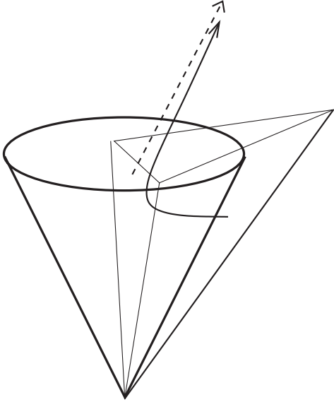
FIG. 2. Nonchaotic behavior. —This picture is a schematic drawing of the asymptotic dynamics of the “diagonal variables” at a given spatial point x , this dynamics is represented in the \beta -space. The dashed arrow represents the asymptotic solution \beta_{[0]} (which is valid after the last collision on a wall and corresponds to a free motion of the particle \beta ). The exact solution is sketched as a continuous curve. The idea is that the approximate solution \beta_{[0]} becomes better and better as \tau \rightarrow +\infty , this is formalized by the Fuchs theorem that tells us precisely how \beta - \beta_{[0]} \rightarrow 0 when \tau \rightarrow +\infty , see the text. Note that here we consider a nonchaotic system and that the “fundamental chamber” determined by the walls is not contained within the light cone.
