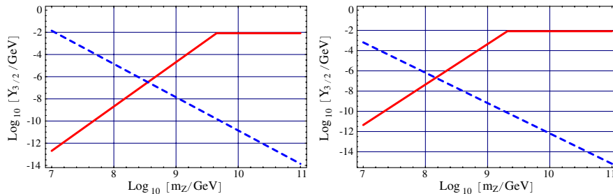
FIG. 2 (color online). The yield of gravitinos for m_{3/2} = 1 TeV (left), 100 GeV (right). Solid (red) lines denote the yields of gravitinos produced by the inflaton decay in Eq. (16) and dashed (blue) lines denote the yields produced by the decay of SUSY breaking field in Eq. (23). Here, we have taken C and C_0 to be 1 and T_R to be 10^7 GeV.
