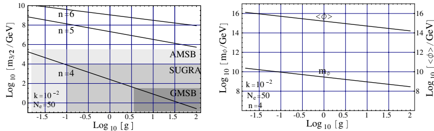
FIG. 1 (color online). (Left) The g dependence of the gravitino mass for a given value of n . The shaded regions represent the typical gravitino mass regions for GMSB ( m_{3/2} \lesssim 30 GeV), SUGRA [ m_{3/2} = O(100) GeV– O(1) TeV], and AMSB [ m_{3/2} = O(10) – O(100) TeV]. (Right) The g dependences of the mass and the VEV of the inflaton for n = 4 .
