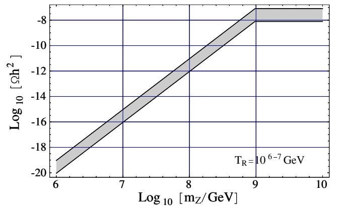
FIG. 4 (color online). The mass density parameter of gravitino produced by the decay of the inflaton for m_{3/2} = 10 GeV, T_R = 10^{6-7} GeV, and b = 0 . For simplicity, we have assumed \langle Z \rangle = 0 .
