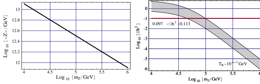
FIG. 3 (color online). (Left) The size of the VEV of the SUSY breaking field, \langle Z \rangle = (m_{3/2}^4 m_Z^{-3})^{1/5} , which we take as an example. (Right) The mass density parameter of the gravitino dark matter, \Omega_{3/2} h^2 , produced by the decay of SUSY breaking field. The shaded region corresponds to the density parameter for T_R = 10^{6-7} GeV. The solid (red) horizontal line shows the observed dark matter density \Omega h^2 = 0.1050_{-0.0040}^{+0.0041} (1\sigma) [28]. In both panels, we have taken m_{3/2} = 10 GeV.
