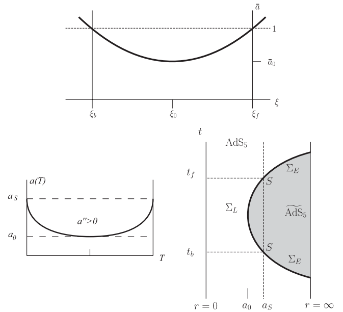
FIG. 1. The Lorentzian phase starts with a signature change at \xi_b , with a scale factor a = a_S ( \bar{a} = 1 ) and vanishing density \rho and pressure p . The model contracts until it reaches the minimum scale a_0 where \rho attains its maximum, which represents a little bang (regular bounce) [15]. The model then “bounces” to an expanding era with accelerated expansion ( a'' > 0 ), in which both \rho and p decrease, until another change of signature occurs at a = a_S , with \rho|_S = p|_S = 0 . The density and pressure remain non-negative everywhere on the Lorentzian phase. The picture on the bottom right describes the whole brane (with its Lorentzian, Euclidean, and null phases) embedded in the \text{AdS}_5 bulks, with \sigma = -\epsilon_1 = 1 and \tilde{\lambda} < \lambda , so that \rho > 0 in \Sigma_L . Observe that \rho|_{\Sigma_L} > 0 requires \Lambda_5 < \tilde{\Lambda}_5 < 0 so that the “eternal” \text{AdS}_5 is more stable. This is very reasonable physically [1].
