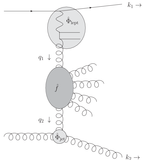
FIG. 1. Kinematics of the partonic cross section.
