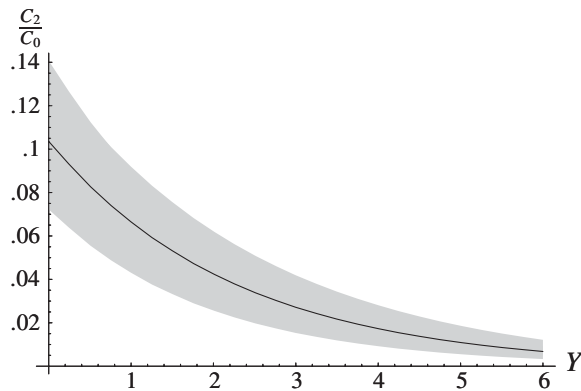
FIG. 3. \langle \cos 2\phi \rangle at the ep collider HERA for resummed kernel. The gray band reflects the uncertainty in s_0 and in the renormalization scale \mu .
