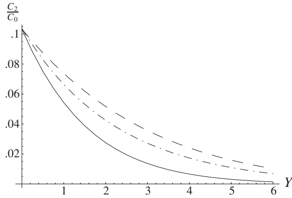
FIG. 2. \langle \cos 2\phi \rangle at the ep collider HERA at leading (solid line), next-to-leading order (dashed line), and for resummed kernel (dash-dotted line).
