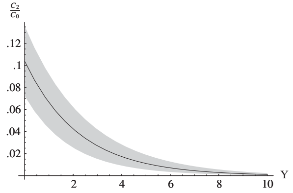
FIG. 4. \langle \cos 2\phi \rangle at a possible ep collider LHeC with a gray band reflecting the uncertainty in s_0 and in the renormalization scale \mu .
