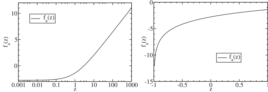
FIG. 2. UV-finite part of the function f_a(z) . Left panel: Euclidean values of z . Right panel: continuation of f_a(z) into the spacelike Minkowski region.
