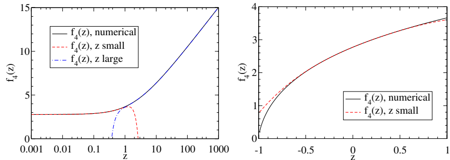
FIG. 3 (color online). The function f_4(z) and its asymptotic expansions for z \rightarrow 0 and v = 1/z \rightarrow 0 . Left panel: Euclidean values of z . Right panel: continuation of f_4(z) into the spacelike Minkowski region.
