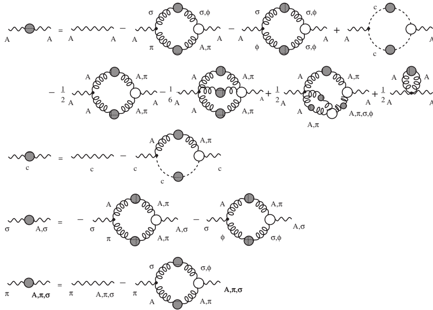
FIG. 1. A diagrammatic representation of the coupled system of Dyson-Schwinger equations. Filled blobs denote dressed propagators and empty circles denote dressed proper vertex functions. Wavy lines denote proper functions, springs denote connected (propagator) functions and dashed lines denote the ghost propagator. Labels indicate the various possible propagator and vertex combinations that comprise the self-energy terms.
