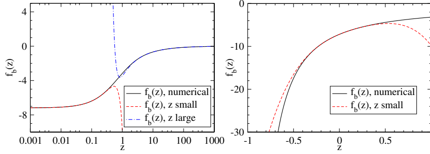
FIG. 4 (color online). UV-finite part of the function f_b(z) and its asymptotic expansions for z \rightarrow 0 and v = 1/z \rightarrow 0 . Left panel: Euclidean values of z . Right panel: continuation of f_b(z) into the spacelike Minkowski region.
