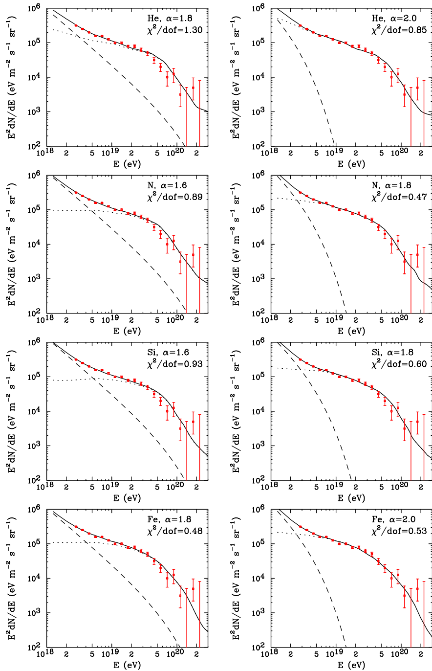
FIG. 3 (color online). The best fit spectrum for an all-helium, all-nitrogen, all-silicon, or all-iron UHECR composition (at injection) for different injected power-law slopes. The dotted, dashed, and solid lines denote the extragalactic, galactic, and combined components, respectively.
