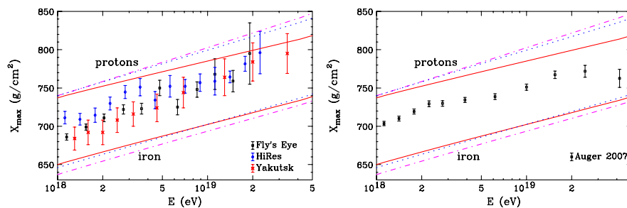
FIG. 2 (color online). The values of X_{\max} as a function of energy as measured by Fly's Eye [31], HiRes [10], and Yakutsk [32] (left frame) and as measured by the PAO [7] (right frame). The measurements are compared to the predictions for an all-proton and all-iron UHECR composition, using three different hadronic physics models. The dotted-dashed (magenta) line, solid (red) line, and dotted (blue) contours correspond to the models EPOS 1.6, QGSJET-III, and SIBYLL 2.1, respectively.
