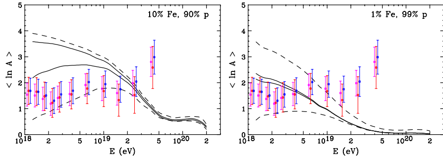
FIG. 6 (color online). The average composition at Earth for two mixtures of iron nuclei and protons in the injected spectrum. In each frame, an exponential energy cutoff of E_{\max} = 10^{22} \text{ eV} \times (Z/26) has been used. The solid lines denote the best fit model, with the split below \sim 10^{19} \text{ eV} resulting from variations in the composition of the galactic component. The range denoted by the dashed lines is that which is consistent with the spectrum measured by the PAO (within the 95% confidence level). The error bars denote the X_{\max} measurements using EPOS 1.6 [offset left (magenta)], QGSJET-III [center, red], and SIBYLL 2.1 [offset right (blue)].
