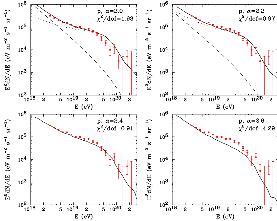
FIG. 1 (color online). The best fit spectrum for an all-proton UHECR composition for injected spectra with power-law slopes of 2.0, 2.2, 2.4, and 2.6. The dotted, dashed, and solid lines denote the extragalactic, galactic, and combined components, respectively. In the lower two frames, the best fit includes a negligible galactic component.
