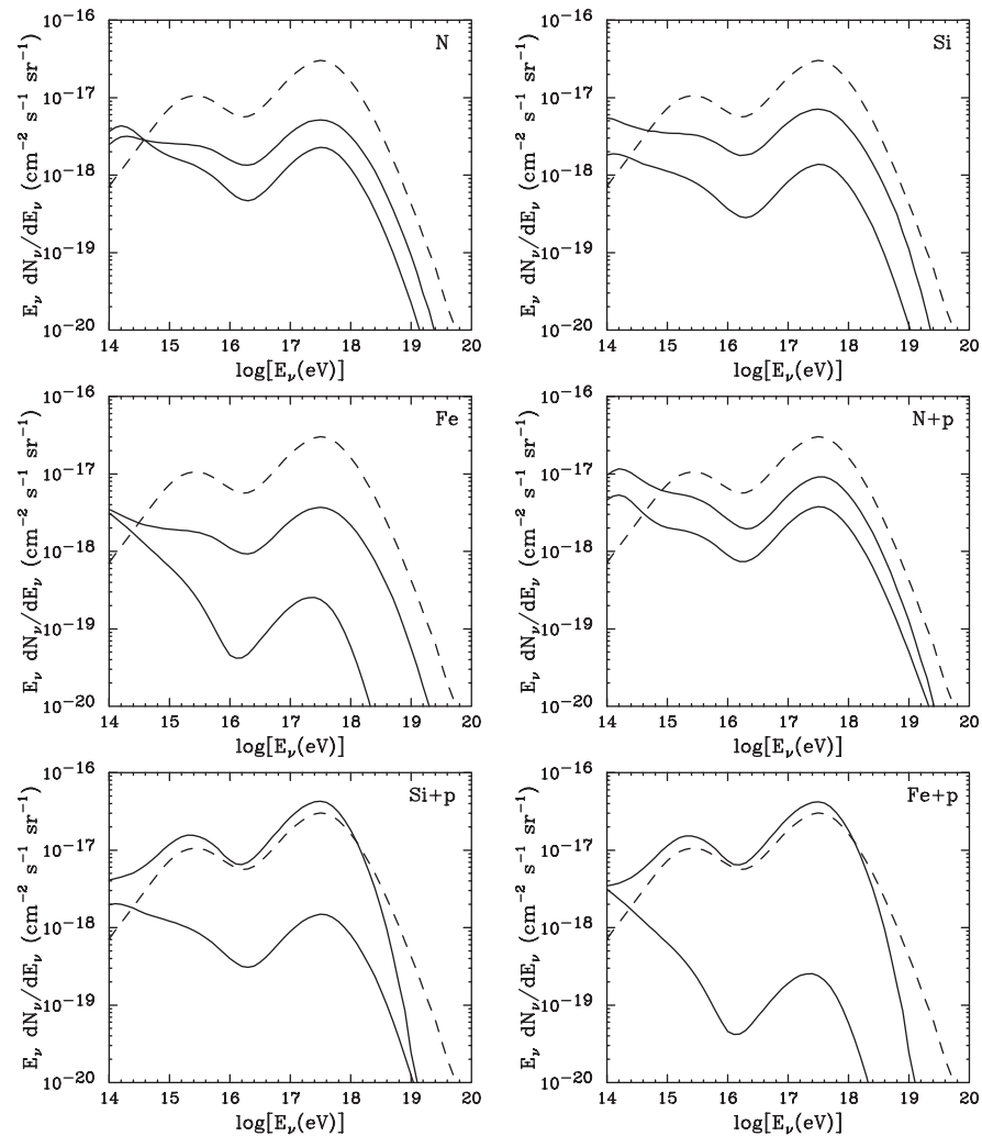
FIG. 7. The range of cosmogenic neutrino spectra we find for various chemical species which are consistent with both the PAO spectrum and X_{\max} measurements. In each case, we have considered model parameters in the range \alpha = 1.4\text{--}3.0 and E_{\max}/Z = 10^{20}\text{--}10^{22} \text{ eV} (although models with E_{\max}/Z below approximately 10^{21} \text{ eV} were found to be inconsistent with the data). In the N + p, Si + p, and Fe + p frames, we show the results for combinations of injected nuclei and protons. In each frame, we show for comparison as a dashed curve the prediction for an all-proton spectrum with \alpha = 2.2 and E_{\max} = 10^{22} \text{ eV} . The solid lines denote the models with the highest and lowest rates predicted in a neutrino telescope such as IceCube.
