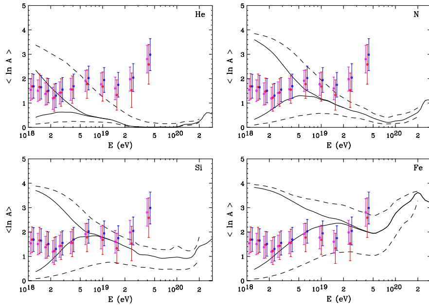
FIG. 4 (color online). The average composition at Earth for pure helium, nitrogen, silicon, or iron nuclei (at injection). The solid lines denote the model best fit to the PAO spectrum, with the range shown below \sim 10^{19} eV resulting from variations in the composition of the galactic component. The range denoted by the dashed lines is that which is consistent with the spectrum measured by the PAO (within the 95% confidence level). In each case, an exponential cutoff above E_{\text{max}} = 10^{22} eV \times (Z/26) was assumed. The error bars correspond to measurements of the elongation rate by the PAO using EPOS 1.6 [offset left (magenta)], QGSJET-III [red center (red)], and SIBYLL 2.1 [offset right (blue)], and in each case include both statistical and systematic uncertainties.
