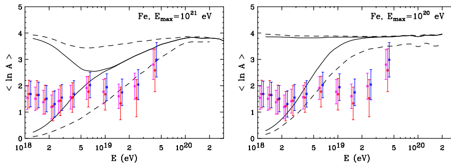
FIG. 5 (color online). The average composition at Earth for a pure iron UHECR spectrum at injection, for two values of the exponential cutoff in energy. The solid lines denote the best fit model, with the split below \sim 10^{19} eV resulting from variations in the composition of the galactic component. The range denoted by the dashed lines is that which is consistent with the spectrum measured by the PAO (within the 95% confidence level). The error bars denote the X_{\text{max}} measurements using EPOS 1.6 [offset left (magenta)], QGSJET-III [center (red)], and SIBYLL 2.1 [offset right (blue)].
