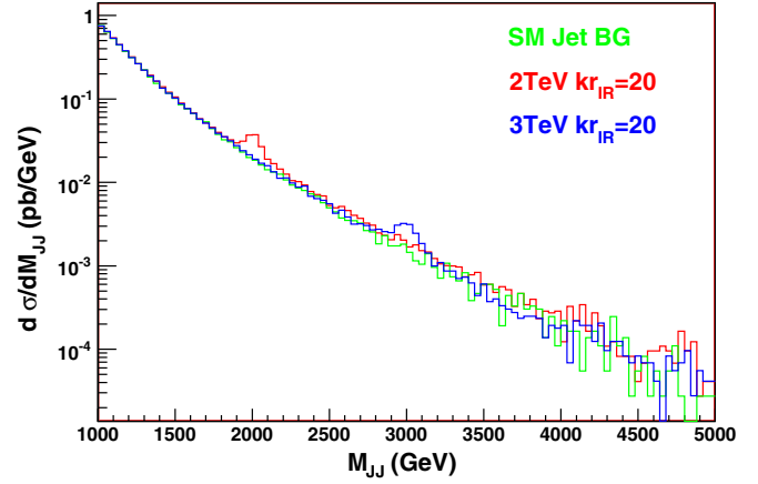
FIG. 7 (color online). Invariant mass distribution of QCD dijets coming from the KK-gluon resonance in models with large brane kinetic term ( \kappa r_{\text{IR}} = 20 ), and the SM prediction. The cuts p_T > 20 GeV, |\eta| < 1.0 , and invariant mass > 1 TeV are applied.
