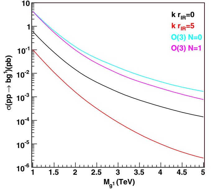
FIG. 5 (color online). Cross section for pp \rightarrow bg^1 at the LHC, for standard RS with the SM in the bulk ( \kappa r_{\text{IR}} = 0 ), a model with a large brane kinetic term ( \kappa r_{\text{IR}} = 5 ) and the model with a larger custodial symmetry, in the cases when 0(1) of the additional KK custodial partner quarks are light enough that g^1 can decay into them.
