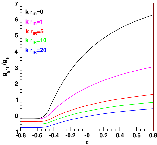
FIG. 2 (color online). Coupling of the first KK gluon (with respect to the zero mode gluon coupling) with \kappa r_{\text{IR}} = 0, 1, 5, 10, 20 (descending) to a fermion zero mode as a function of bulk mass parameter c .
