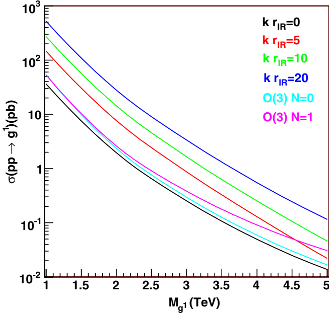
FIG. 4 (color online). Cross section for pp \rightarrow g^1 at the LHC, for standard RS with the SM in the bulk ( \kappa r_{\text{IR}} = 0 ), three models with large brane kinetic terms ( \kappa r_{\text{IR}} = 5, 10, 20 ), and the model with a larger custodial symmetry, in the cases when N = 0 or 1 , of the additional KK custodial partner quarks are light enough that g^1 can decay into them.
