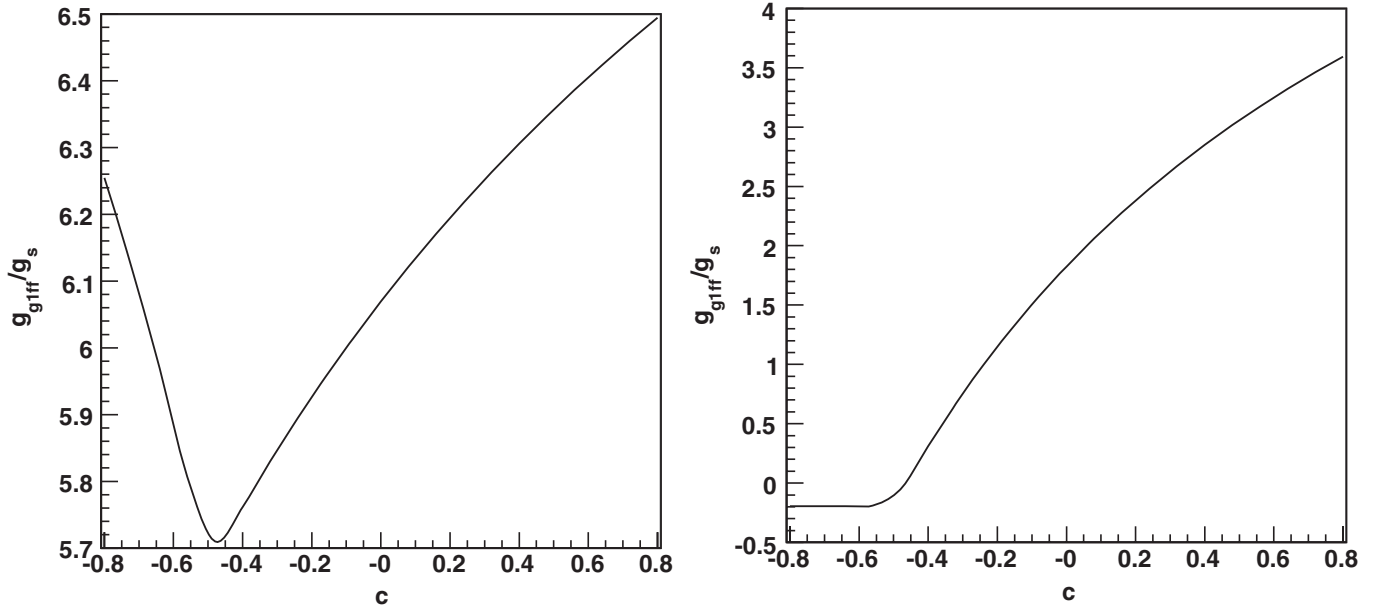
FIG. 3. Coupling of the first KK mode of the gluon to the light KK modes of the custodial partners of the right-handed up-type quark as a function of the bulk mass parameter c . The left panel shows the left-handed coupling whereas the right panel the right-handed coupling.
