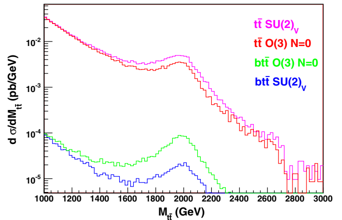
FIG. 6 (color online). Invariant mass distribution of t\bar{t} in the standard RS model [ SU(2)_V custodial symmetry] and the model with a larger O(3) custodial symmetry in pp \rightarrow t\bar{t} and pp \rightarrow bt\bar{t} , respectively.
