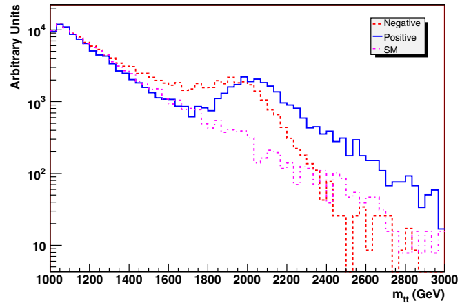
FIG. 10 (color online). Invariant mass distribution of pp \rightarrow t\bar{t} in models with positive and negative coupling to light fermions, along with the SM prediction.
