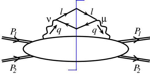
FIG. 1 (color online). Diagrammatic representation of hadronic dilepton production via a virtual photon of four-momentum q .
