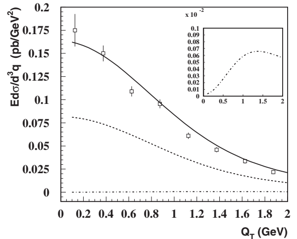
FIG. 4. The transverse momentum dependence of the angular-integrated Drell-Yan cross section, obtained from the contributions of the helicity structure functions, W_T and W_L , in Eq. (53), is shown as a solid line and compared with data from Fermilab experiment E772 [36] for Q in the interval (8,9) GeV. The dashed and dot-dashed curves show our calculations for the contributions from W_T and W_L . The inset shows the W_L contribution on an expanded scale.
