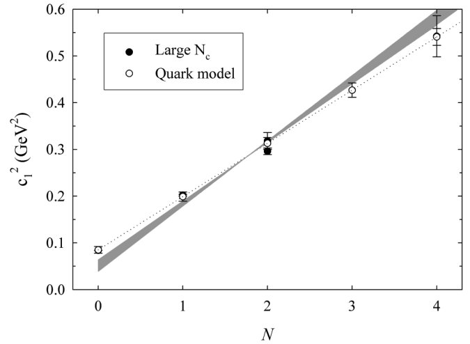
FIG. 1. Values of c_1^2 computed in the 1/N_c expansion (full circles) from a fit to experimental data (Eq. (7) for N = 0 , Refs. [21,23] for N = 1 , Ref. [24] for N = 2 and Ref. [26] for N = 4 ), compared with results from a fit (see text) of the formula (29) (empty circles and dotted line to guide the eyes). No data is available for N = 3 in large N_c studies. Values of c_1^2 as predicted by formula (29) for \sigma \in [0.17, 0.20] GeV 2 are located in the shaded area.
