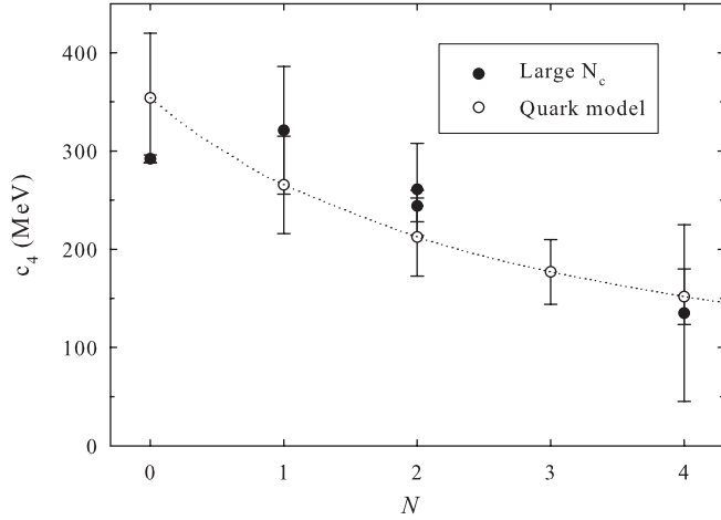
FIG. 3. Values of c_4 computed in the 1/N_c expansion (full circles) from a fit to experimental data (Eq. (7) for N = 0 , Refs. [21,23] for N = 1 , Ref. [24] for N = 2 and Ref. [26] for N = 4 ), compared with results from formula (31) (empty circles and dotted line to guide the eyes). No data is available for N = 3 in large N_c studies.
