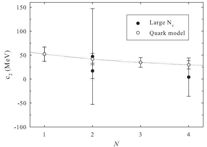
FIG. 2. Values of c_2 computed in the 1/N_c expansion (full circles) from a fit to experimental data (Refs. [21,23] for N = 1 , Ref. [24] for N = 2 and Ref. [26] for N = 4 ), compared with results from formula (31) (empty circles and dotted line to guide the eyes). No data is available for N = 3 in large N_c studies.
