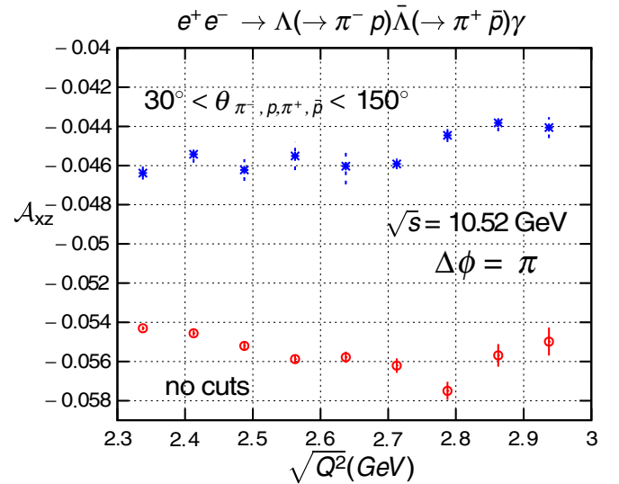
FIG. 4 (color online). The asymmetry \mathcal{A}_{xz} (see Eq. (20) for definition) for the maximal relative phase ( \Delta\phi = \pi ) between the G_M and G_E form factors.
