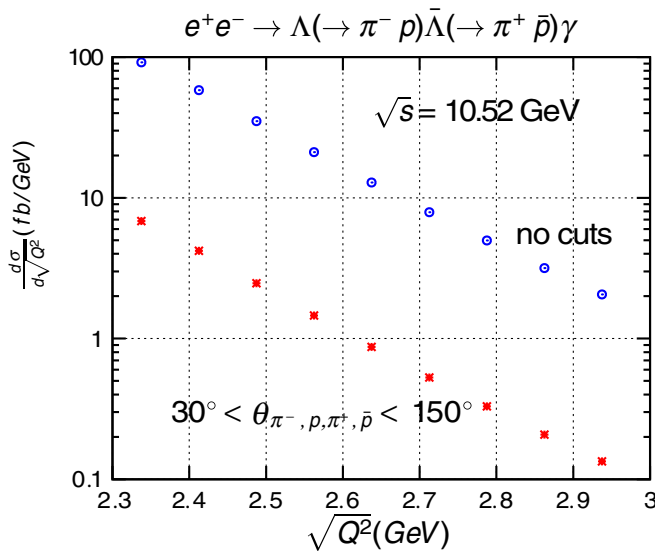
FIG. 2 (color online). The predicted differential cross section of the reaction e^+e^- \rightarrow \Lambda(\rightarrow \pi^- p)\bar{\Lambda}(\rightarrow \pi^+ \bar{p})\gamma .
