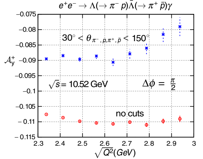
FIG. 3 (color online). The asymmetry \mathcal{A}_y^+ (see Eq. (19) for definition) for the maximal relative phase ( \Delta\phi = \pi/2 ) between the G_M and G_E form factors.
