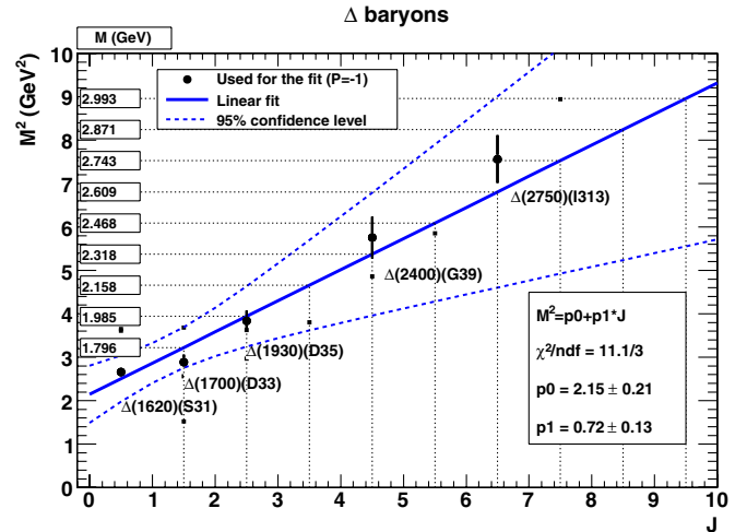
FIG. 5 (color online). As Fig. 2, but the fit was performed for the lowest-mass \Delta baryons with P = -1 .
