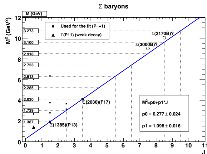
FIG. 4 (color online). The (J, M^2) plane for \Sigma baryons. The filled circles show the \Sigma baryons with P = +1 . The filled triangle shows the lowest-mass weakly-decaying \Sigma with P = +1 , while the small filled squares show all other PDG \Sigma baryons. The open circles indicate possible locations of several high-mass PDG baryons with unknown J .
