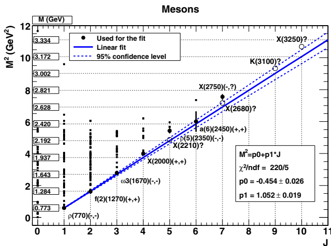
FIG. 8 (color online). The (J, M^2) plane for mesons. The filled circles show the mesons with smallest masses and J \geq 1 used for a weighted-least squares linear regression (the solid line). The dashed lines indicate a 95% confidence-level interval for the linear regression. For each meson used in the fit, space parity ( P ) and charge conjugation parity ( C ) are indicated in parentheses. Small filled squares show all other PDG mesons and the open circles indicate guessed location of several high-mass mesons with unknown J .
