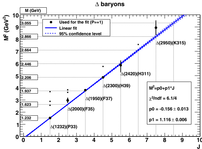
FIG. 2 (color online). The (J, M^2) plane for \Delta baryons with P = +1 . The filled circles show lowest-mass \Delta baryons used for the linear weighted-least squares regression. The solid line shows the fit, while the dashed line indicates a 95% confidence-level interval. Small filled squares show all other \Delta baryons.
