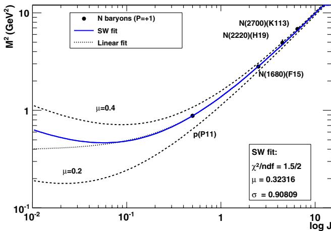
FIG. 6 (color online). The fit results for leading and daughter nucleons with positive parity. Only baryons with the minimum-mass requirement for a given J were used. The solid line indicated the fit by using Eq. (4) (the so-called SW fit) with two free parameters, \mu and \sigma . The parameter uncertainties are negligible (not shown). In order to illustrate the fit sensitivity to \mu , the dashed lines show the same fit function but with different \mu . The dotted line shows the linear fit shown in Fig. 1.
