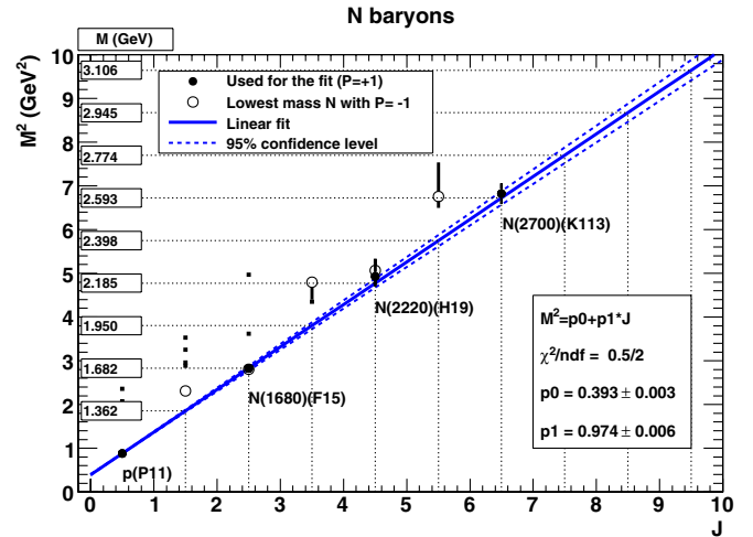
FIG. 1 (color online). The (J, M^2) plane for N -baryons. The linear fit was performed using the P = +1 baryons with smallest masses for a given J . The solid line shows the weighted-least squares regression using a linear model and the dashed lines show the corresponding 95% confidence-level interval. The open symbols show lowest-mass baryons with P = -1 : N(1520) \times (D13) (with J = 3/2 ), N(1675)(D15) (with J = 5/2 ), N(2190)(G17) (with J = 7/2 ), N(2250)(G19) (with J = 9/2 ) and N(2600)(I111) (with J = 13/2 ). The N(1675)(D15) state overlaps in mass with the N(1680)(F15) baryon with positive parity.
