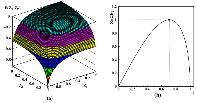
FIG. 9 (color online). F(Z_1, Z_2) as a function of Z_1 and Z_2 (left) and Z_n shown as a function of the (di)quark velocity (right).
