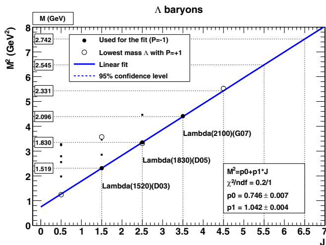
FIG. 3 (color online). The (J, M^2) plane for \Lambda baryons with P = -1 (filled symbols) and P = +1 (open symbols). The latter hadrons correspond to \Lambda(1115)(P01) , \Lambda(1820)(F05) , \Lambda(1890)(P03) and \Lambda(2350)(H09) . The \Lambda(1820)(F05) baryon with P = +1 is on top of \Lambda(1830)(D05) with P = -1 . Small filled squares show all other PDG \Lambda baryons.
