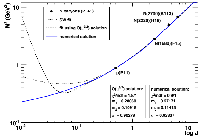
FIG. 7 (color online). The dotted line shows the SW fit as in Fig. 6. The dashed line shows the fit using the solution of the diquark string model calculated up to \mathcal{O}(\mu^{5/2}) terms, see Eq. (B10) of Appendix B. The fit was performed using two mass parameters, m_1 and m_2 ( m_1 > m_2 ) and a string tension \sigma . The solid line shows the fit using the exact numerical solution (see the text). The parameter uncertainties are negligible. Table II gives more exact numbers from the fits.
