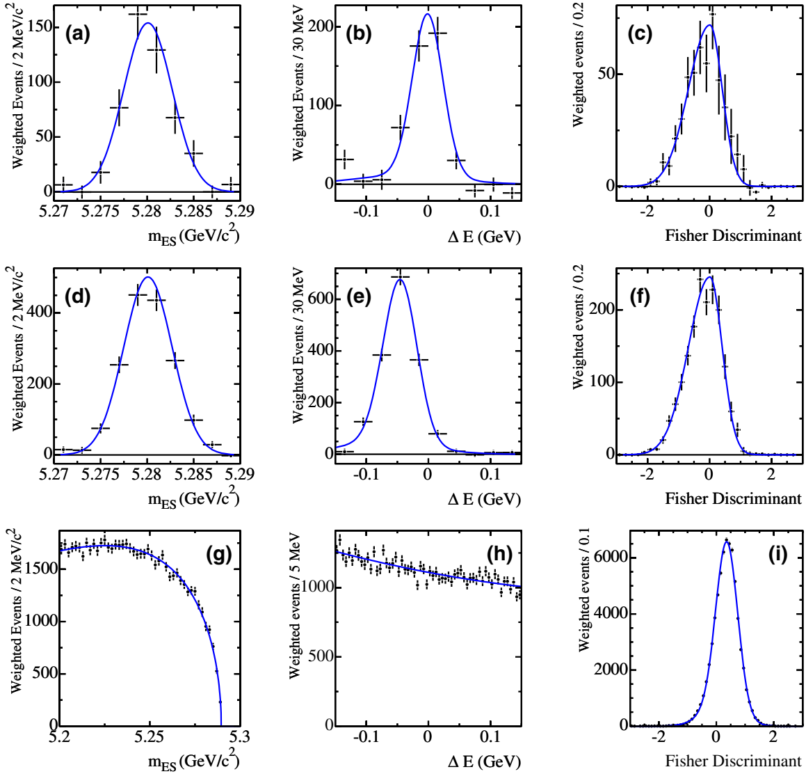
FIG. 1 (color online). Data distributions (points with error bars) of m_{ES} , \Delta E , and \mathcal{F} for signal \pi^+\pi^- (a,b,c), signal K^+\pi^- (d,e,f) and background for the three channels (g,h,i), using the weighting technique described in the text. Solid curves represent the corresponding PDFs used in the fit. The distribution of \Delta E for signal K^+\pi^- events is shifted due to the assignment of the pion mass for all tracks.
