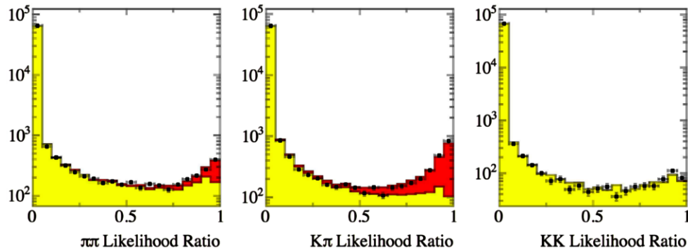
FIG. 2 (color online). (Color online) Distribution of the likelihood ratio \mathcal{L}_S / \sum \mathcal{L}_i , where \mathcal{L}_S is the likelihood for each event to be a signal \pi^+\pi^- (left), K^+\pi^- (middle), or K^+K^- (right) event. The points with error bars show the distribution obtained on the fitted data sample, while the histograms show the distributions obtained by generating signal (dark shaded, red) and background (light shaded, yellow) events directly from the PDFs.
