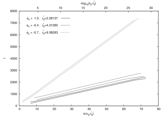
FIG. 3. The oscillon lifetime, \tau , versus -\ln|r_0 - r_0^*| is shown for states close to 3 different resonances. The lower lines plotted with a given line type represent subcritical, r_0 < r_0^* , states while the upper lines with the same line type correspond to supercritical, r_0 > r_0^* , solutions.
