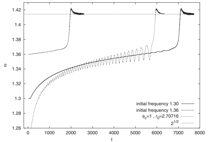
FIG. 32. Time evolution of the frequency of the oscillation of \phi at r = 0 for the three kinds of evolution simulations shown on the previous figure.
