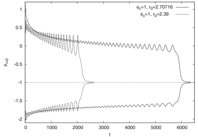
FIG. 1. The upper and lower envelope of the oscillations of the field \phi(r = 0) is shown for the evolution of Gaussian initial data of the type (12) with two different sets of initial parameters. It is important to note that the field \phi oscillates with a nonconstant period 4.6 < T < 5 . For generic oscillons the period T shows a decreasing tendency towards T \approx 4.6 .
