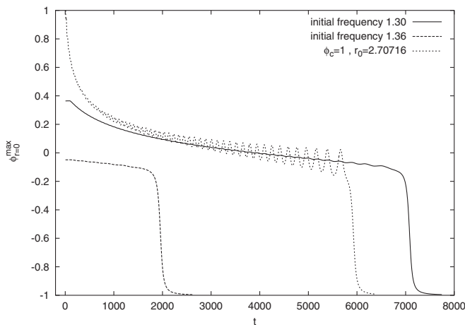
FIG. 31. Time evolution of the upper envelope curve of the oscillation of \phi at r = 0 generated by three different initial data. The first two initial data are provided with the mode decomposition method, solving the system (17) by choosing the frequencies \omega = 1.30 and \omega = 1.36 . The third evolution corresponds to Gaussian-type initial data (12) with \phi_c = 1 and r_0 = 2.70716 .
