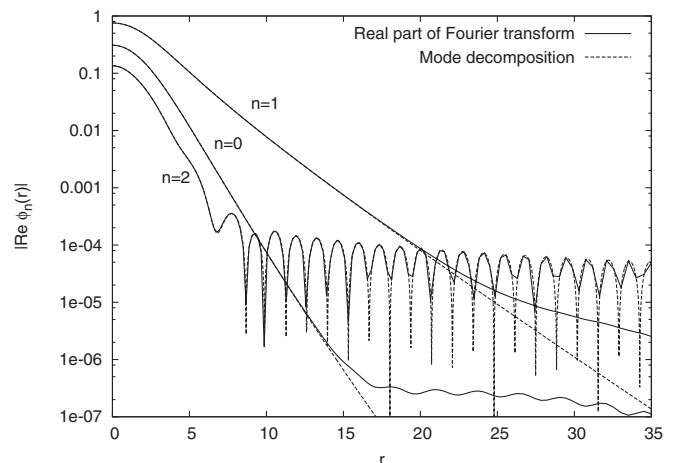
FIG. 33. Fourier decomposition of the evolution of the \omega = 1.3 initial data close to the moment of time when its frequency increases to 1.36. The results are compared to the modes of the periodic solution obtained by the mode decomposition method for the \omega = 1.36 frequency.
