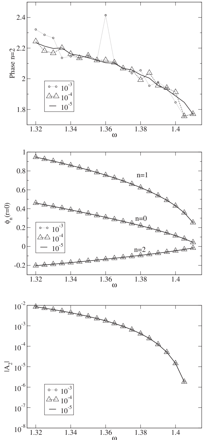
FIG. 8. Convergence of the various results with respect to the precision required when finding the minimum of |A_2| .
