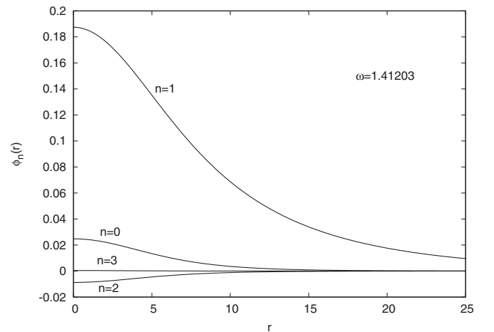
FIG. 7. Radial dependence of Fourier modes obtained by decomposition of a near-periodic state with frequency \omega = 1.41203 .
