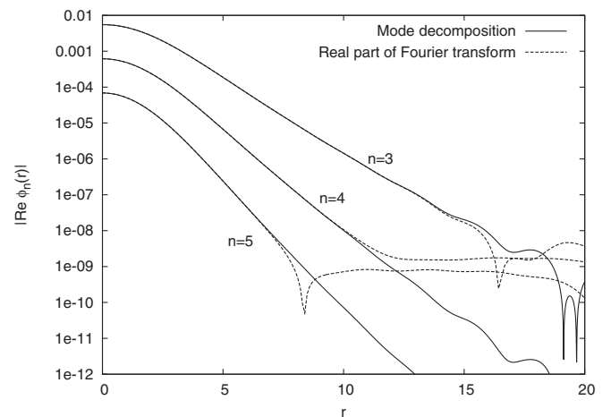
FIG. 20. Comparison of the higher modes of the two systems presented on the previous figure.
