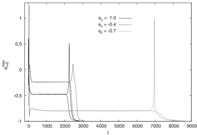
FIG. 4. Upper envelopes of the oscillations of the field value at r = 0 for three pairs of subcritical and supercritical oscillon states close to the first resonances corresponding to three given \phi_c initial parameters. The fine-tuning was performed using 32 digit arithmetics.
