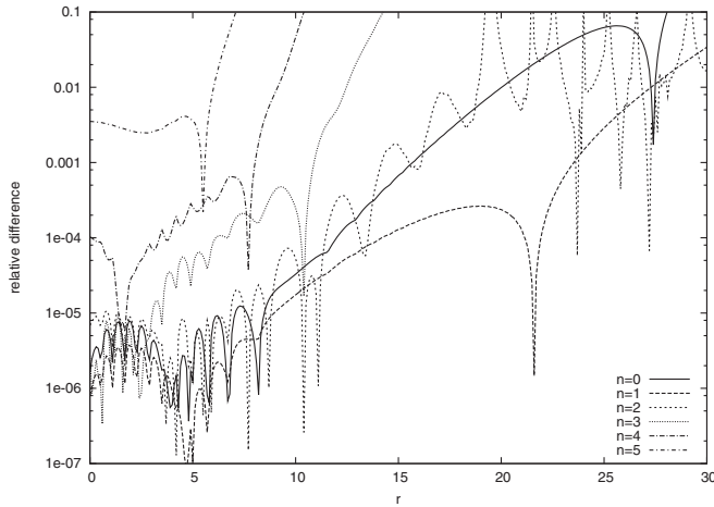
FIG. 21. Dependence on the radius r of the relative difference of the modes coming from the mode decomposition and the Fourier transformation for \omega = 1.398\,665 . The relative difference is defined as the absolute value of the ratio of the difference and the mode decomposition value.
