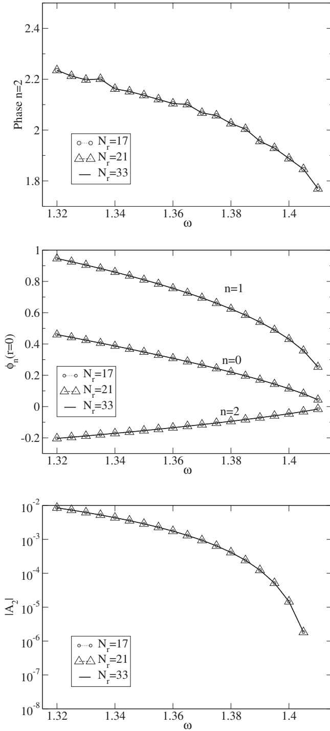
FIG. 10. Same as Fig. 8 but when varying the N_r in each domain.
