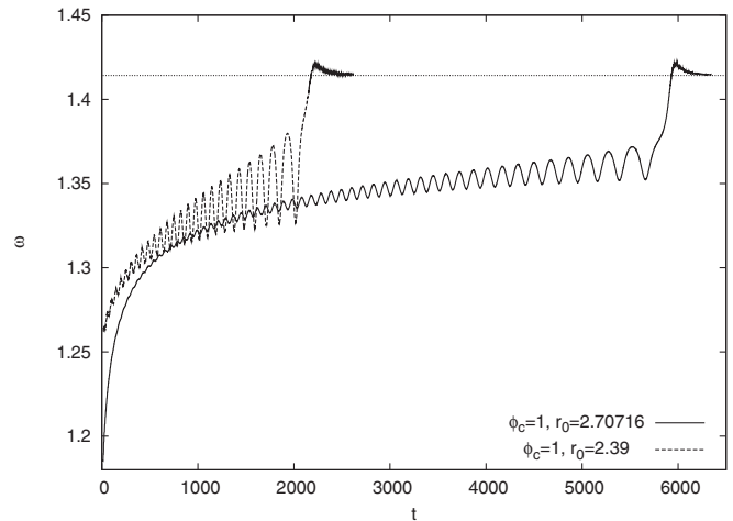
FIG. 23. Time evolution of the underlying high frequency oscillation of the oscillon state of Fig. 1 is presented.
