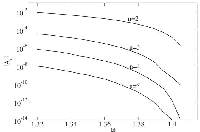
FIG. 14. Coefficients of the oscillatory homogeneous solutions \phi_n ( n = 2, 3, 4, 5 ) as a function of \omega .
