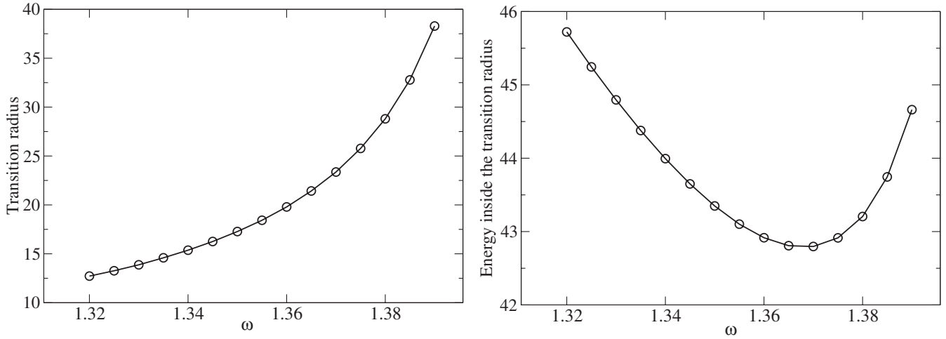
FIG. 17. The transition radius between the exponential decay and the oscillatory tail (left panel) and the energy inside this radius (right panel), as a function of \omega .
