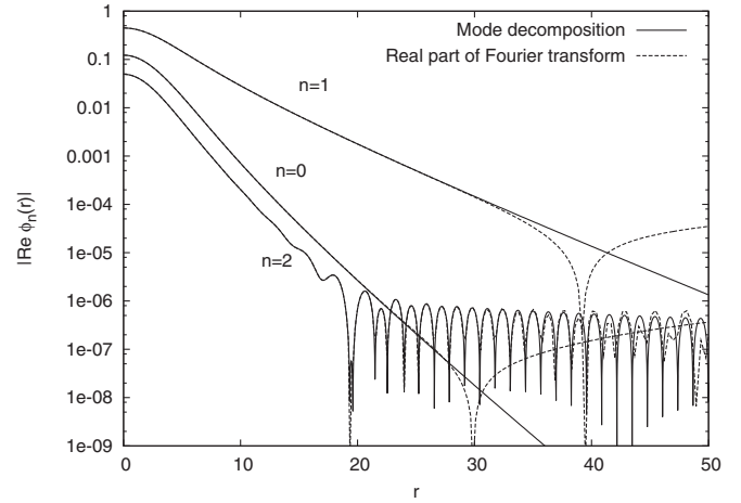
FIG. 19. Comparison between the modes coming from solving the system (17) directly and the real part of the modes obtained by performing a Fourier transform of the evolution for \omega = 1.398665 . In order to be able to represent on the same graph the large values in the central oscillon region along with the small tails at high radii, the absolute values are plotted logarithmically. We note that the central value \phi_n(0) is positive for n = 0 and for odd n while it is negative for other n . The peaks pointing downwards on the figure correspond to places where the functions change signature.
