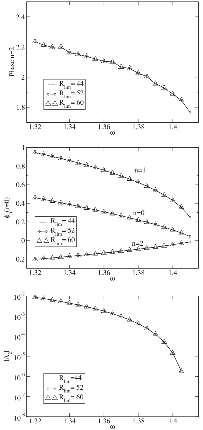
FIG. 11. Same as Fig. 8 but changing the value of R_{lim} .
