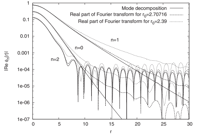
FIG. 26. The modes of the periodic solution with frequency 1.36 is compared with the Fourier decomposition of two different oscillon states. The first oscillon state with initial data \phi_c = 1 , r_0 = 2.70716 is decomposed between the two subsequent maxima after t = 4158.76 , where the calculated frequency is 1.3596. The second state with \phi_c = 1 , r_0 = 2.39 is decomposed just after t = 1526.58 , where the frequency is 1.3613.
