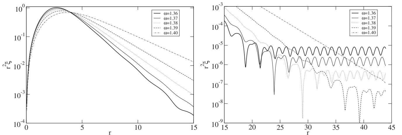
FIG. 16. Same as Fig. 15 but with the volume element included: r^2\xi .
