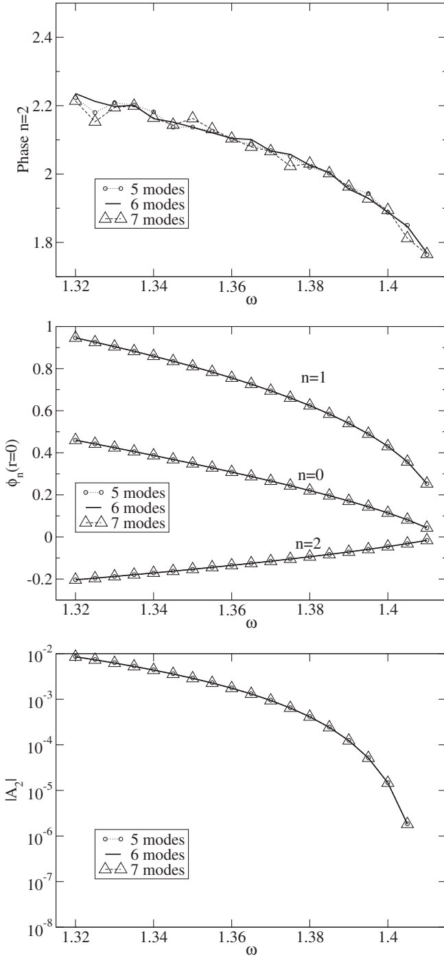
FIG. 12. Same as Fig. 8 but varying the number of modes.
