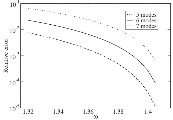
FIG. 13. Relative difference between the lhs and rhs members of Eq. (3). The result is averaged over one period and we present the error as a function of \omega , for 5, 6, and 7 modes.
