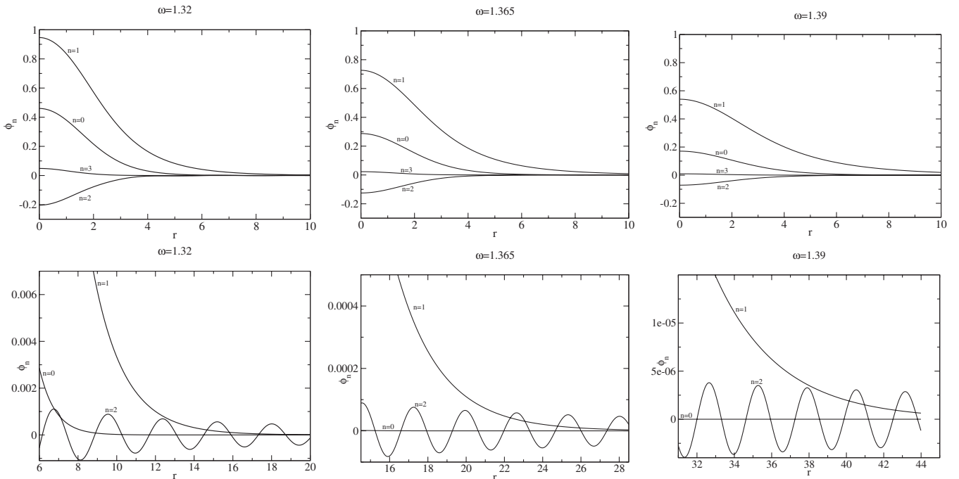
FIG. 18. The first modes near the origin and in the transition region for \omega = 1.32, 1.365, and 1.39 .
