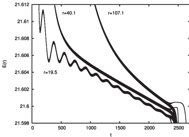
FIG. 6. The time dependence of the energy contained in spheres of radii r = 19.5 , r = 40.1 , and r = 107.1 for the \phi_c = -0.4 first peak. The thickness of the curve indicates that the high frequency oscillation is still not negligible at these high radii. The different endings of the curves correspond to subcritical and supercritical states.
