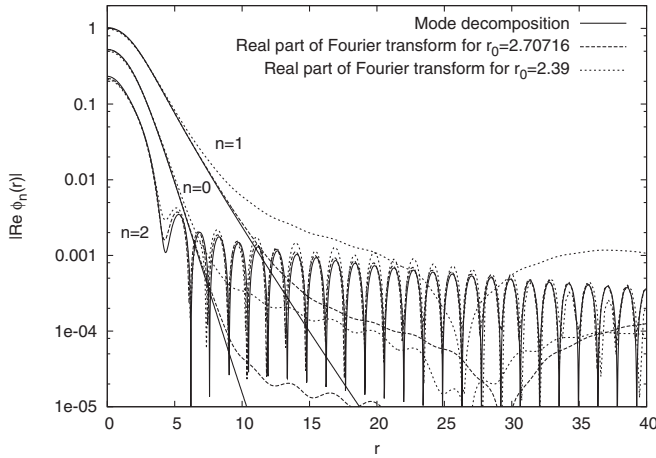
FIG. 24. The modes of the periodic solution with frequency 1.3 are compared with the Fourier decomposition of two different oscillon states. The first oscillon state with initial data \phi_c = 1 , r_0 = 2.70716 is decomposed between the two subsequent maxima after t = 471.47 , where the calculated frequency is 1.2995. The second state with \phi_c = 1 , r_0 = 2.39 is decomposed just after t = 298.72 , where the frequency is 1.3011.
