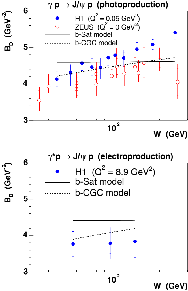
FIG. 21 (color online). The t -slope parameter B_D vs W compared to predictions from the b-Sat and b-CGC models using the “boosted Gaussian” vector meson wave function.
