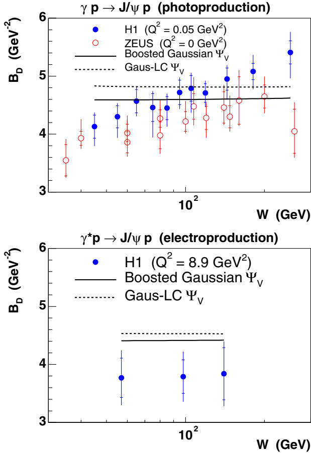
FIG. 18 (color online). The t -slope parameter B_D vs W , where B_D is defined by fitting d\sigma/dt \propto \exp(-B_D|t|) , compared to predictions from the b-Sat model using two different vector meson wave functions.
