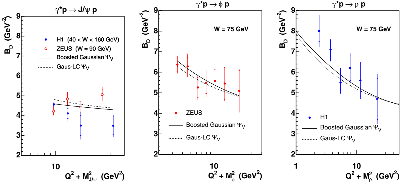
FIG. 14 (color online). The t -slope parameter B_D vs (Q^2 + M_V^2) , where B_D is defined by fitting d\sigma/dt \propto \exp(-B_D|t|) , compared to predictions from the b-Sat model using two different vector meson wave functions.
