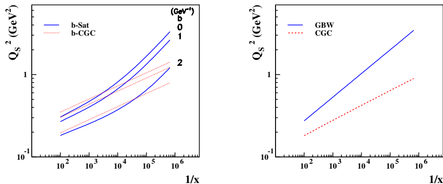
FIG. 22 (color online). The saturation scale Q_S^2 \equiv 2/r_S^2 , where r_S is defined as the solution of (54), found in the b-Sat and b-CGC models (left), and in the GBW and CGC models (right).
