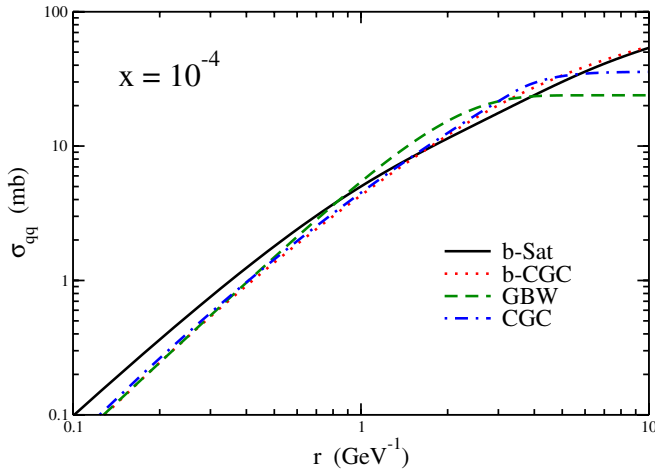
FIG. 27 (color online). The dipole cross section \sigma_{q\bar{q}}(x, r) at fixed x = 10^{-4} , integrated over the impact parameter \mathbf{b} , obtained in the b-Sat, b-CGC, GBW, and CGC models.
