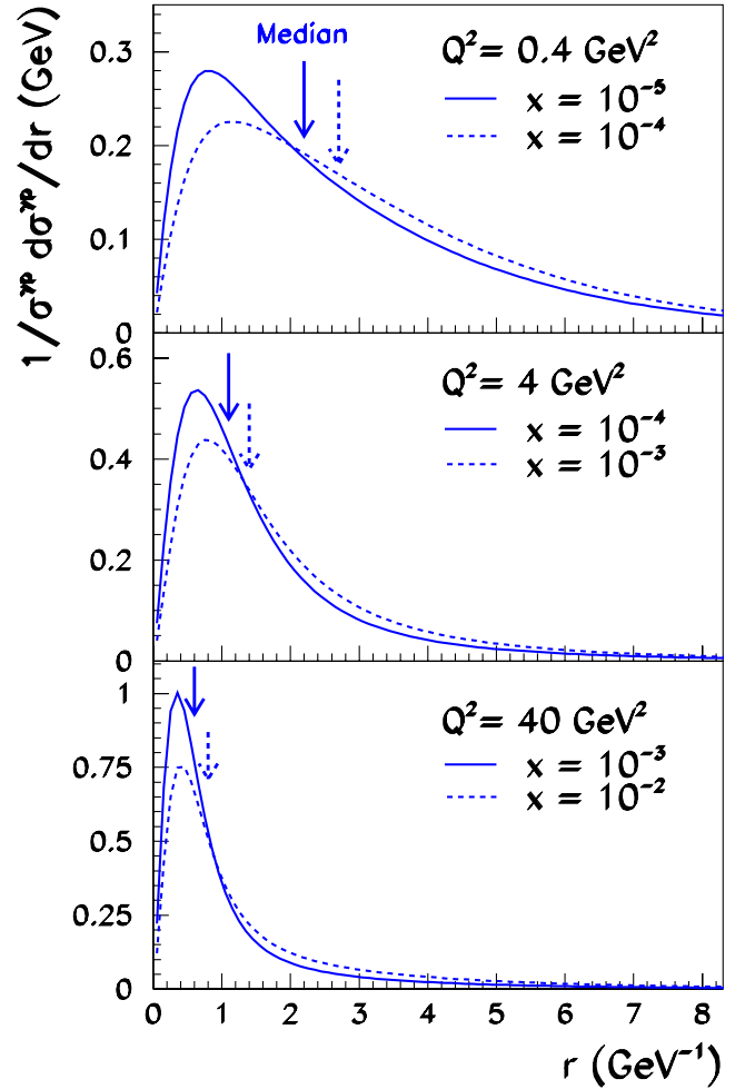
FIG. 28 (color online). The distribution of dipole sizes r contributing to the total inclusive DIS cross section in the b-Sat model for various virtualities, Q^2 , of the photon. The median values are indicated by vertical arrows.
