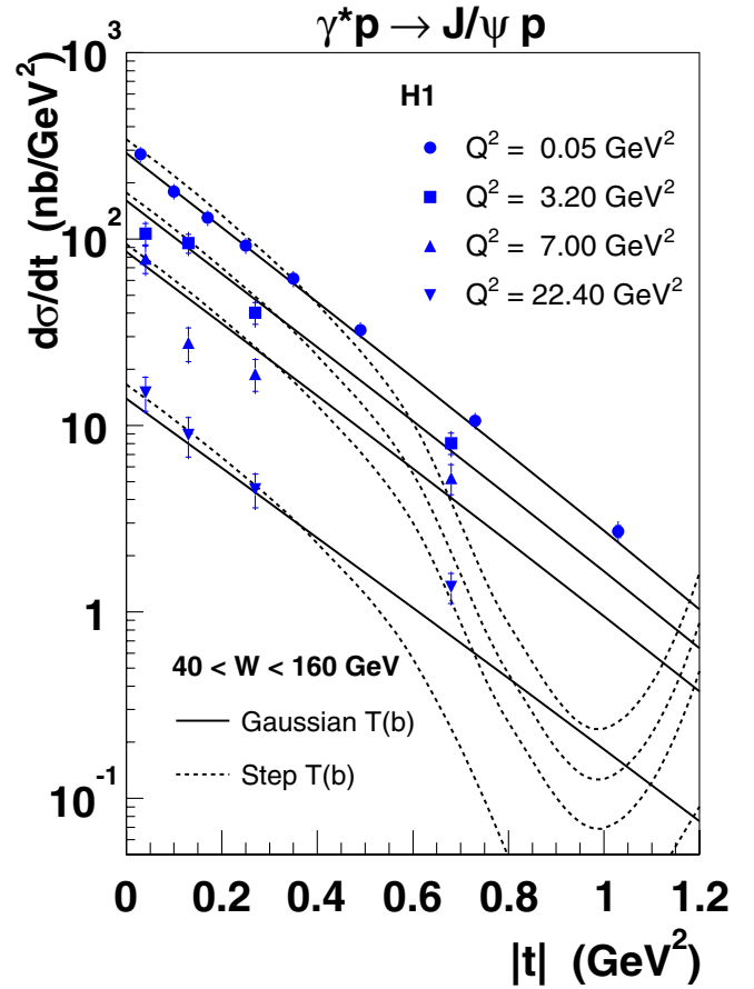
FIG. 25 (color online). Differential J/\psi meson cross section d\sigma/dt vs |t| compared to predictions from the b-Sat model using the “boosted Gaussian” vector meson wave function with either a Gaussian or a step T(b) .
