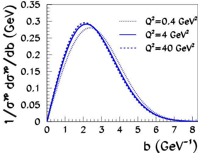
FIG. 23 (color online). The b -dependence of the total cross section, \sigma_{\text{tot}}^{\gamma p} , for Q^2 = 0.4, 4 and 40 \text{ GeV}^2 with x = 10^{-4}, 10^{-3} and 10^{-2} respectively, using a Gaussian T(b) of width B_G = 4 \text{ GeV}^{-2} .
