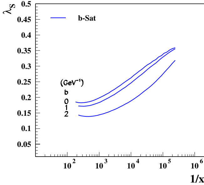
FIG. 24 (color online). The saturation exponent \lambda_S as a function of x and impact parameter b .
