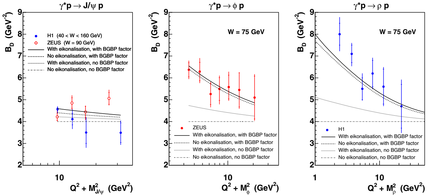
FIG. 15 (color online). The t -slope parameter B_D vs (Q^2 + M_V^2) compared to predictions from the b-Sat model using the “boosted Gaussian” vector meson wave function. We show the effect of switching off the eikonalization in the dipole cross section (41), and omitting the BGBP [40] factor, \exp[i(1-z)\mathbf{r} \cdot \mathbf{\Delta}] , in (12).
