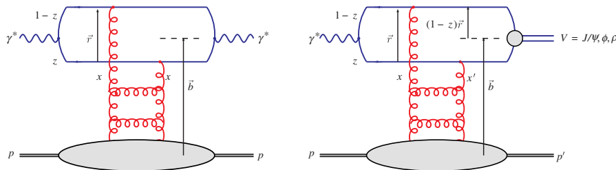
FIG. 2 (color online). The elastic scattering amplitude for inclusive DIS (left) and vector meson production (right). For DVCS, the outgoing vector meson in the right-hand diagram is replaced by a real photon.
