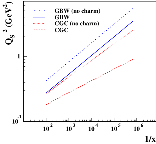
FIG. 26 (color online). The saturation scale Q_S^2 \equiv 2/r_S^2 , where r_S is defined as the solution of (54), found in the GBW and CGC models with and without charm quarks. The presence of charm quarks dramatically lowers the saturation scale, especially for the CGC model.
