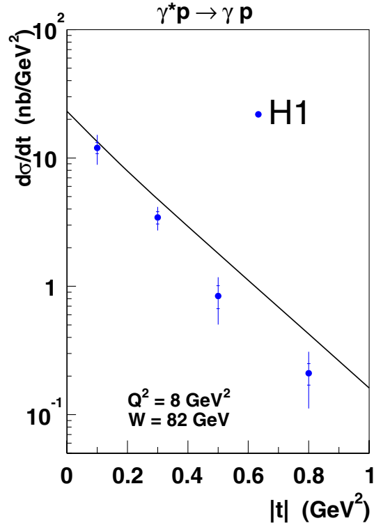
FIG. 20 (color online). Differential DVCS cross section d\sigma/dt vs |t| compared to the prediction from the b-Sat model.
