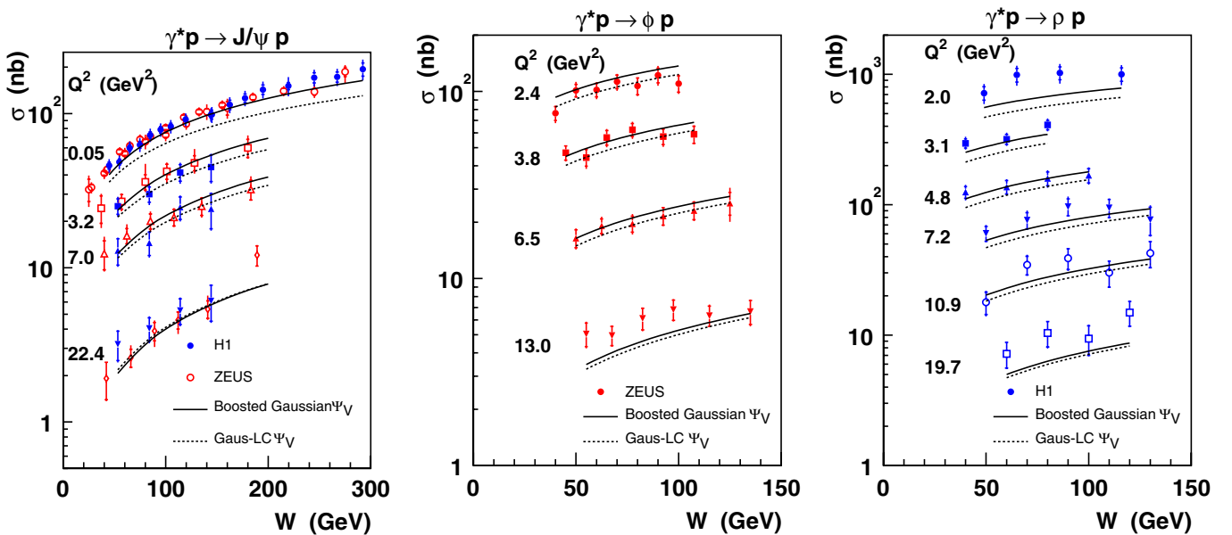
FIG. 8 (color online). Total vector meson cross section \sigma vs W compared to predictions from the b-Sat model using two different vector meson wave functions. The ZEUS J/\psi data points [25,26] have been scaled to the H1 Q^2 values [27] using the Q^2 dependence measured by ZEUS of the form \sigma \propto (Q^2 + M_V^2)^{-2.44} [26].
