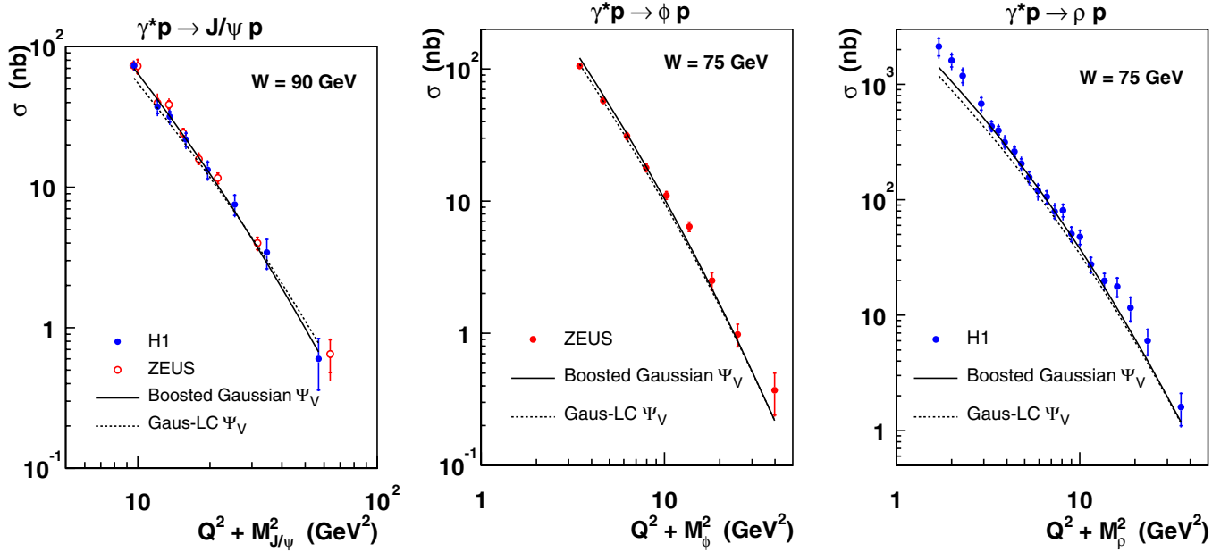
FIG. 7 (color online). Total vector meson cross section \sigma vs (Q^2 + M_V^2) compared to predictions from the b-Sat model using two different vector meson wave functions. The ZEUS J/\psi photoproduction point is taken from Table 1 of Ref. [25], from the muon decay channel with W = 90\text{--}110 \text{ GeV} .
