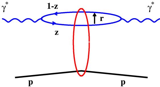
FIG. 1 (color online). The elastic scattering of a virtual photon on a proton in the dipole representation.
