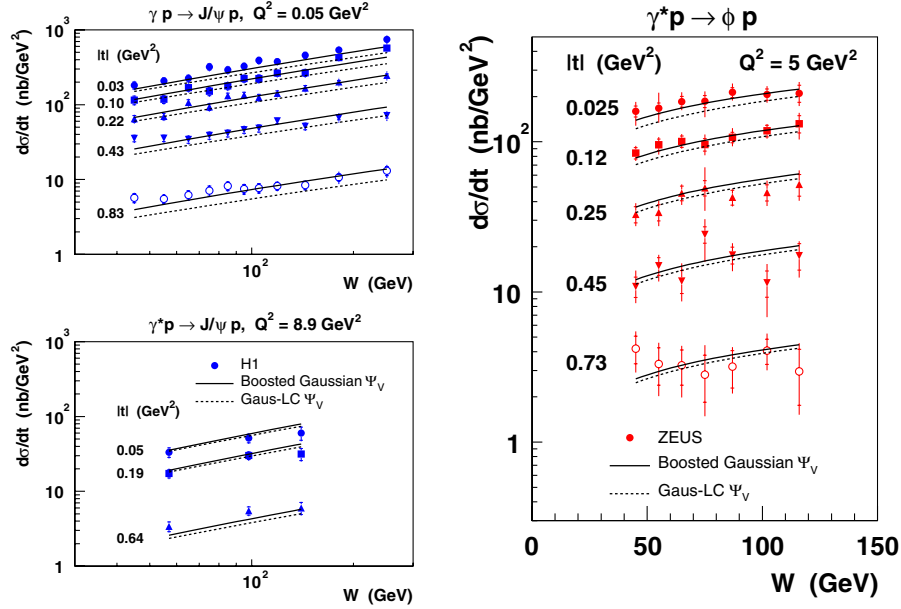
FIG. 16 (color online). Differential vector meson cross section d\sigma/dt vs W compared to predictions from the b-Sat model using two different vector meson wave functions.
