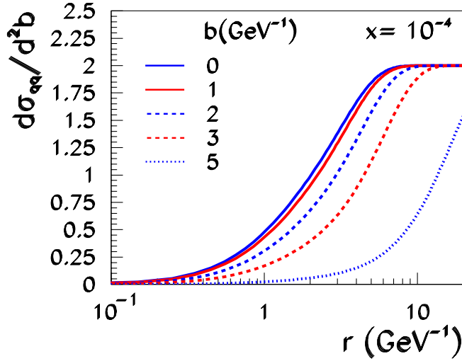
FIG. 4 (color online). Dipole cross section at various impact parameters, as determined in the b-Sat model.
