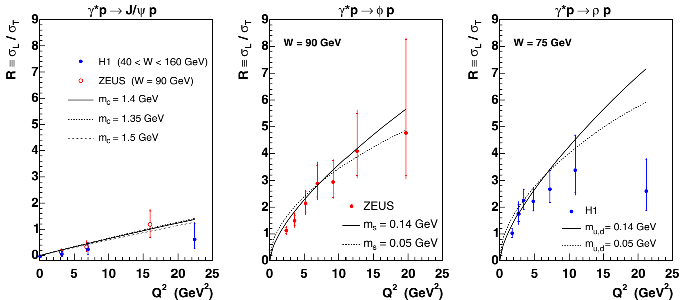
FIG. 12 (color online). The ratio R \equiv \sigma_L/\sigma_T vs Q^2 compared to predictions from the b-Sat model using the “boosted Gaussian” vector meson wave function for different quark masses.
