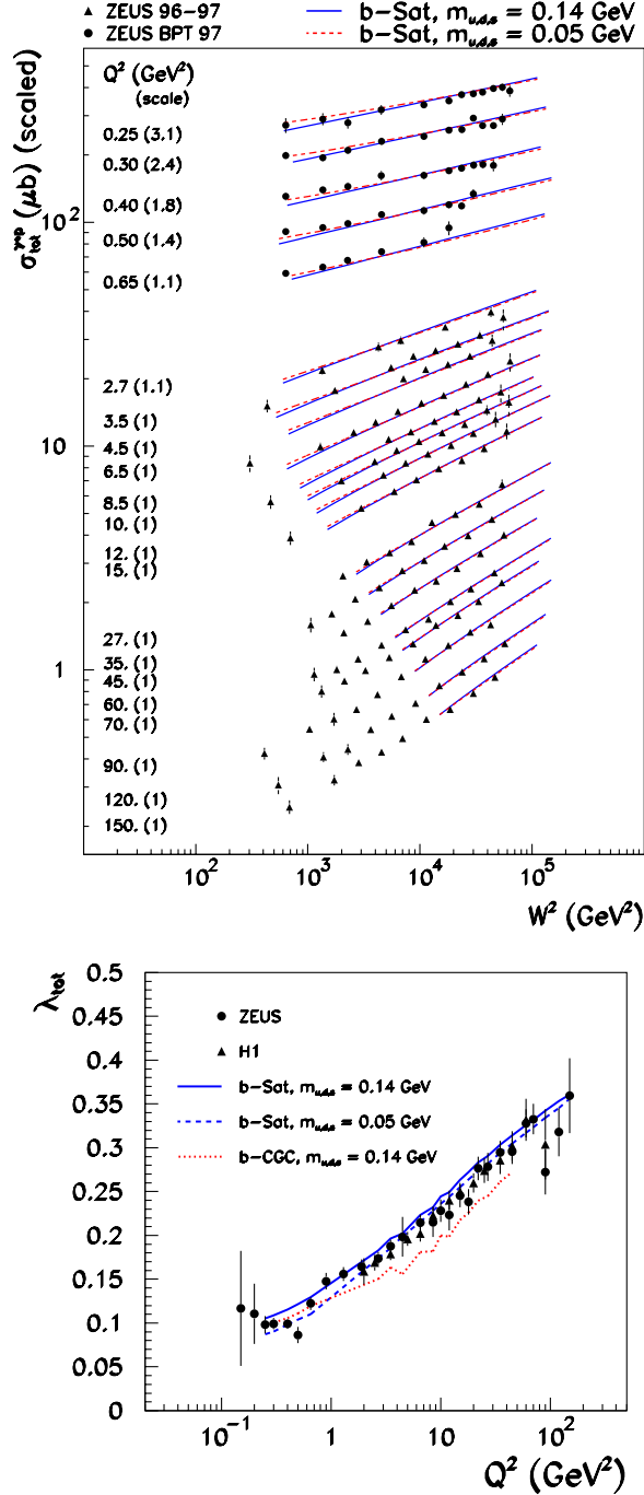
FIG. 5 (color online). Top : The total DIS cross section \sigma_{\text{tot}}^{\gamma^* p} vs W^2 for different Q^2 . The data points plotted are from ZEUS [22,23]. Bottom : The \lambda_{\text{tot}} parameter for inclusive DIS defined by \sigma_{\text{tot}}^{\gamma^* p} \propto (1/x)^{\lambda_{\text{tot}}} . The data points plotted are from ZEUS [22,23] and H1 [24].
