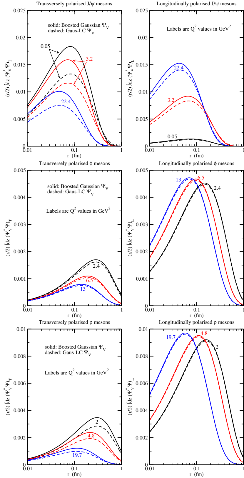
FIG. 3 (color online). Overlap functions (21) and (22) between the photon and vector meson wave functions integrated over z for the three different vector mesons at Q^2 values representative of the data.
