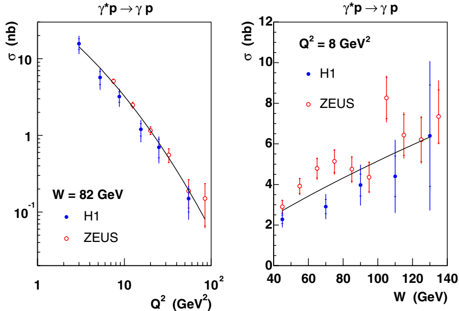
FIG. 19 (color online). Total DVCS cross sections \sigma vs Q^2 (left) and \sigma vs W (right) compared to predictions from the b-Sat model.
