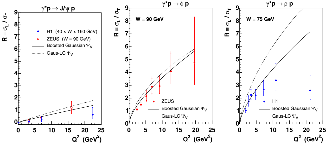
FIG. 11 (color online). The ratio R \equiv \sigma_L/\sigma_T vs Q^2 compared to predictions from the b-Sat model using two different vector meson wave functions.
