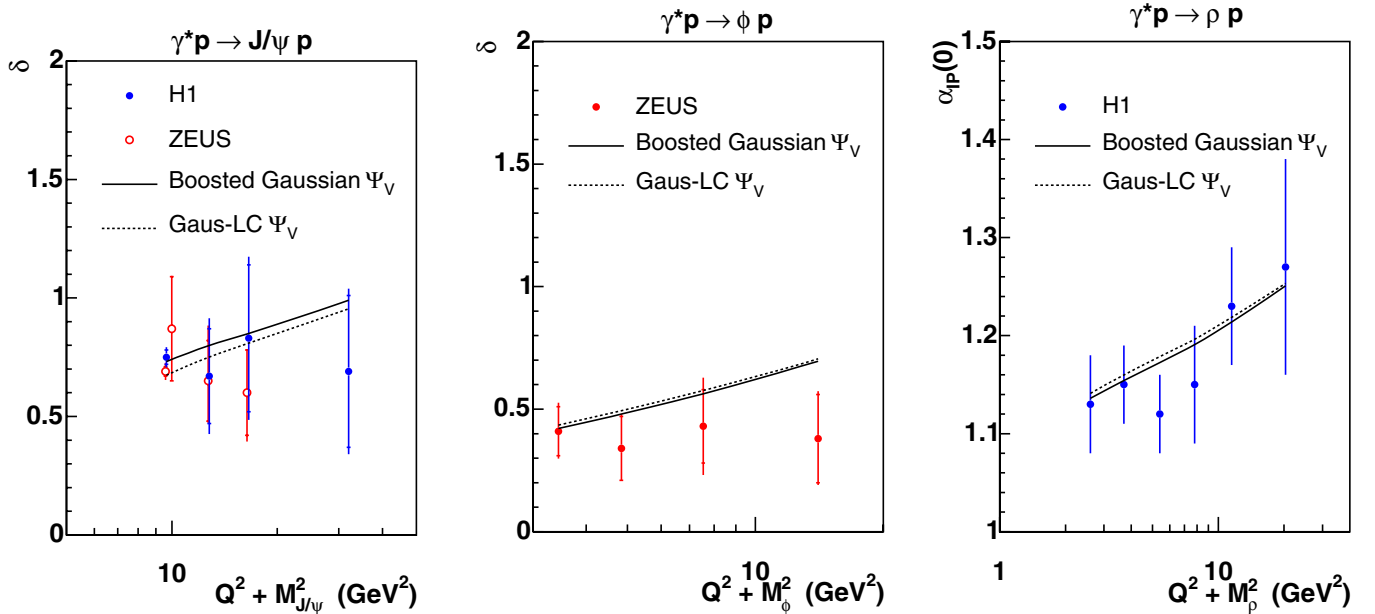
FIG. 10 (color online). The power \delta vs (Q^2 + M_V^2) , where \delta is defined by fitting \sigma \propto W^\delta , compared to predictions from the b-Sat model using two different vector meson wave functions. For \rho mesons, we instead show \alpha_\rho(0) defined in the main text; the error bars represent the statistical and noncorrelated systematic uncertainties only [29].
