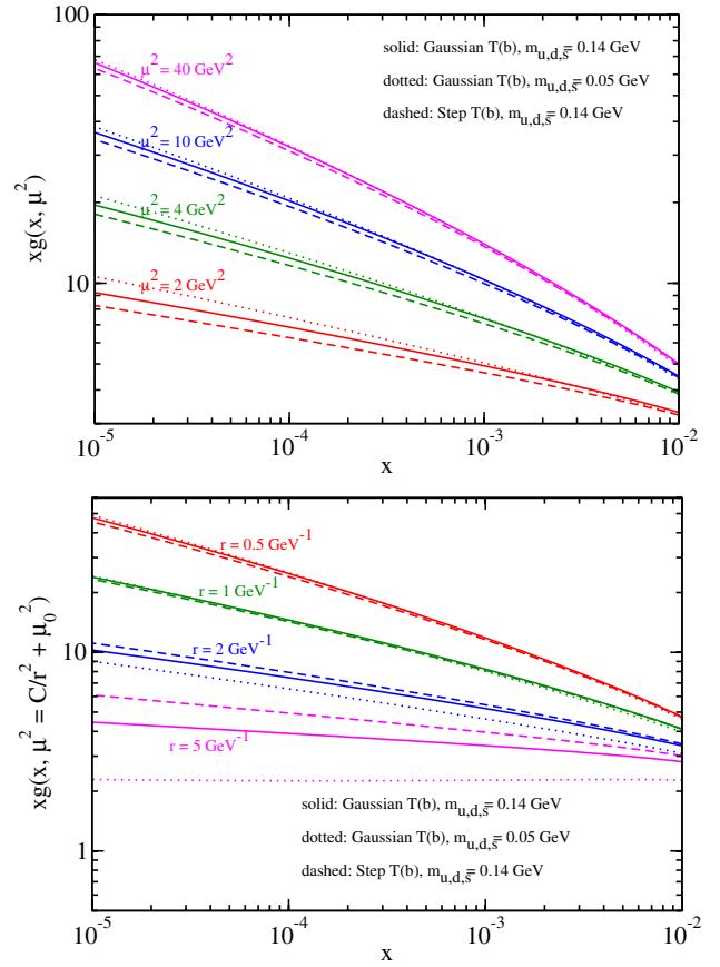
FIG. 6 (color online). The gluon distribution xg(x, \mu^2) for different fixed \mu^2 (top) or fixed r (bottom).
