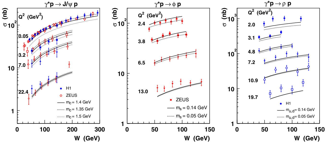
FIG. 9 (color online). Total vector meson cross section \sigma vs W compared to predictions from the b-Sat model using the “boosted Gaussian” vector meson wave function for different quark masses.
