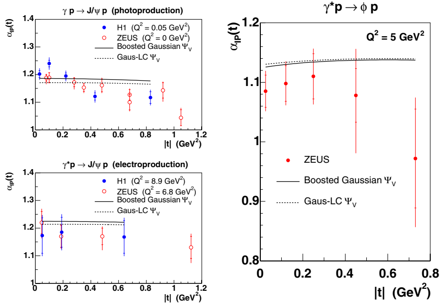
FIG. 17 (color online). The Pomeron trajectory \alpha_p(t) vs |t| , where \alpha_p(t) is determined by fitting d\sigma/dt \propto W^{4[\alpha_p(t)-1]} , compared to predictions from the b-Sat model using two different vector meson wave functions.
