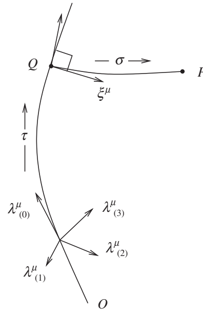
FIG. 1. Schematic construction of Fermi coordinates at P .
