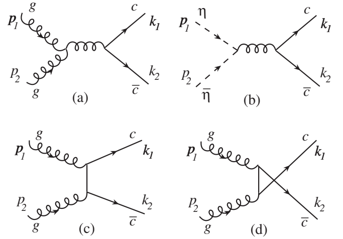
FIG. 17. (a) Gluon fusion via the s -channel into a c\bar{c} final state. (b) Ghost-antighost annihilation that cancels the contribution from the unphysical gluon polarization states in the covariant gauge. (c) t -channel and (d) the crossed u -channel charm exchange diagram.
