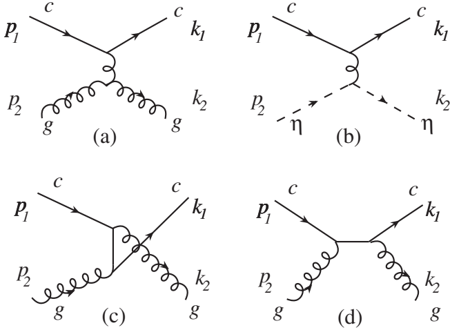
FIG. 19. (a) Charm quark on gluon scattering via t -channel gluon exchange. (b) Charm-ghost scattering that cancels the contribution from the unphysical gluon polarization states in the covariant gauge. (c) Charm quark on gluon scattering via virtual heavy quark exchange in the u -channel. (d) The corresponding s -channel diagram. Anticharm on gluon scattering is given by a similar set of diagrams.
