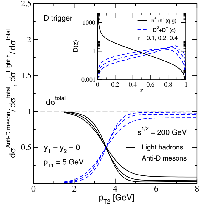
FIG. 5 (color online). Contribution of light hadrons and anti-charm mesons to the fractional production cross section for p_{T_1} = 5 GeV D^0 + D^+ meson-triggered away-side correlations for y_1 = y_2 = 0 in p + p collisions. The insert illustrates the difference in the fragmentation of light quarks and gluons into hadrons versus that for the c quark into charm mesons. Three different values for the nonperturbative fragmentation parameter r = 0.1, 0.2 and 0.4 were used.
