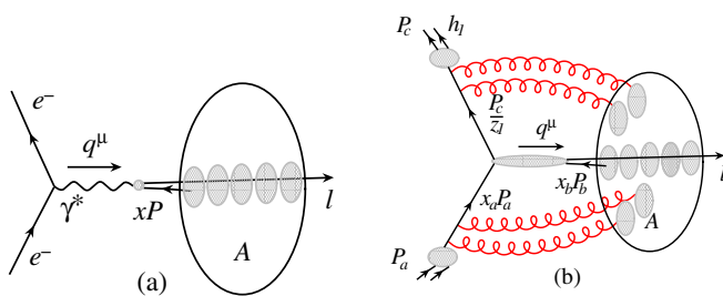
FIG. 7 (color online). Coherent multiple scattering of the struck parton in deep inelastic scattering (a) and in proton-nucleus collisions (b). Notice the difference between p + A and DIS in terms of the multiple initial- and final-state scattering of the incoming and outgoing partons (‘‘a’’ and ‘‘c’’).
