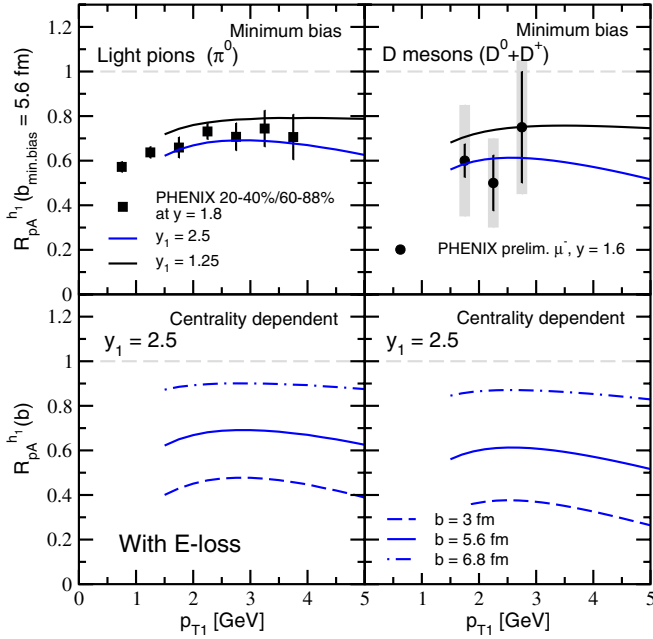
FIG. 14 (color online). Nuclear modification of single inclusive \pi^0 (left panels) and D^0 + D^+ mesons (right panels) in d + Au collisions at RHIC. The same rapidities and centralities as in Fig. 10 are shown. Energy loss is taken into account in the theoretical calculations.
