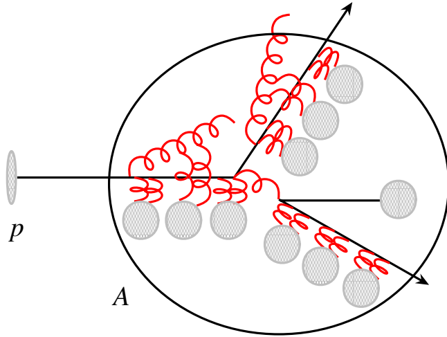
FIG. 1 (color online). Schematic representation of the initial- and final-state elastic, inelastic and coherent multiple parton scattering that give the nuclear A^{n/3} -enhanced corrections similar to Eq. (2) for proton-nucleus collisions in the nuclear rest frame.
