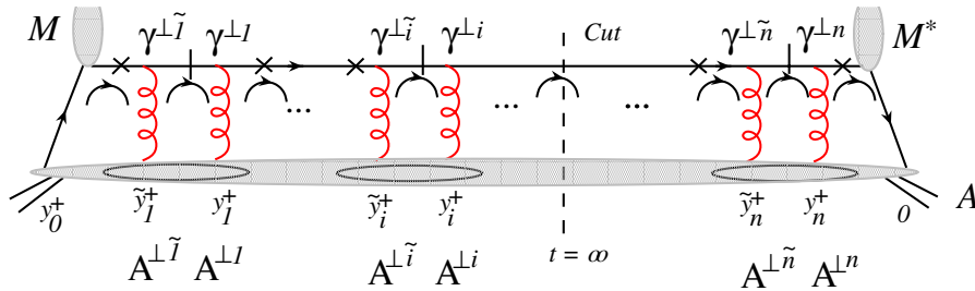
FIG. 20 (color online). Multiple coherent scattering of the outgoing partons in proton-nucleus reactions in the t -channel. We have denoted by \times \rightarrow and + \rightarrow the long distance and contact propagators, respectively. We have indicated the light cone positions, e.g. y_i^+ . Arcs show the momentum routing. Gluons are dominated by their transverse components and the fields, e.g. A^{\perp i}(y_i^+) , are shown before the conversion to the field strength tensor and before the factorization of the color and Lorentz indexes.
