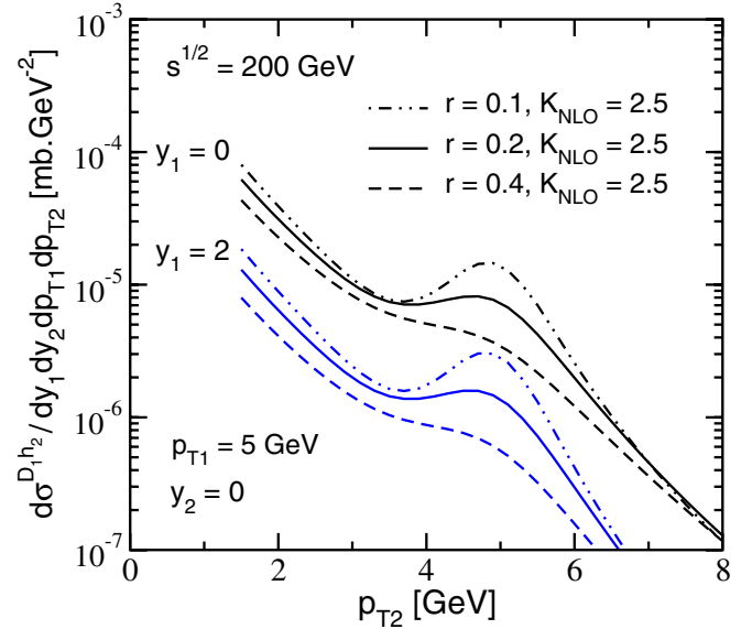
FIG. 6 (color online). The double inclusive hadron production cross section at RHIC for a D^0 + D^+ trigger at p_{T_1} = 5 GeV in p + p collisions. Three different combinations of r and K_{\text{NLO}} are studied. Two different rapidity gaps y_1 - y_2 = 0, 2 are shown for comparison. The characteristic hump represents hard \bar{c} fragmentation into \bar{D} mesons.
