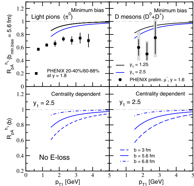
FIG. 10 (color online). Top: suppression of the single inclusive hadron production rates in d + Au reactions versus p_T for rapidities y_1 = 1.25 (smaller attenuation) and y_1 = 2.5 (larger attenuation) at \sqrt{s_{NN}} = 200 GeV. Bottom: impact parameter dependence of the calculated nuclear modification for central, b = 3 fm, minimum bias, b_{\text{min.bias}} = 5.6 fm and peripheral, b = 6.8 fm, collisions. The scale of higher twist per nucleon \xi^2 = 0.12 GeV 2 . Data is from PHENIX [17,35]. Theory does not include energy loss.
