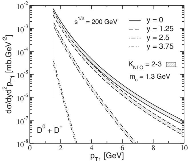
FIG. 3. The cross section for D^0 + D^+ charm meson production to LO in perturbative QCD at \sqrt{s} = 200 GeV in p + p collisions at RHIC with K_{\text{NLO}} = 2-3 and r = 0.2 . The differential cross section is shown in four rapidity bins: y = 0, 1.25, 2.5 and 3.75 .
