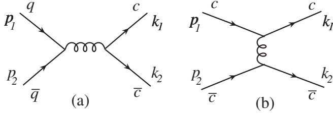
FIG. 16. (a) Light quark-antiquark annihilation into a massive c\bar{c} final state. (b) t -channel scattering contribution for the case of non-negligible initial (anti)charm parton distributions. Note that for c\bar{c} \rightarrow c\bar{c} both diagrams contribute. Time increases from left to right in all diagrams and arrows indicate momentum flow.
