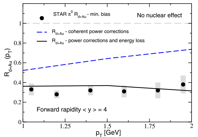
FIG. 12 (color online). Suppression of \pi^0 production at y = 4 for d + Au collisions at \sqrt{s_{NN}} = 200 \text{ GeV} at RHIC [18]. Calculations of dynamical shadowing with and without cold nuclear matter energy loss are shown.
