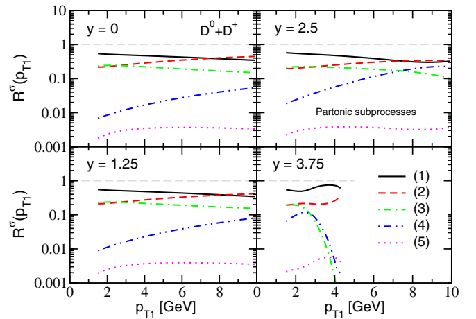
FIG. 4 (color online). Fractional contribution of partonic subprocesses ( i ) to moderate and high p_{T_1} D^0 + D^+ meson production in \sqrt{s} = 200 GeV p + p collisions at rapidities y = 0, 1.25, 2.5 and 3.75 . We considered (1) cg \rightarrow cg (solid line), (2) cq(\bar{q}) \rightarrow cq(\bar{q}) (dashed line), (3) gg \rightarrow c\bar{c} (dot-dashed line), (4) q\bar{q} \rightarrow c\bar{c} (double dot-dashed line) and (5) c\bar{c} \rightarrow c\bar{c} (dotted line). Note the dominance (except at the highest values of p_{T_1} ) of the cg \rightarrow cg channel.
