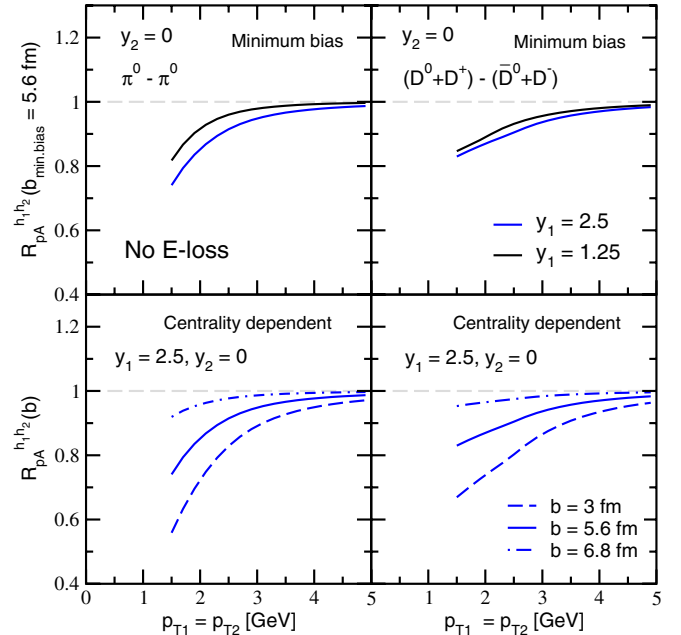
FIG. 11 (color online). Top: suppression of double inclusive hadron production rates in d + Au reactions versus p_T for trigger and associated hadrons of the same transverse momentum but different rapidities: y_1 = 1.25 (smaller attenuation) and y_1 = 2.5 (larger attenuation) for the trigger and y_2 = 0 for the associated hadron. Bottom: impact parameter dependence of the calculated nuclear modification for central, b = 3 fm, minimum bias, b_{\text{min.bias}} = 5.6 fm and peripheral, b = 6.8 fm, collisions. The scale of higher twist per nucleon \xi^2 = 0.12 GeV 2 . Theory does not include energy loss.
