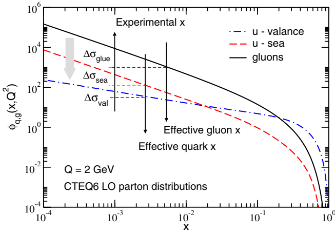
FIG. 8 (color online). Effects of rescaling of the momentum fraction x are illustrated using as an example the lowest order CTEQ6 parton distribution functions for valence and sea u -quarks. Gluons rescatter in the final-state to lowest order only in hadronic collisions and are included for completeness. The effective parton distributions or partonic flux are reduced after the rescaling of the momentum fraction. We used Q^2 = 4 \text{ GeV}^2 and the large rescaling in x is for purposes of illustration only.
