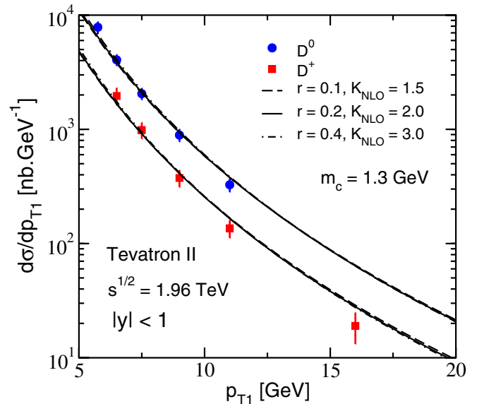
FIG. 2 (color online). Cross section for D^0 and D^+ charm meson production to LO in perturbative QCD at \sqrt{s} = 1.96 TeV. Three approximately equivalent pairs of a phenomenological K -factor and the D meson fragmentation parameter r are shown.
