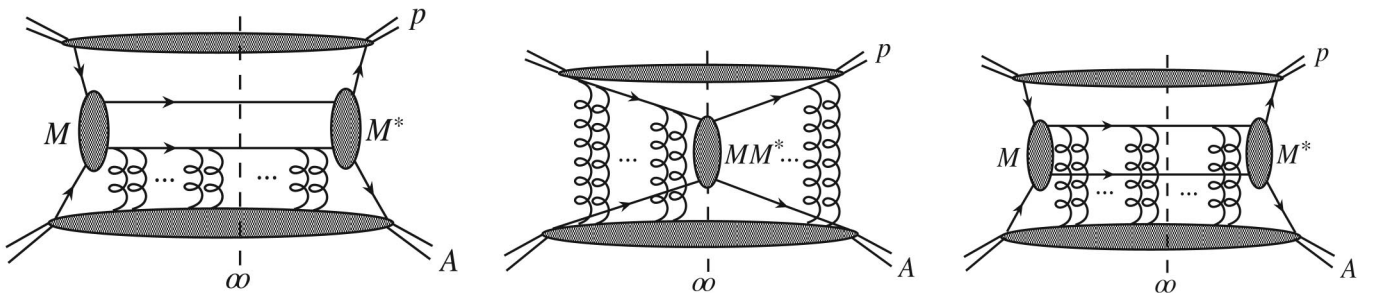
FIG. 9. Multiple coherent scattering of the incoming and outgoing partons in p + A reactions in the t -, s - and u -channels, respectively.
