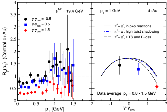
FIG. 13 (color online). Left panel: nuclear modification at three different rapidities y - y_{\text{cm}} in \sqrt{s_{NN}} = 19.4 GeV d + \text{Au} collisions. Data is from NA35 [37]. Right panel: theoretical calculations of charged pion production in p + p and d + \text{Au} collisions with high-twist shadowing (HTS) and energy loss compared to the experiment.
