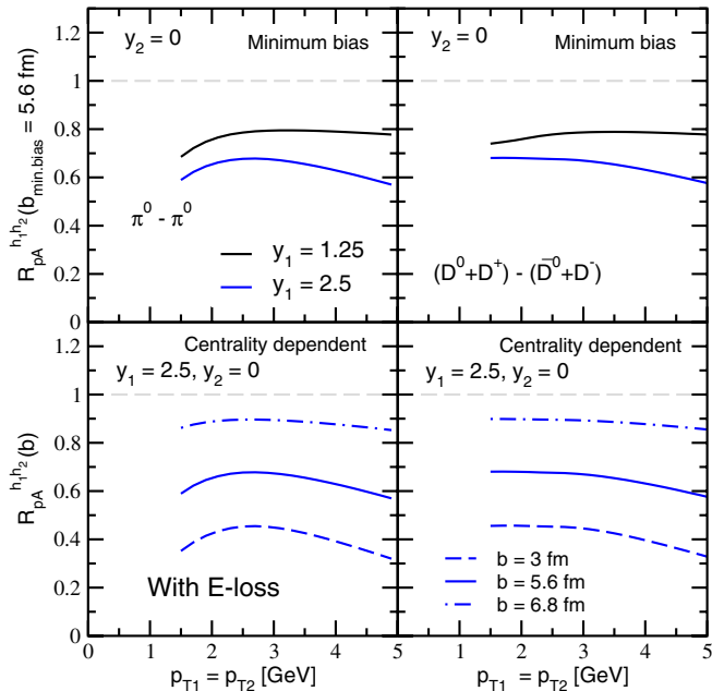
FIG. 15 (color online). Nuclear modification of \pi^0 - \pi^0 di-hadron correlations (left panels) and (D^0 + D^+) - (\bar{D}^0 + D^-) mesons correlations (right panels) in d + Au collisions at RHIC. The same rapidities and centralities as in Fig. 11 are shown. Energy loss is taken into account in the theoretical calculations.
