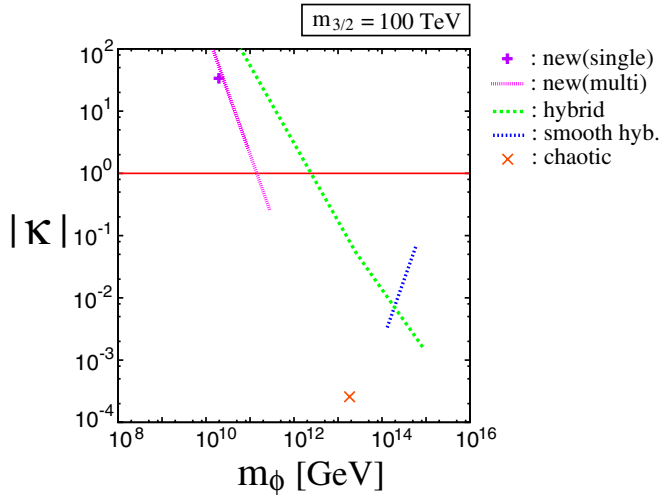
FIG. 7 (color online). Same as Fig. 6 except for m_{3/2} = 100 TeV.
