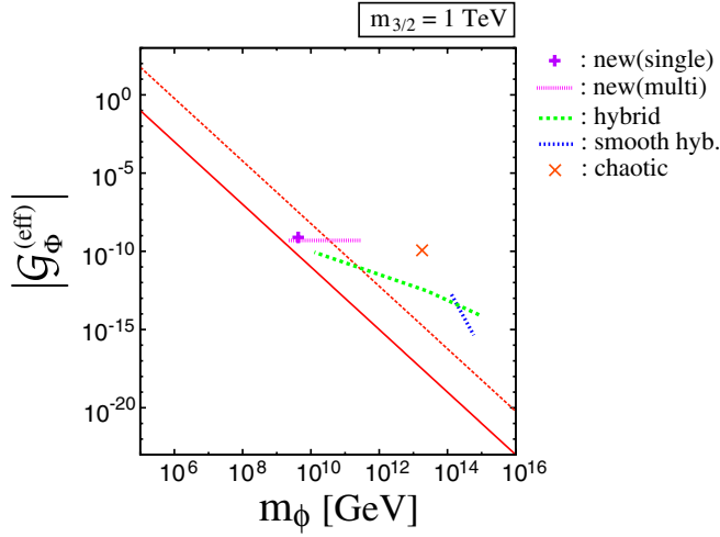
FIG. 3 (color online). Same as Fig. 2 except for m_{3/2} = 1 TeV. The typical values of \mathcal{G}_\phi^{(\text{eff})} and m_\phi for the single-field new inflation model with \kappa = 1 are also plotted. The solid and dashed lines are for the hadronic branching ratio B_h = 1 and 10^{-3} , respectively.
