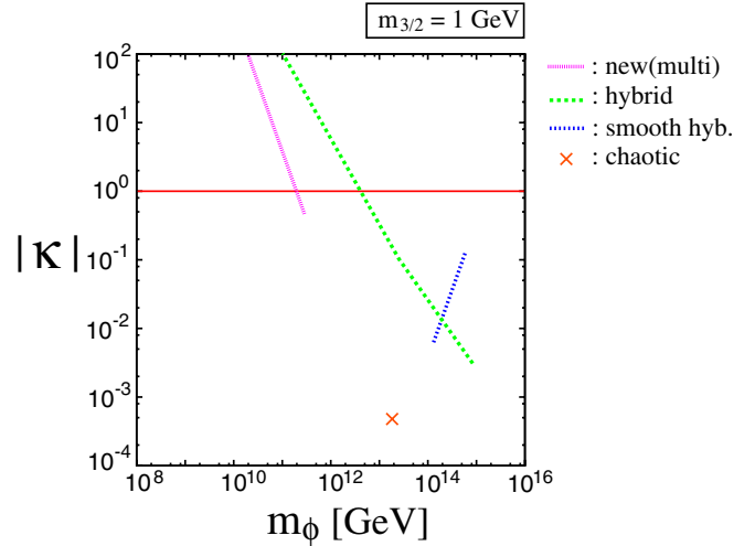
FIG. 5 (color online). Upper bounds on \kappa as a function of the inflaton mass m_\phi , with m_{3/2} = 1 GeV, for the multifield new, hybrid, and smooth hybrid, and chaotic inflation models are also shown. See the text for the definition of \kappa in each model.
