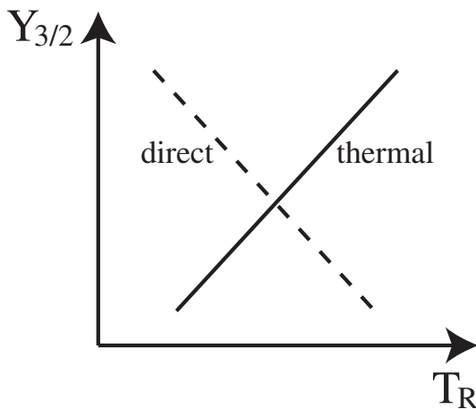
FIG. 1. Dependence of the gravitino-to-entropy ratio on the reheating temperature T_R . The solid line represents the abundance of the thermally produced gravitinos, while the dashed line corresponds to that directly produced by the inflaton decay. See (3) and (22) in the text.
