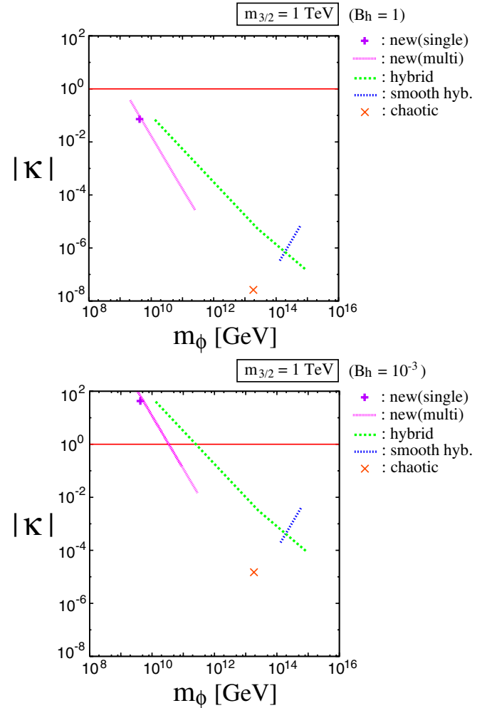
FIG. 6 (color online). Same as Fig. 5 except for m_{3/2} = 1 TeV. The bound on the single-field new inflation model is also plotted.
