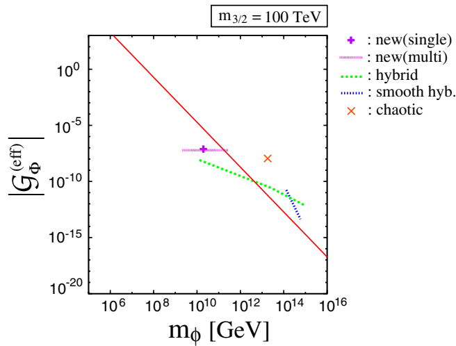
FIG. 4 (color online). Same as Fig. 3 except for m_{3/2} = 100 TeV.
