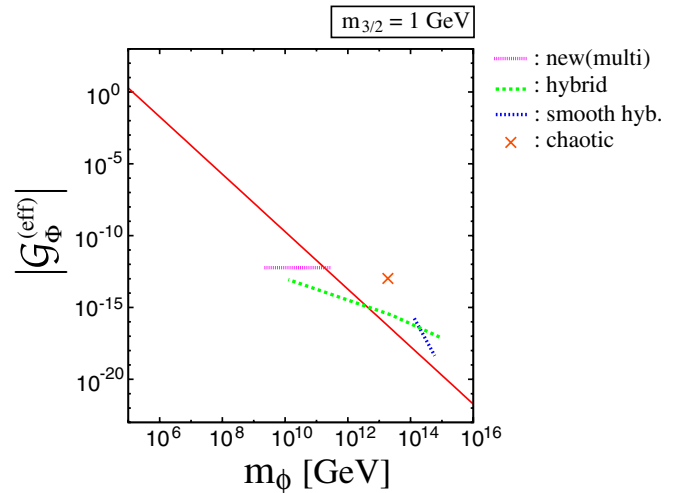
FIG. 2 (color online). Upper bound on the (effective) auxiliary field of the inflaton \mathcal{G}_\Phi^{(\text{eff})} as a function of the inflaton mass m_\phi , with m_{3/2} = 1 \text{ GeV} . We set m_{\tilde{g}_3} = 500 \text{ GeV} . T_R is set to be the largest allowed value, and the bound becomes severer for lower T_R . The typical values of \mathcal{G}_\Phi^{(\text{eff})} and m_\phi for the multifield new, hybrid, smooth hybrid, and chaotic inflation models with \kappa = 1 are also shown. The chaotic inflation can avoid this bound by assuming Z_2 symmetry (see the text for details).
