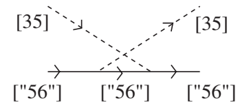
FIG. 2. Diagrammatic representation of the crossed nucleon pole term.
