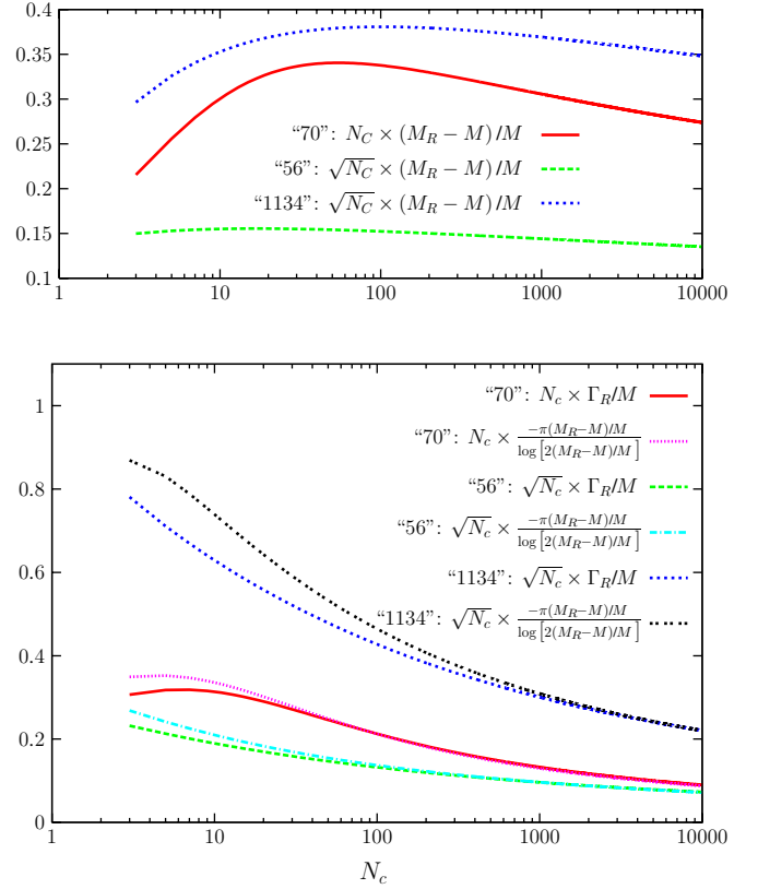
FIG. 3 (color online). SU(6) “70”, “56”, and “1134” resonance masses ( M_R ) and widths ( \Gamma_R ) obtained from \mathcal{H}_{\text{WT,SU}(6)}^{\text{SU}(N_c)} as a function of N_c .
