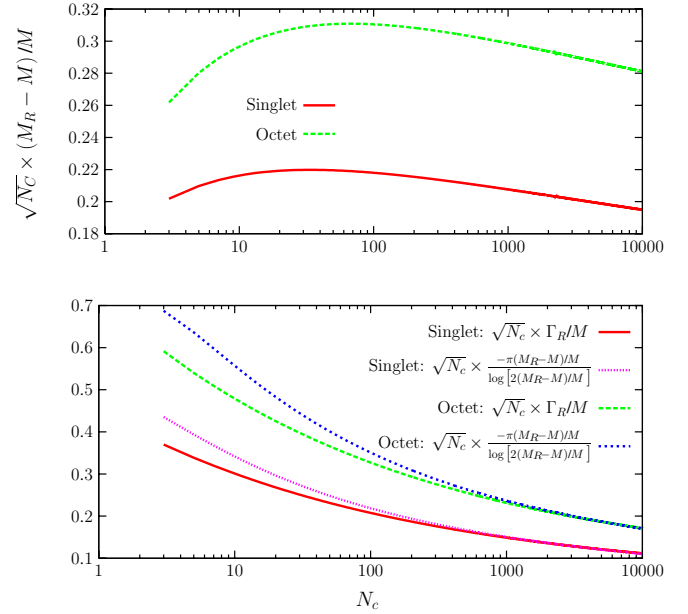
FIG. 1 (color online). Singlet and octet resonance masses ( M_R ) and widths ( \Gamma_R ) as a function of N_c from the naive large N_c limit of the \chi - \text{BS}(3) .
