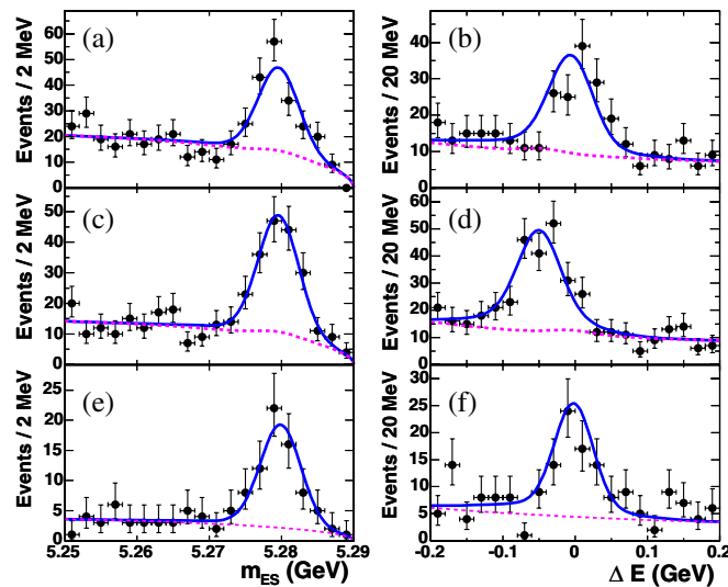
FIG. 1 (color online). The B candidate m_{\text{ES}} and \Delta E projections for B^+ \rightarrow \omega\pi^+ (a, b), B^+ \rightarrow \omega K^+ (c, d), and B^0 \rightarrow \omega K^0 (e, f) shown for a signal-enhanced subset of the data. Points with error bars represent the data, the solid line the fit function, and the dashed line the background components. Note that the \omega K^+ signal in the \Delta E plot is displaced from zero since \Delta E is defined for the \omega\pi^+ hypothesis.
