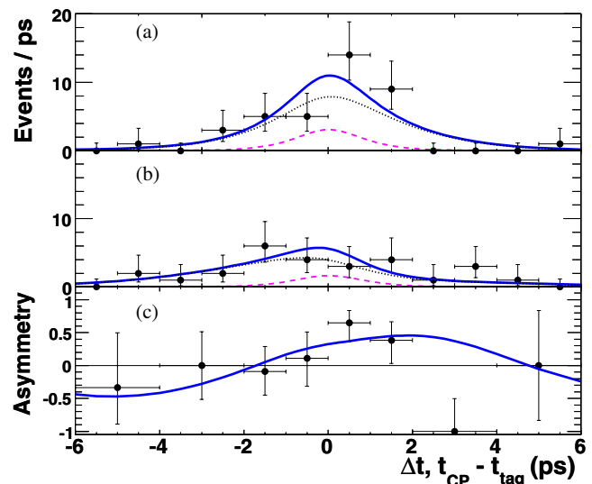
FIG. 2 (color online). Projections onto \Delta t for B^0 \rightarrow \omega K^0 . Data (points with errors), the fit function (solid line), background component (dashed line), and signal component (dotted line), for events in which the tag meson is (a) B^0 and (b) \bar{B}^0 , and (c) the asymmetry (N_{B^0} - N_{\bar{B}^0}) / (N_{B^0} + N_{\bar{B}^0}) .
