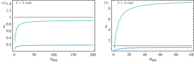
FIG. 5 (color online). The dimensionless four-fermion coupling: g_4^{(6)} on the 3-brane summing up until N_{\text{KK}} ; the horizontal dashed line is g_4^{\text{crit}} = 1 on the 3-brane. Fig. (a) is for D = 6 ( \delta = 2 ), and (b) for D = 8 ( \delta = 4 ). The upper lines are T^\delta -compactification cases with k = 0 and the lower lines are T^\delta/Z_2^k -compactification cases with k = 1 (for \delta = 2 ) and k = 2 (for \delta = 4 ).
