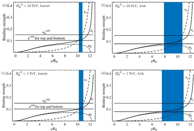
FIG. 4 (color online). Binding strengths for tau, bottom and top. In (a) and (b) shown are the binding strengths \kappa_\tau , \kappa_t and \kappa_b for tau, top and bottom, respectively, on the 5-brane with R_6^{-1} = 10 TeV, while in (c) and (d) shown are those with R_6^{-1} = 1 TeV. The upper horizontal line in the figures is the critical binding strength for tau, \kappa_6^{\text{crit}} = 0.15 (nonlocal gauge fixing method). The lower line is the one for top and bottom, \kappa^{\text{crit}} derived by using the upper bound of c (the coefficient of the dimensionless four-fermion coupling): (a), (c) are those by the lowest KK mode only, while (b), (d) are those by the summation till the 4th KK modes. The shaded regions which are equivalent to the corresponding shaded regions in Fig. 3 are the tMAC scales: \Lambda_{\text{tM}}R_6 = (a)10.2–10.8, (b) 7.8–10.8, (c) 10.3–11, (d) 7.5–11.
