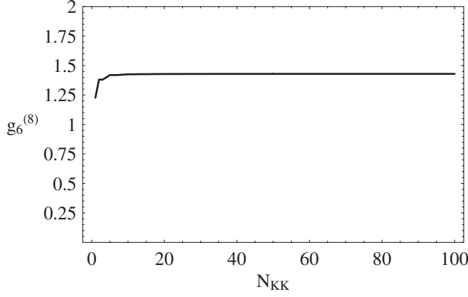
FIG. 6. The estimation of g_6^{(8)} for Eq. (59) for the summation by N_{\text{KK}} (KK-mode mass 2 is N_{\text{KK}}^2 M_1^2 ).
