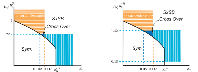
FIG. 3 (color online). The phase diagram and the tMAC region by the nonlocal gauge fixing method; These figures are for R_6^{-1} = 10 \text{ TeV} case. (a) is estimated by the lowest KK mode only, and (b) is by the summation till the 4th KK modes. The vertical dashed lines are the value of \kappa_t at scale \Lambda_\tau . The vertical stripe pattern regions are the allowed regions from Eqs. (66) and (67). In order to make top quark condense, these vertical stripe regions and the horizontal stripe (no tau condensation) regions must have cross over regions. In this figure, there exists cross over regions (shaded regions).
