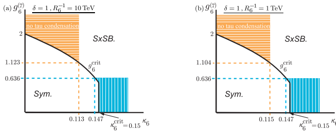
FIG. 2 (color online). The phase diagram of D(=6) -dimensional gauged NJL model [25] with the induced four-fermion coupling by the 7-dimensional bulk gluons (one compactified dimension \delta = 1 ). The critical line in Eq. (70) is denoted by g_6^{\text{crit}} with the nonlocal gauge estimation. The region above g_6^{\text{crit}} is the S\chi SB -phase, and that below is the Symmetric -phase. The vertical stripe pattern regions are from Eq. (81): g_6^{\text{crit}}(\kappa_t) < g_6^{\text{induced}} < 0.636 or equivalently \kappa_t > \kappa_t^{\text{crit}} > \kappa_6^{\text{crit}}(0.636) = 0.147 . The horizontal stripe pattern regions are those satisfying Eq. (77), namely, the region for the top condensate without tau condensation: (a) is for R_6^{-1} = 10 TeV with (\kappa_t(\Lambda_\tau), g_6^{\text{crit}}(\kappa_t(\Lambda_\tau))) = (0.113, 1.123) and (b) is for R_6^{-1} = 1 TeV with (\kappa_t(\Lambda_\tau), g_6^{\text{crit}}(\kappa_t(\Lambda_\tau))) = (0.115, 1.104) . The tMAC scale satisfying Eq. (78) would be the overlap region between regions of the vertical and the horizontal stripe pattern, which does not exist in either case (a) or (b).
