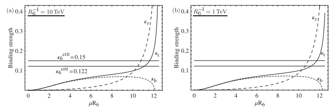
FIG. 1. Binding strengths \kappa_\alpha ( \alpha = t, b, \tau ) for the top, bottom and \tau on the 5-brane: A compactification scale is (a) R_6^{-1} = 10 \text{ TeV} and (b) R_6^{-1} = 1 \text{ TeV} . Note that the upper horizontal line is \kappa_6^{\text{crit}} by using the nonlocal gauge fixing method ( \kappa_6^{\text{crit}} = 0.15 ) and the lower one is \kappa_6^{\text{crit}} by using the Landau gauge fixing method ( \kappa_6^{\text{crit}} = 0.122 ) [21,24].
