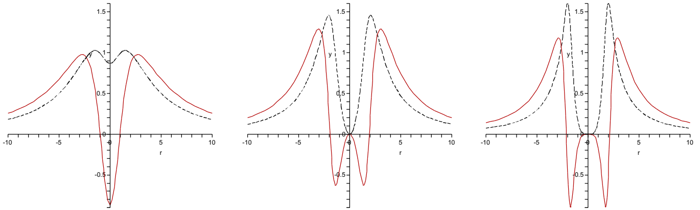
FIG. 1 (color online). V_{\text{QM}}^- (continuous line) and V_{\text{QM}}^+ (dashed line) for the double walls with s = 1 , s = 3 and s = 5 .
