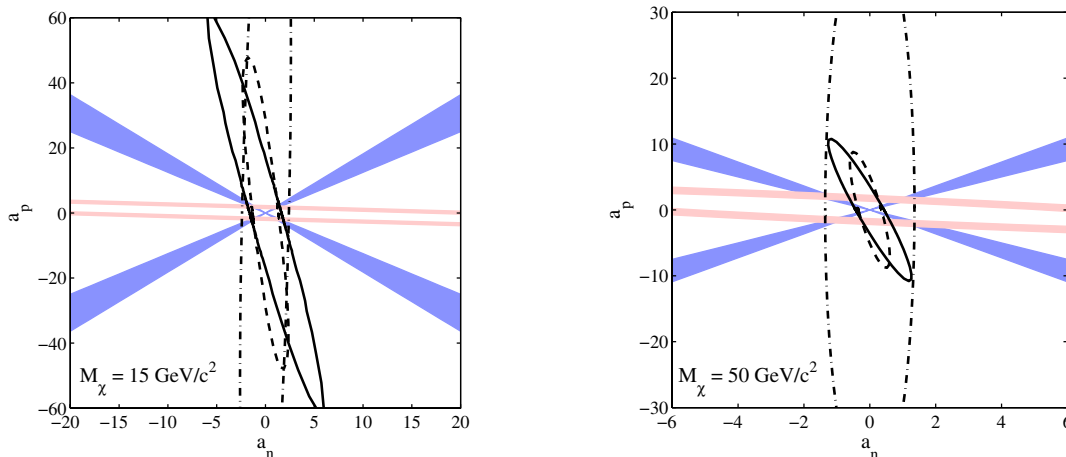
FIG. 2 (color online). Regions in the a_p - a_n plane allowed (at the 90% confidence level) by CDMS data. Each data set excludes the exterior of the corresponding ellipse. Two choices of WIMP mass M_\chi are shown: 15 \text{ GeV}/c^2 (left) and 50 \text{ GeV}/c^2 (right). Dot-dashed ellipses represent Si limits, solid ellipses represent Ge limits, and dashed ellipses represent Ge limits using the alternate form factor. Also shown are the corresponding interpretations of the DAMA/NaI modulation signal (near-horizontal light (pink) filled bands are 3\sigma -allowed). The thin dark (blue) filled wedges correspond to models satisfying 0.55 < |\frac{a_n}{a_p}| < 0.8 , a constraint from the effMSSM framework [16].
