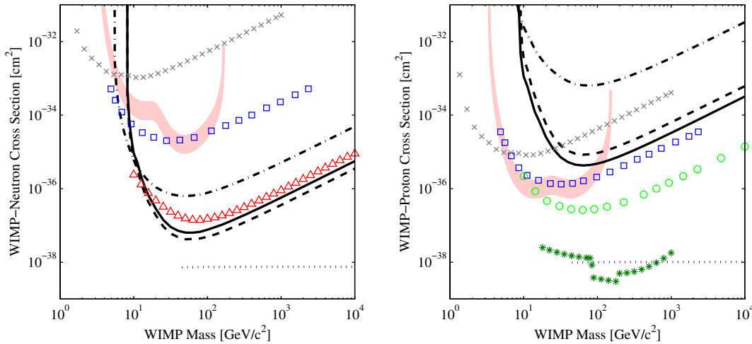
FIG. 1 (color online). Upper limit contours (90% confidence level) for recent CDMS data sets, plotted in the cases of (left) pure neutron and (right) pure proton coupling. We show limits based on Ge (solid line) and Si (dash-dot line) from the combined Soudan data (black). Dashed curves represent Ge limits using the alternate form factor from [18]. As benchmarks, we also include interpretations of the DAMA/NaI annual modulation signal [10] (filled regions are 3\sigma -allowed) and limits from other leading experiments: CRESST I [23] as computed in [11] (“×”s), PICASSO [26] (squares), NAIAD [27] (circles), ZEPLIN I [28] (triangles), and Super-Kamiokande [29] (asterisks; an indirect search, based on different assumptions). EDELWEISS [30] and SIMPLE [31] report limits (not shown for clarity) comparable to CDMS Si and PICASSO, respectively. As a theoretical benchmark (see text), horizontal dotted lines indicate expected cross sections for a heavy Majorana neutrino. Plots courtesy of [32].
