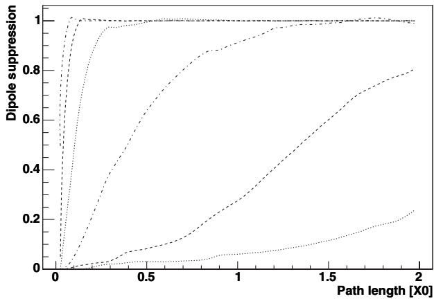
FIG. 3. Average Cherenkov photon emission rate for pairs with energies from 10^{10} (leftmost, dot-dashed curve) to 10^{15} eV (rightmost, dotted curve) vs the distance traveled by the pair in water, relative to emission from two independent particles.
