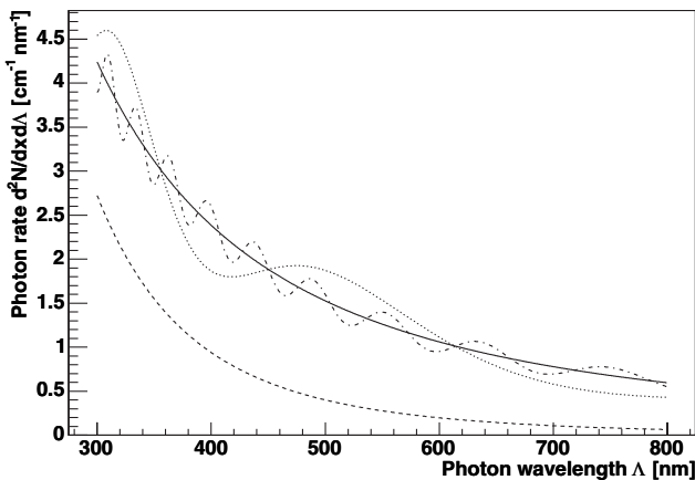
FIG. 2. The spectrum of Cherenkov radiation at \beta = 1 , \sqrt{\epsilon(\omega)} = n = 1.3 . Solid line is for e^+e^- with the particles considered independently, and the dashed lines are for pairs treated coherently, with separations 100 nm, 1 \mu\text{m} and 5 \mu\text{m} .
