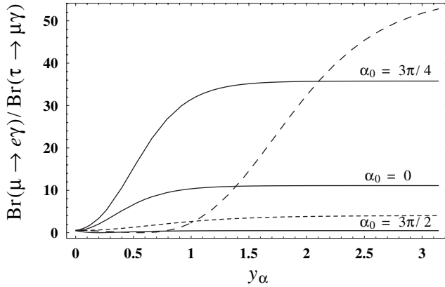
FIG. 2. The ratio of the branching ratios is shown in the IH case for Q_1 with \alpha_0 = 0, 3\pi/4, 3\pi/2 (solid curves), for Q_2 (dotted curve), and for Q_3 (dashed curve).
