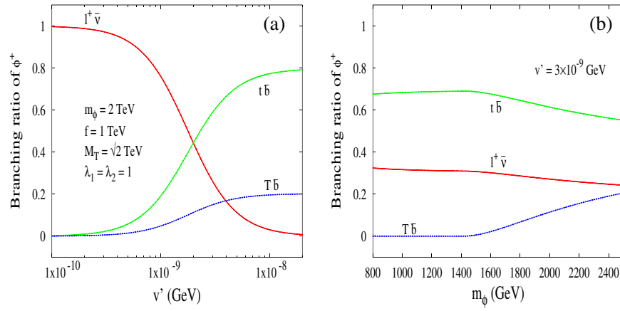
FIG. 3 (color online). Branching ratio of \phi^+ (a) versus the triplet vev for Yv' = 10^{-10} \text{ GeV} and m_\phi = 2 \text{ TeV} and (b) versus m_\phi for v' = 3 \times 10^{-9} \text{ GeV} .
