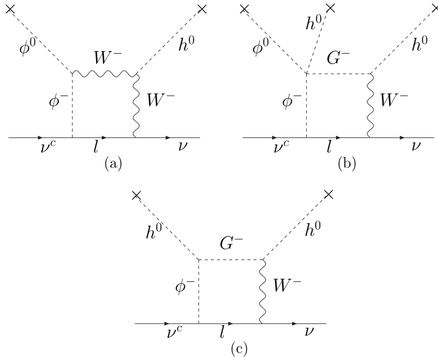
FIG. 1. Representative one-loop diagrams giving rise to neutrino masses via dimension-five operators.
