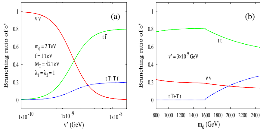
FIG. 4 (color online). Branching ratios of \phi^s (a) versus the triplet vev for Yv' = 10^{-10} \text{ GeV} and m_\phi = 2 \text{ TeV} and (b) versus m_\phi for v' = 3 \times 10^{-9} \text{ GeV} . The branching ratios of \phi^p are virtually identical for the parameter ranges shown.
