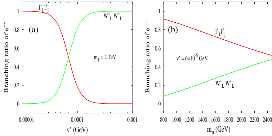
FIG. 2 (color online). Branching ratios of \phi^{++} (a) versus the triplet vev for Yv' = 10^{-10} GeV and m_\phi = 2 TeV and (b) versus m_\phi for v' = 6 \times 10^{-5} GeV.
