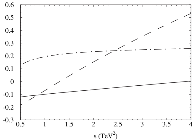
FIG. 2. The total electroweak logarithmic two-loop corrections to \mathcal{R}_{IQ} (dashed line), \mathcal{R}_{lq} (dot-dashed line) and \mathcal{R}_W (solid line) in percent.
