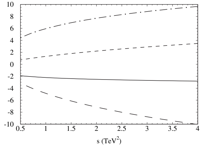
FIG. 1. The LL (short-dashed line), NLL (long-dashed line), NNLL (dot-dashed line) and N^3 LL (solid line) two-loop electroweak corrections to \mathcal{R}_{lq} in percent.
